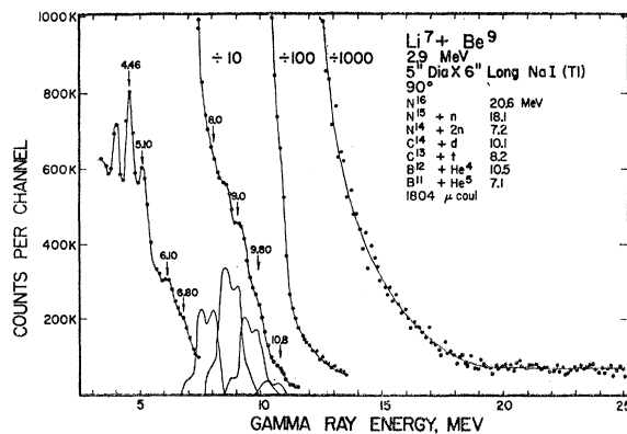
FIG. 3. \text{Li}^7 + \text{Be}^9 , 2.9-MeV bombarding energy, 1804 \mu\text{C} of triply charged ion beam current.
