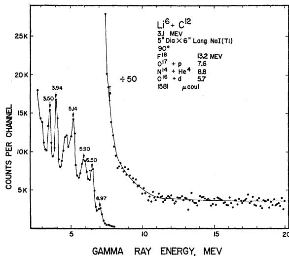
FIG. 8. Li 6 +C 12 , 3.1-MeV bombarding energy, 1581 μC of triply charged ion beam current.
