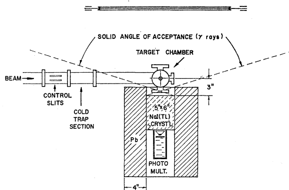
FIG. 1. Diagram of experimental geometry. Crystal was recessed in lead block so that no gamma rays produced in control slits or cold trap section could reach crystal except by scattering.
