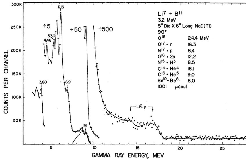
FIG. 7. Li 7 +B 11 , 3.2-MeV bombarding energy, 1001 μC of triply charged ion beam current.
