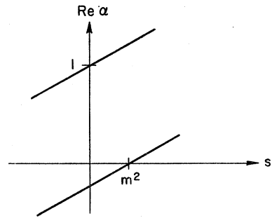
FIG. 6. Pommeranchuk and meson trajectories.
