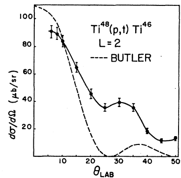
FIG. 4. Angular distribution of tritons from Ti^{48}(p,t)Ti^{46} , 0.887-MeV state. The dashed line represents a plane-wave Butler fit obtained with a radius r=5.0 F. Using the same radius as for the L=0 ground state fit, the second maximum occurs at 19^\circ .
