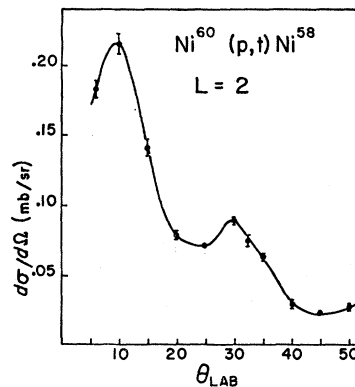
FIG. 24. Angular distribution of tritons from \text{Ni}^{60}(p, t)\text{Ni}^{58} , 1.452-MeV state.
