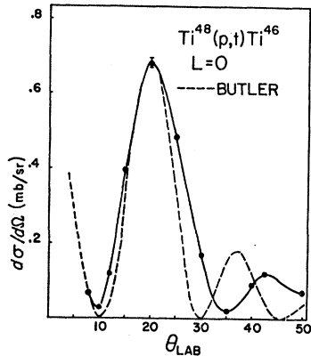
FIG. 3. Angular distribution of tritons from Ti^{48}(p,t)Ti^{46} , ground state. The dashed line represents a plane wave Butler fit obtained with a radius r=8.63 F.
