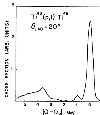
FIG. 2. Energy spectrum of tritons from Ti^{48}(p,t)Ti^{46} .
