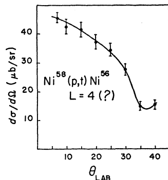
FIG. 21. Angular distribution of the 3.87-MeV triton group from \text{Ni}^{58}(p, t)\text{Ni}^{56} .
