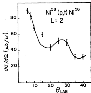
FIG. 20. Angular distribution of the 2.85-MeV triton group from \text{Ni}^{58}(p, t)\text{Ni}^{56} .
