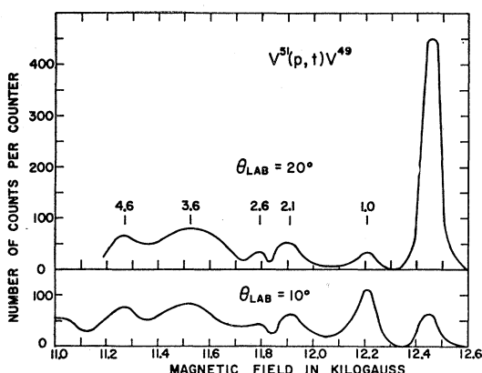
FIG. 5. Energy spectra of tritons from V^{51}(p,t)V^{49} .
