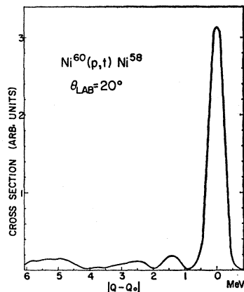
FIG. 22. Energy spectrum of tritons from \text{Ni}^{60}(p, t)\text{Ni}^{58} .
