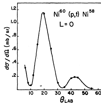
FIG. 23. Angular distribution of tritons from \text{Ni}^{60}(p, t)\text{Ni}^{58} , ground state.
