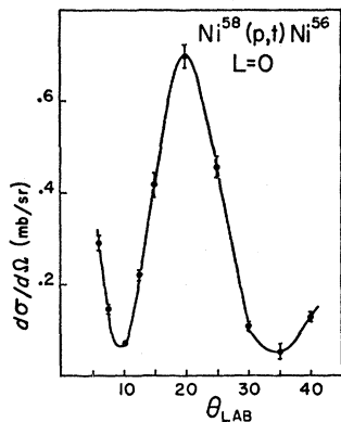
FIG. 19. Angular distribution of tritons from \text{Ni}^{58}(p, t)\text{Ni}^{56} , ground state.
