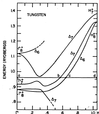
FIG. 1. Relativistic energy bands for tungsten (Ref. 6).
