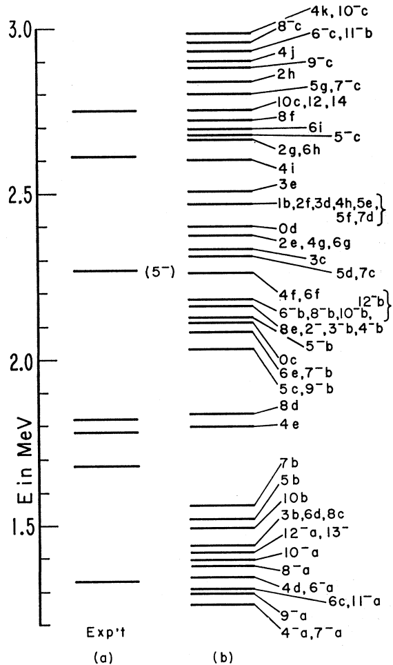
FIG. 3. Continuation of the level schemes of Fig. 2 (a) and (b) up to energy E=3.0 MeV (energy of excitation 4.25 MeV). Part (a) shows the observed levels, Part (b), those calculated for the Gaussian SE interaction. Experimental results indicate that the (5^-) state with E=2.27 MeV (excitation 3.52 MeV) is core-excited. (The level 11^-b should be at 1.94 MeV instead of 2.94 MeV.)
