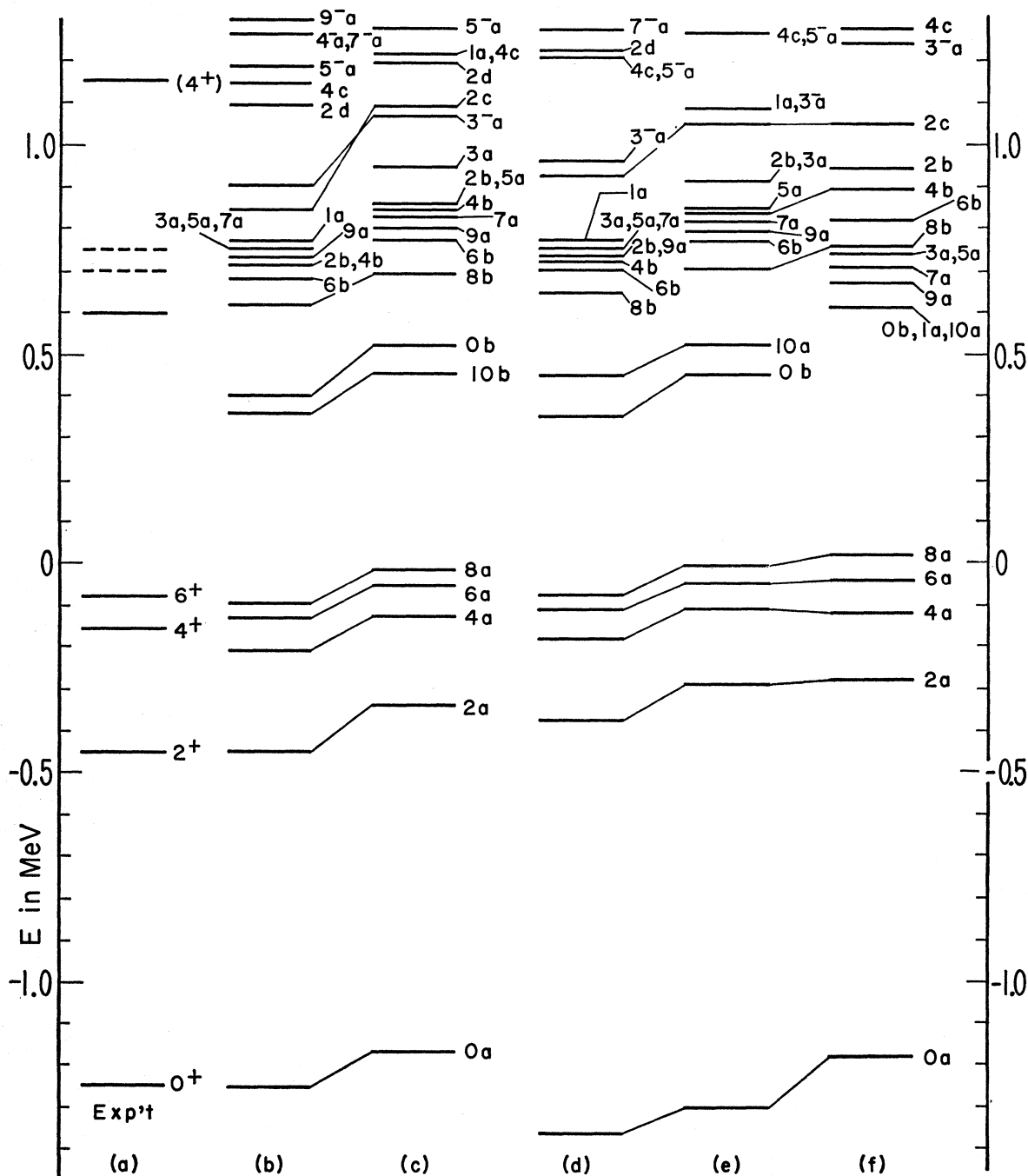
FIG. 2. (a) Observed levels of Pb^{210} . The ordinate is the energy of interaction between the two outer nucleons. The energy of the nucleons in the ground state is taken from data as -1.250 MeV. The remaining schemes show calculated levels: (b) Gaussian SE interaction. (c) Gaussian SE+repulsive TO interaction, from Eqs. (3) and (5) with \alpha = -0.5 . (d) Yukawa SE interaction. (e) Yukawa SE+repulsive TO interaction from Eqs. (4) and (5) with \alpha = -0.559 . (f) Yukawa SE+Feshbach-Schwinger central+tensor TO interaction, from Eq. (7). The radius parameter \nu equals 0.20539 F^{-2} for both (b) and (c), and 0.18457 F^{-2} for (d), (e), and (f). Theoretical levels with parity + are labeled Jx ; those with parity - are labeled J-x . Here, x indicates the order, with x = a for the lowest state.
