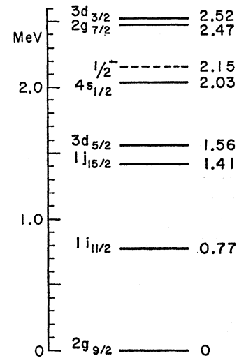
FIG. 1. The energies \Delta(j) of the states below 3 MeV which have been identified in the reaction Pb^{208}(d,p)Pb^{209} (Ref. 12). Each level except the 1/2^- level, represented by a dashed line, has a single-particle assignment.
