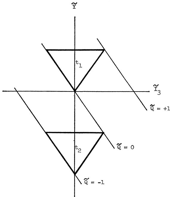
FIG. 2. The two-triplet model.
