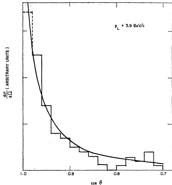
FIG. 3. Fit of calculation using (5) with \rho^N \eta_{1/2} = 0 and \Lambda^2 = \infty to the data of Ref. 2. The first bin is dotted to note that the experimental value is uncertain and is an estimate of the correct value by Z. Guiragossian.
