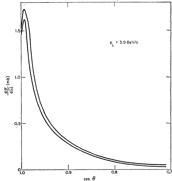
FIG. 5. Upper curve uses Eq. (5) for the absorptive corrections with \rho^N \eta_{1/2} = 0 and \Lambda^2 = 50m_\pi^2 whereas the lower one uses (6) with \rho^N \eta_{1/2} = 0 and \Lambda^2 = 30m_\pi^2 .
