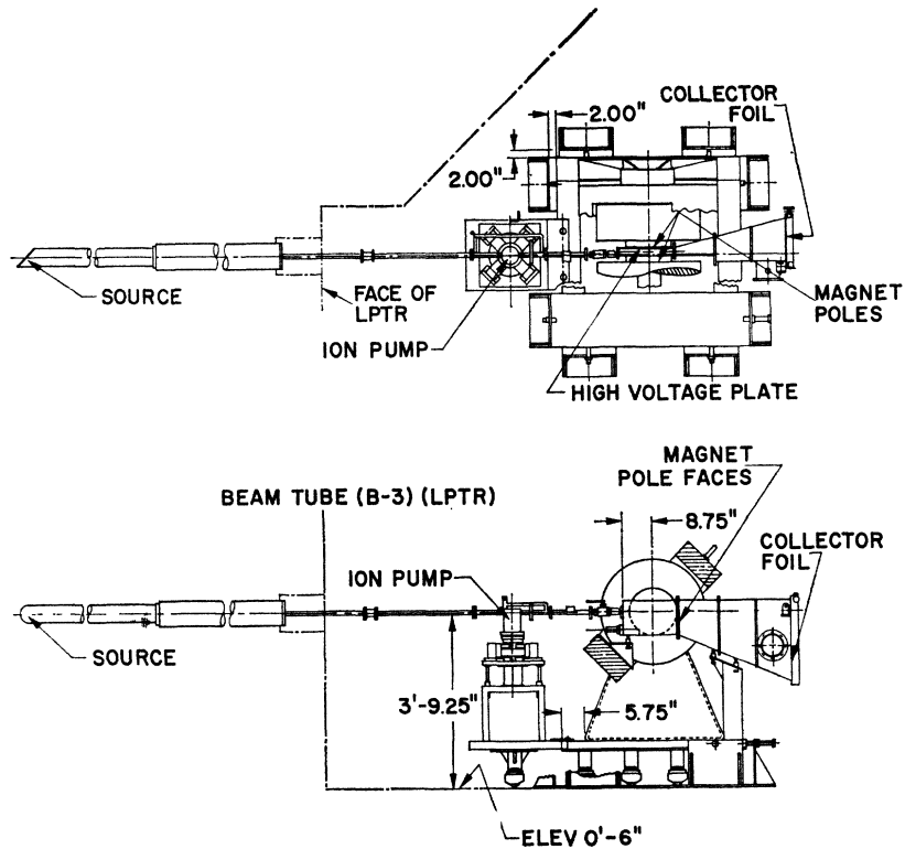
FIG. 3. Fission-fragment analyzer used to obtain the data in this report.
