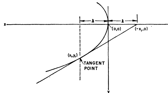
FIG. 5. A line from the point (-x_1,0) to the parabola at the point (x_1,y_1) is tangent to the parabola at that point. This line therefore represents an approximation to the parabola in the neighborhood of (x_1,y_1) .
