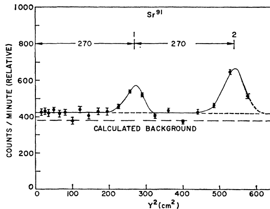
FIG. 9. Low-charged fragments of mass 91 as measured by Sr^{91} .
