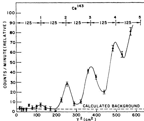
FIG. 15. Low-charged fragments of mass 143 as measured by Ce 143 .
