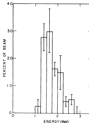
FIG. 16. Energy spectrum of singly charged mass-99 fission fragments emerging from a thick uranium source.
