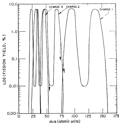
FIG. 1. Yield (atoms per hundred fissions) of fission products of various masses plotted against mass-to-charge ratio of fragments for various assumed values of the ionic charge. It can be seen that only the curve for charge 1 (extreme right-hand curve in the figure) is essentially free of overlap with curves for other charges. Curves for charges higher than 4 are omitted for clarity. All such curves would lie between existing curves and the vertical axis, with a great deal of overlap on the charge 3 and 4 curves.
