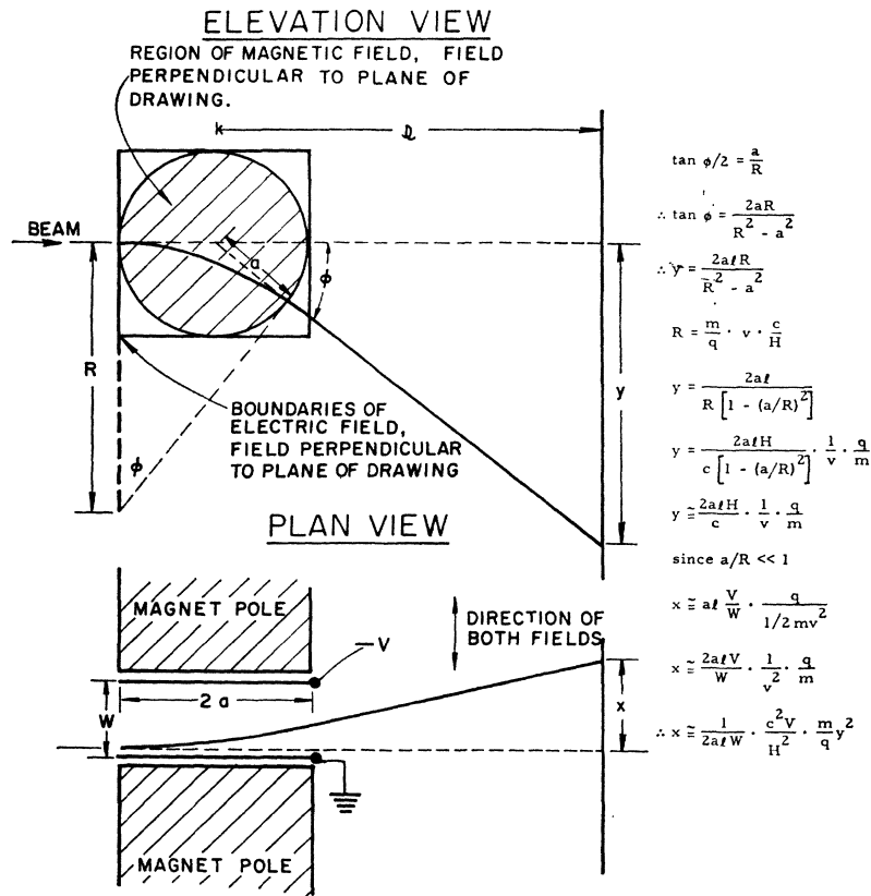
FIG. 2. Schematic views of the essential parts of the Thomson parallel field mass analyzer.
