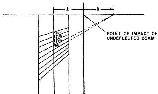
FIG. 6. Method of cutting collector foil for radiochemical analysis. The trapezoidal sections are rough approximations to parabolic arcs passing through the origin and through the centers of the trapezoids.
