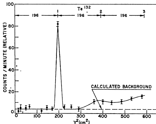
FIG. 13. Low-charged fragments of mass 132 as measured by Te^{132} .
