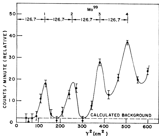
FIG. 11. Low-charged fragments of mass 99 as measured by Mo^{99} .
