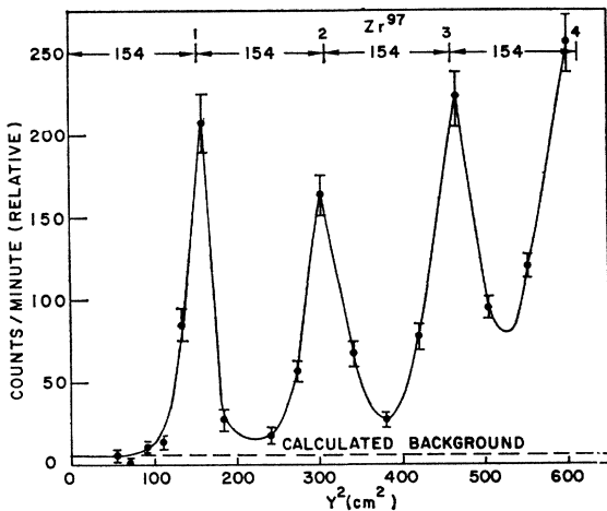
FIG. 10. Low-charged fragments of mass 97 as measured by Zr^{97} .
