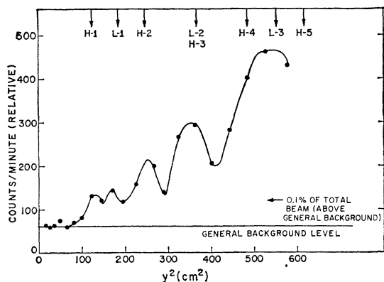
FIG. 7. Gross activity of cut sections of collector foil, showing predicted positions of light and heavy fission fragments. The general background level is presumed to come from deposition of fission products thermally evaporated from the source. This background level persists over the entire collector foil.
