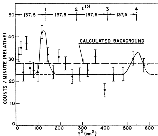
FIG. 12. Low-charged fragments of mass 131 as measured by I^{131} .
