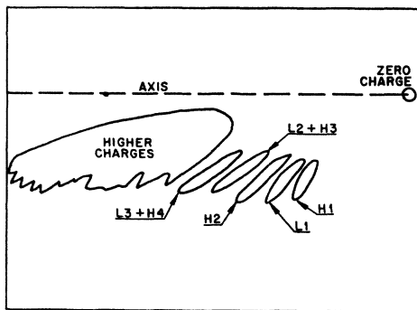
FIG. 4. Outline of autoradiograph of collector foil from fission-fragment analyzer. Circular area at right represents the undeflected beam. Dotted line indicates position of one of the coordinate axes. Magnetic deflection is horizontal (leftward), electric deflection is vertical (downward). In the original autoradiograph faint smudges representing lower charged fission fragments could be seen to the right of the large irregular area. The ellipsoidal areas labeled H1, L1, and so on are the resolved low-charge beams. H indicates "heavy fragment"; L indicates "light fragment." The numeral next to each letter indicates the assumed fragment ionic charge.
