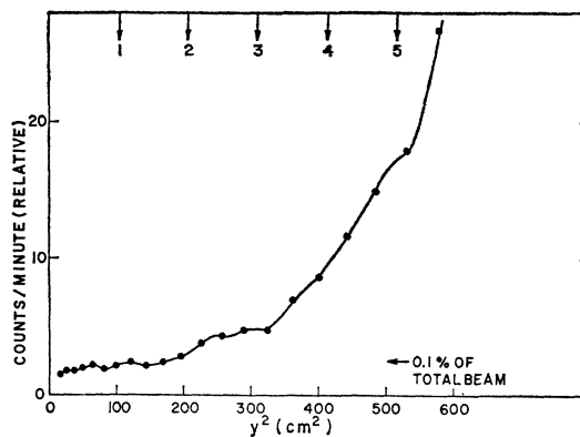
FIG. 8. Low-charged fragments of mass 140 as measured by Ba^{140} have been obscured by decay products from thermally evaporated Xe^{140} .
