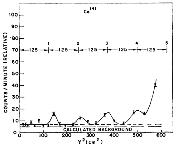
FIG. 14. Low-charged fragments of mass 141 as measured by Ce 141 .
