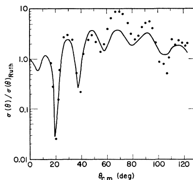
FIG. 22. A plot of \sigma/\sigma_{\text{Ruth}} for 38.1-MeV alpha particles scattered from C^{12} (Ref. 23). The solid line is the predicted value of \sigma/\sigma_{\text{Ruth}} obtained using the optical-model parameters listed in Table VII.
