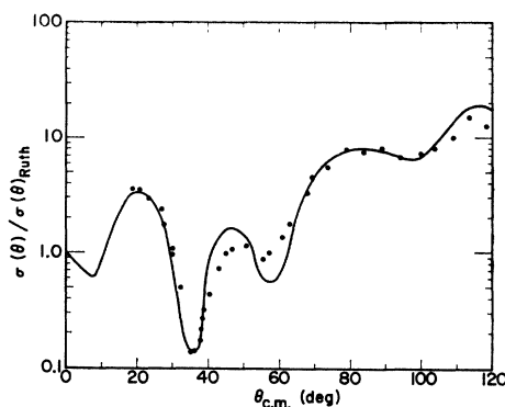
FIG. 21. A plot of the ratio \sigma/\sigma_{\text{Ruth}} of actual to Rutherford cross section for 20.9-MeV deuterons scattered from N^{14} (Ref. 22). The solid line is the predicted value of \sigma/\sigma_{\text{Ruth}} obtained using the optical-model parameters listed in Table VII.
