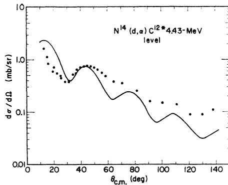
FIG. 23. Angular distribution of alpha particles from the N^{14}(d,\alpha)C^{12*} (4.43-MeV) transition. The solid line was calculated for L=2 , interaction radius=5.25 F, and the following optical-model parameters:
