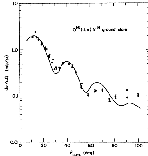
FIG. 25. Angular distribution of alpha particles from the O^{16}(d,\alpha)N^{14} ground-state transition. The solid line was calculated for L=2 , interaction radius=6.00 F, and the following optical-model parameters:
