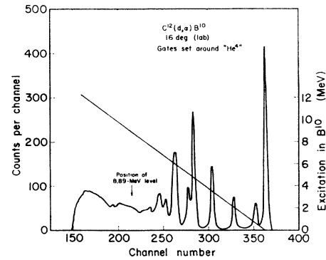
FIG. 5. Alpha-particle energy spectrum from the C 12 (d, α)B 10 reaction.
