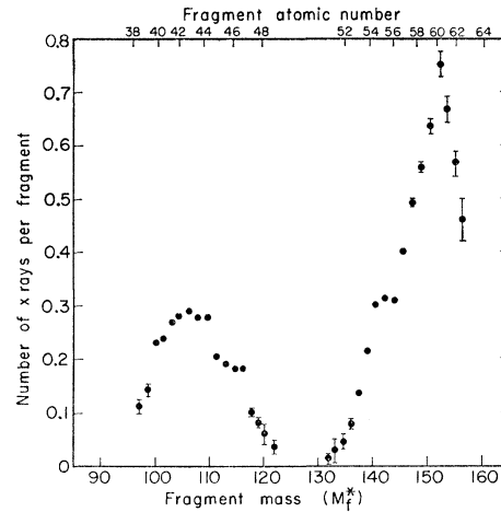
Fig. 7. The observed yield of the prompt K x rays per fragment emitted in times from 0–50 nsec, versus the final masses ( M_f^* ) and atomic numbers of the fragments (corrected for mass dispersion).
