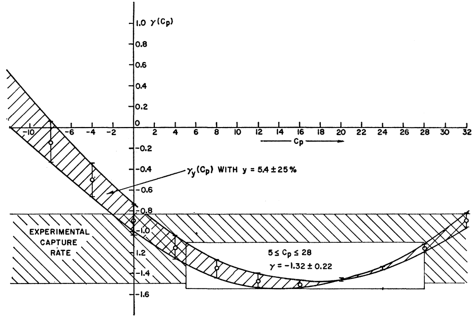
FIG. 3. The quantity \gamma_\nu(C_p) defined in Eq. (44) is plotted against C_p = m_\mu F_p / F_A^\mu . y is discussed in Eqs. (36)–(42) and the estimated uncertainty in y is indicated in the figure. The value of \gamma(C_p) as determined from Eq. (44) and the experimental value of the partial muon capture rate given in Eq. (3) [using the “canonical values” of the other coupling constants (Ref. 14)] is also shown.
