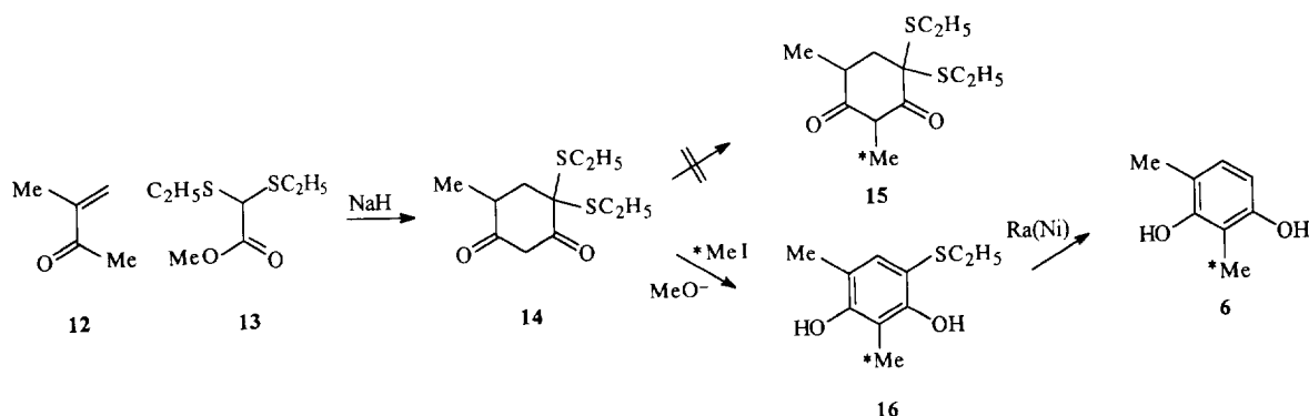
Fig. 3. Synthesis of [2-Me- 13 C]-6.
