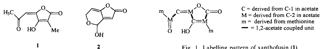
Fig. 1. Labelling pattern of xanthofusin (1).
