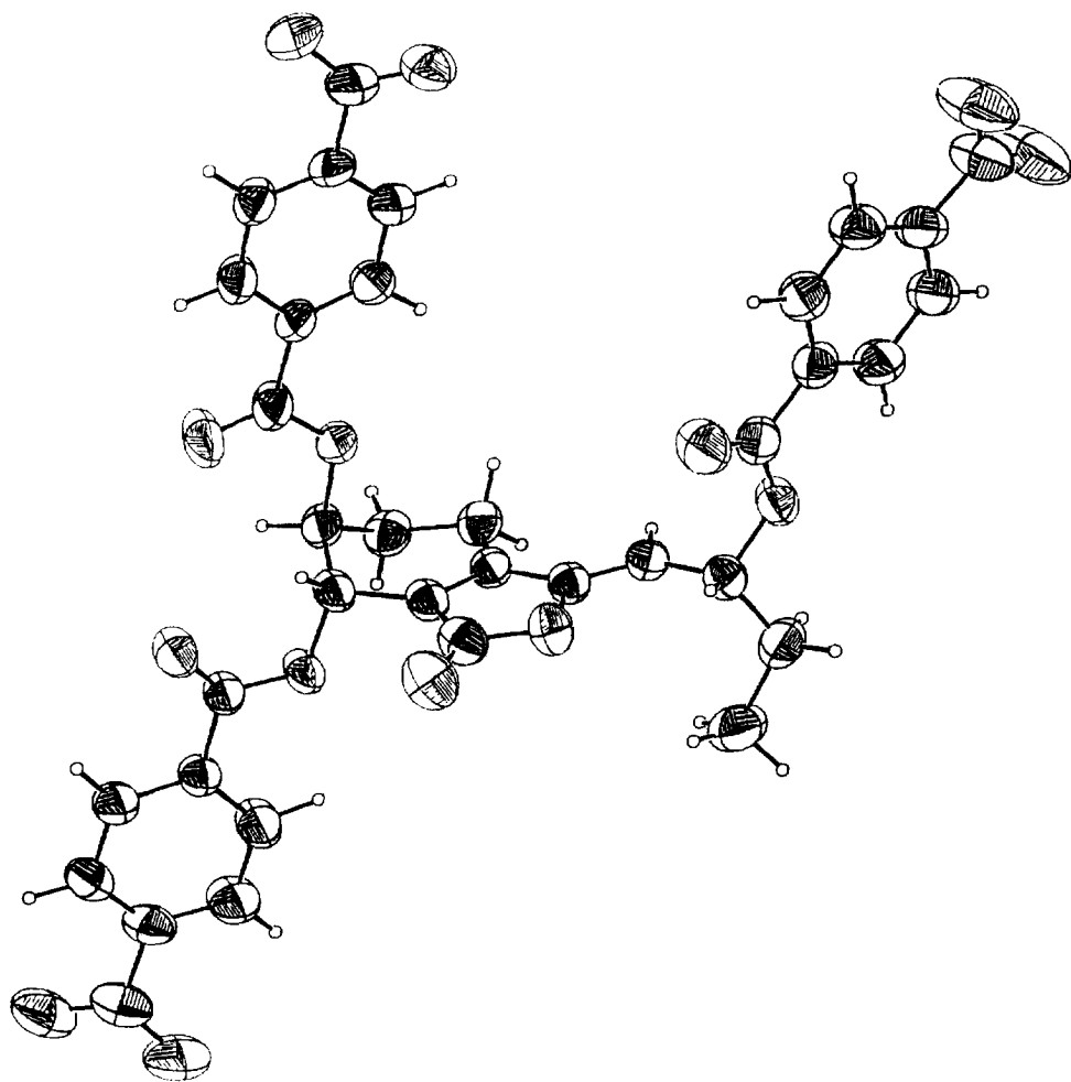
Fig. 1. ORTEP drawing of 1a.
