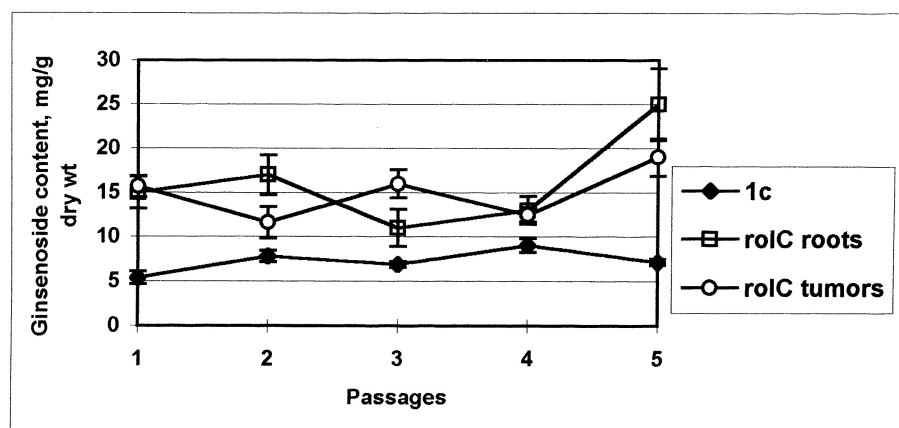
Fig. 1. Ginsenoside production in Panax ginseng 1c culture, 1c- rolC -II root culture and 1c- rolC -II secondary tumour culture grown in W 4 CPA liquid medium for 4 weeks at 25°. Values are means ± s.e. for three independent determinations.
