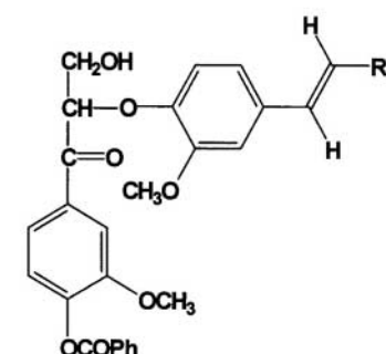
6a R = CH 3 b R = CHO
