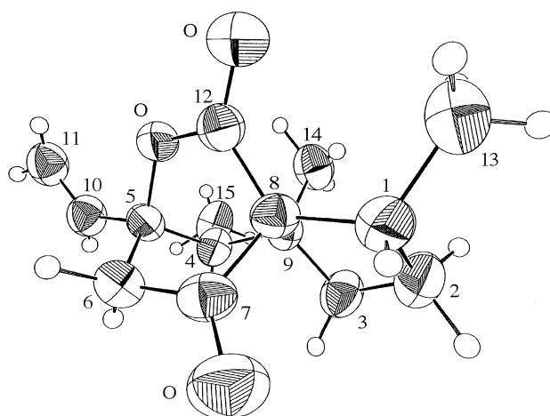
Fig. 2. ORTEP drawing of acutifolone B ( 7 ).
