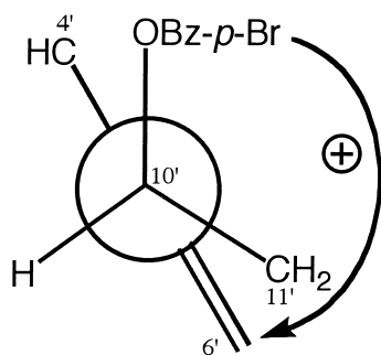
Fig. 4. A positive Cotton effect for allyl benzoate ( 15 ).
