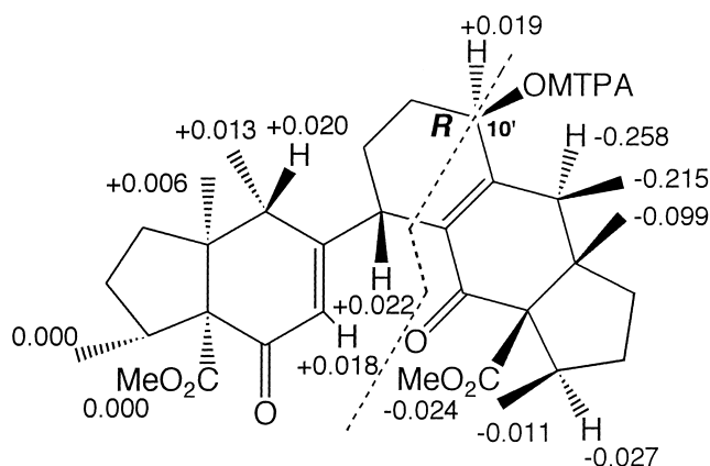
Fig. 5. \Delta\delta values [ \delta(-) - \delta(+) ] for (+)-MTPA ester ( 16 ) and (-) MTPA ester ( 17 ) of bisacutifolone A ( 13 ).
