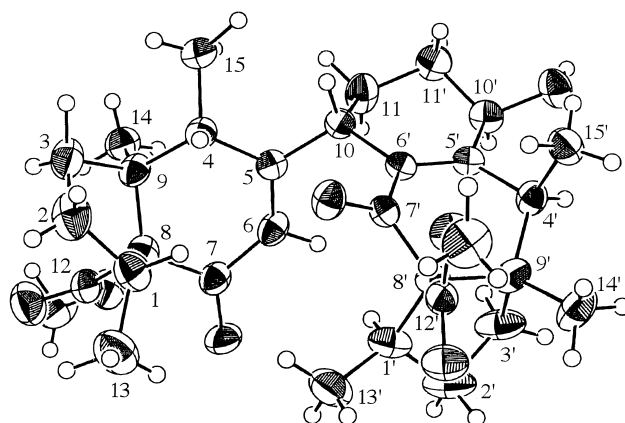
Fig. 3. ORTEP drawing of bisacutifolone A ( 13 ).
