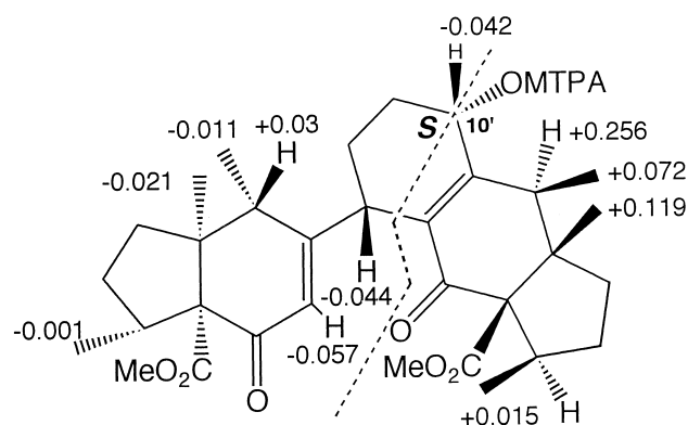
Fig. 6. \Delta\delta values [ \delta(-) - \delta(+) ] for (+)-MTPA ester ( 20 ) and (-) MTPA ester ( 21 ) of bisacutifolone B ( 18 ).
