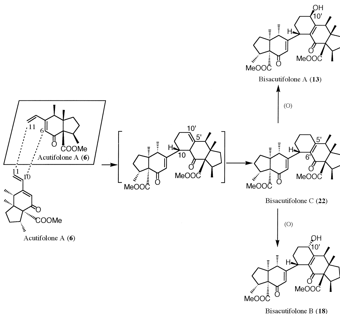
Fig. 8. Possible biogenetic pathway of bisacutifolone A–C ( 13 , 18 and 22 ).
