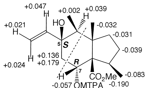
Fig. 1. \Delta\delta values [ \delta(-) - \delta(+) ] for (+)-MTPA ester ( 11 ) and (–)-MTPA ester ( 12 ) of 7 \alpha -hydroxy-pinguisenol-12-methyl ester ( 9 ).
