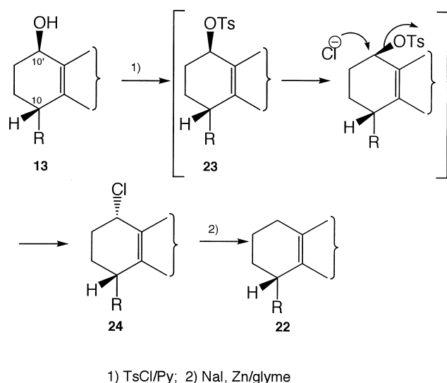
Fig. 7. Formation of bisacutifolone C (22) from bisacutifolone A (13).
