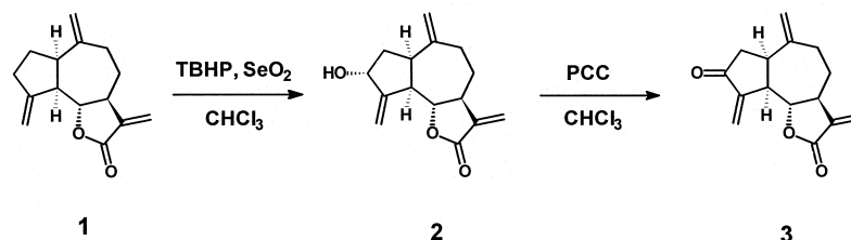
Fig. 1. Semi-synthesis of dehydrozalanin C (3) from dehydrocostuslactone (1).
