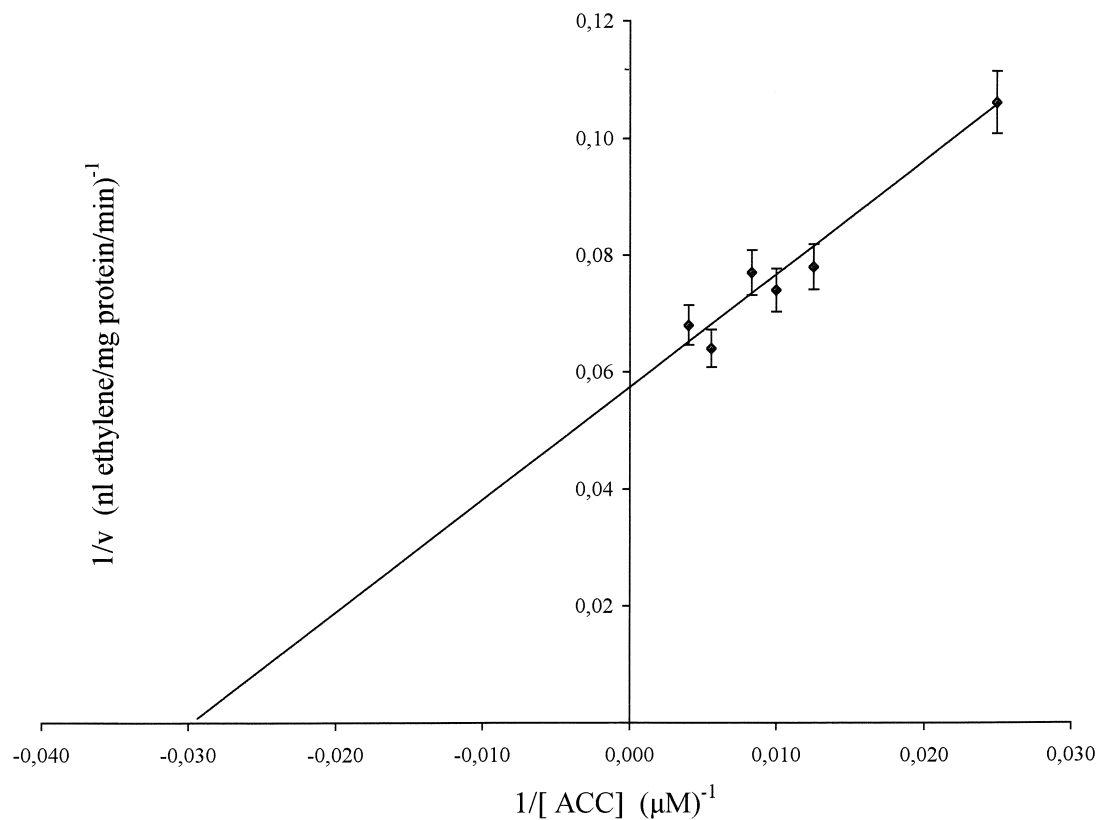
Fig. 2. Double reciprocal plot (Lineweaver–Burk) of ACO activity vs concentration of ACC. K_m \approx 30 \mu M .
