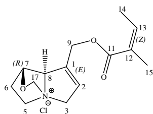
(7 R , 8 R )-Petranine ( 3a )
