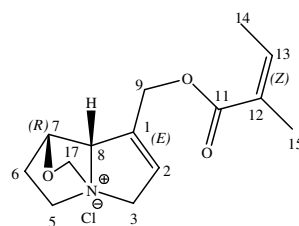
(7 R , 8 S )-Petranine ( 3b )
