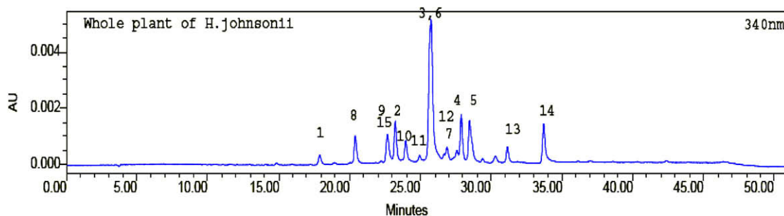
Fig. 1. The HPLC–UV chromatogram of the methanol extract of Halophila johnsonii .
