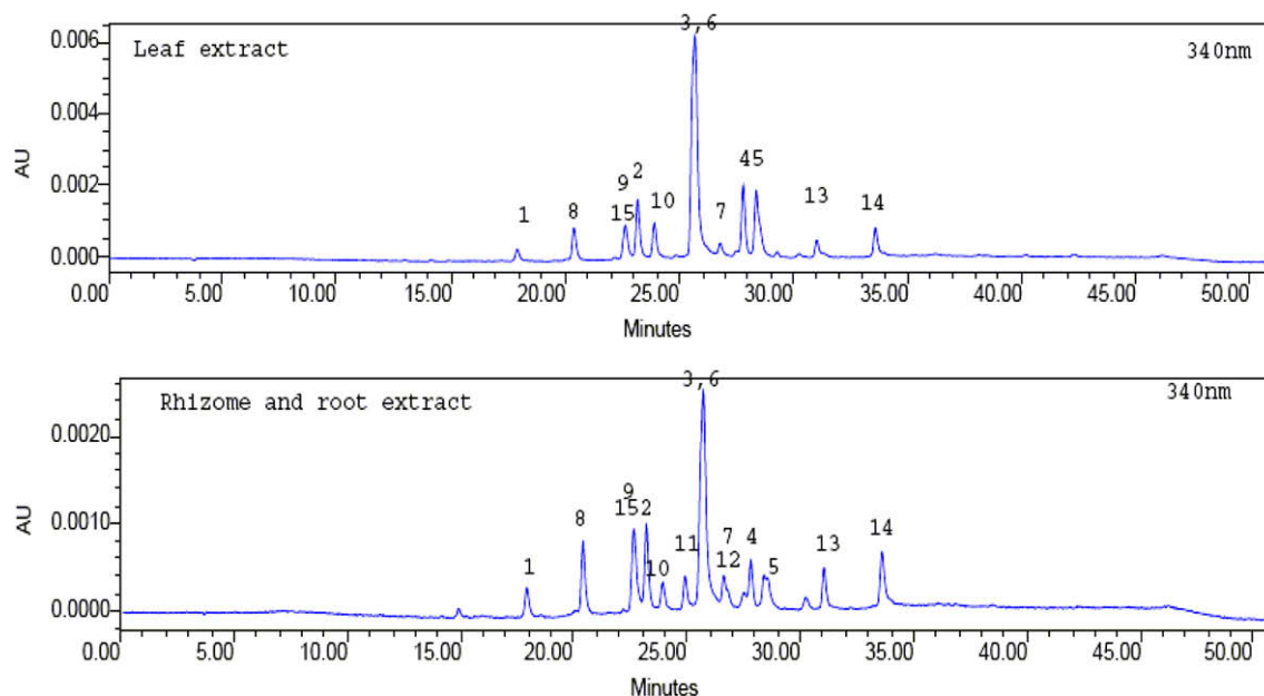
Fig. 2. HPLC-UV chromatograms of Halophila johnsonii leaf, rhizome and root extracts.
