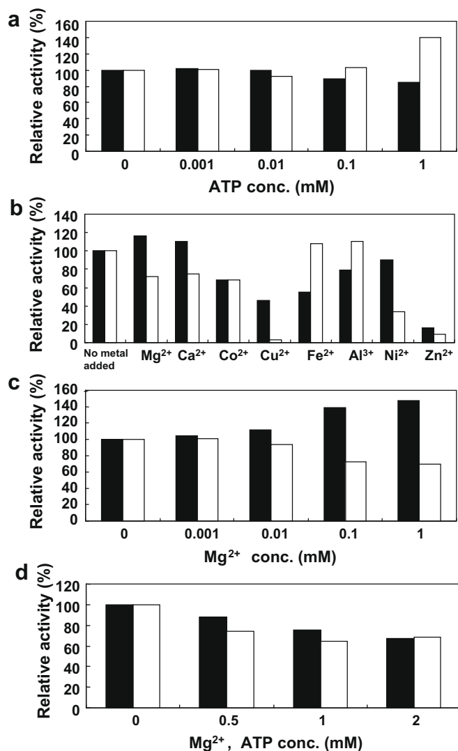
Fig. 6. Effects of metal ions and ATP on serine racemase activity. (a) Effect of ATP; (b) effects of various metal ions; (c) effect of Mg 2+ ; (d) effects of Mg 2+ and ATP. Reactions were carried out according to the methods described in Section 3.6. Black bar: serine racemase activity of SerR; white bar: L-serine dehydratase activity of SerR.
