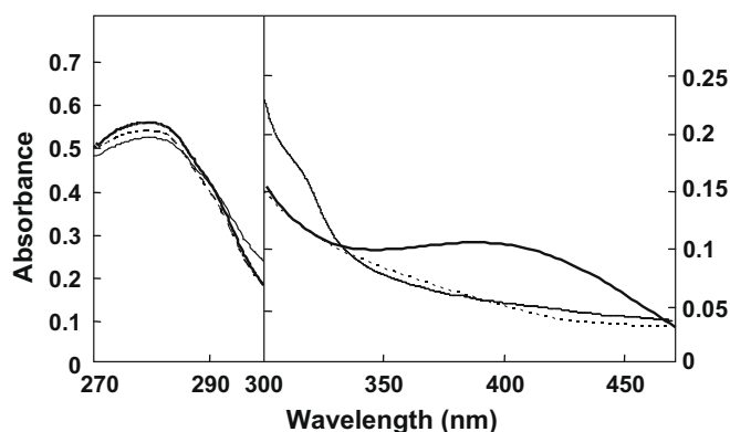
Fig. 5. Absorption spectra of serine racemase from Oryza sativa L. Solid line: the holo SerR (1 mg/ml in a 10 mM sodium phosphate buffer (pH 8.0) containing 10 mM PLP and 0.02% 2-mercaptoethanol); Narrow line: the reduced form of SerR (1 mg/ml in a 10 mM sodium phosphate buffer (pH 8.0) containing 0.02% 2-mercaptoethanol after reduction with NaBH 4 ); Dashed line: the apo SerR (1 mg/ml in a 10 mM sodium phosphate buffer (pH 8.0) containing 0.02% 2-mercaptoethanol). The spectra were taken with a Jasco V550 spectrophotometer (Jasco, Tokyo) at room temperature (about 25 °C).
