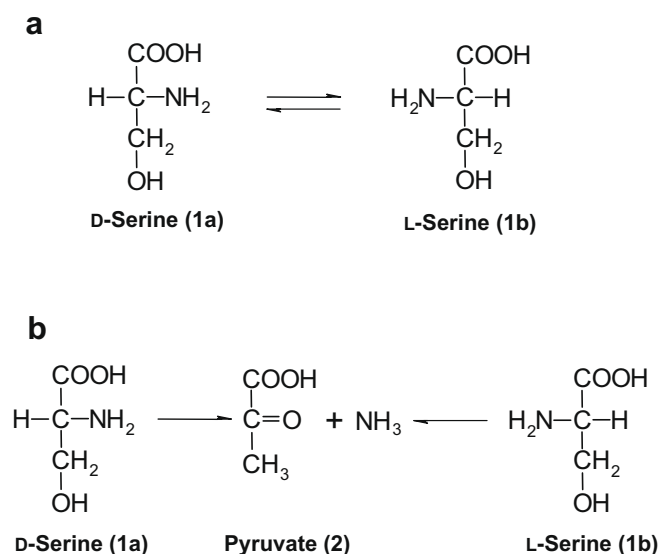
Fig. 1. Reaction pathways of D-serine ( 1a ) and L-serine ( 1b ) by serine racemase from Oryza sativa L. (a) Racemase reaction; (b) Dehydratase reaction.
