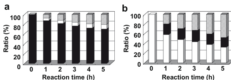
Fig. 4. Time course of the reaction products of serine racemase from Oryza sativa L. (a) D-Serine ( 1a ) was used as substrate. (b) L-Serine ( 1b ) was used as substrate. The preparation of a reaction mixture and the measurement of D- and L-serine ( 1a and 1b ) and pyruvate were conducted according to the method described in Section 3.6. An aliquot (500 µl) was taken from the reaction mixture after 0, 1, 2, 3, 4, and 5 h. Black bar: D-serine, white bar: L-serine, striped bar: pyruvate.
