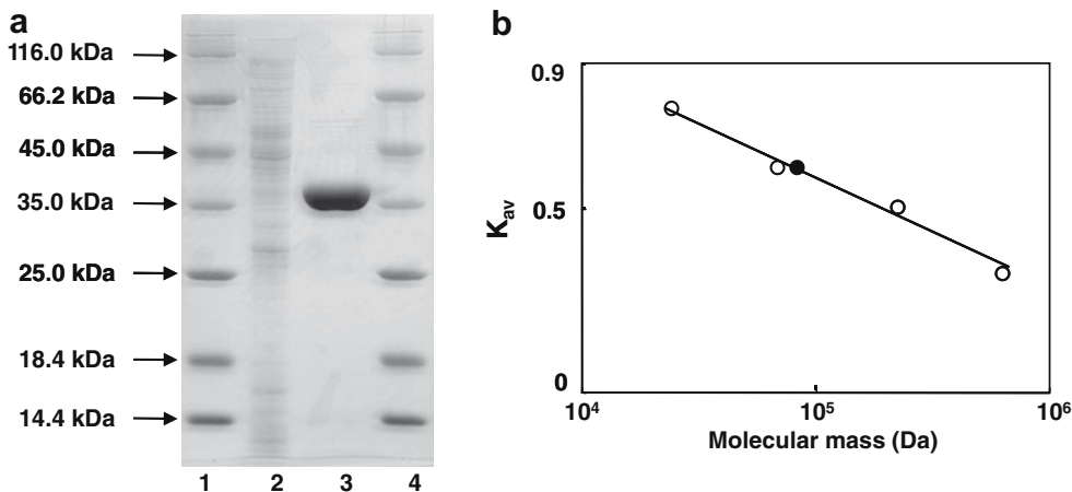
Fig. 3. Subunit and quaternary structures of the serine racemase from Oryza sativa L. (a) SDS-PAGE Electrophoresis was conducted with a Ready gel cell 108 BR (Bio-Rad Japan, Tokyo) equipped with a Power pac 300 (Bio-Rad). The concentration of acrylamide was 12%T. Lane 1: protein marker: \beta -galactosidase from Escherichia coli , 116.0 kDa; bovine serum albumin from bovine plasma, 66.2 kDa; ovalbumin from chicken egg white, 45.0 kDa; lactate dehydrogenase from porcine muscle, 35.0 kDa; restriction endonuclease Bsp 981 from E. coli , 25.0 kDa; \beta -galactoglobulin from bovine milk, 18.4 kDa; lysozyme from chicken egg white, 14.4 kDa. Lane 2: a crude extract of E. coli BL21 (DE3) cells harboring pET-21b/serr (protein: 8 \mu g). Lane 3: purified SerR (protein: 8 \mu g). Lane 4: protein marker. (b) Gel filtration. K_{av} values were calculated according to the equation of K_{av} = V_e - V_0 / V_t - V_0 , where V_e is the elution volume for the protein, V_0 is the column void volume, i.e., an elution volume for Blue Dextran 2000, and V_t is the total bead volume. The mobile phase used was 10 mM potassium phosphate buffer containing 300 mM NaCl. The flow rate was 0.3 ml/min. The column and protein marker used are described in Section 3.11.
