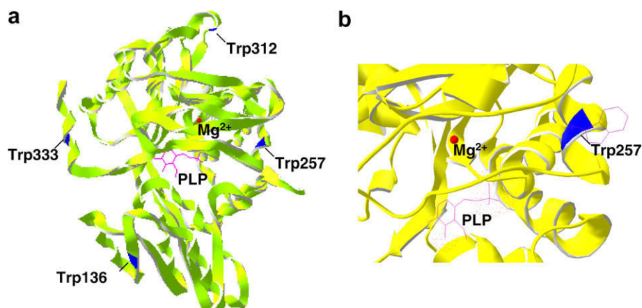
Fig. 7. Proposed three-dimensional subunit structure of serine racemase from Oryza sativa L. (a) Subunit structure: The three-dimensional subunit structure of SerR (yellow ribbon) was superimposed on that of serine racemase from Schizosaccharomyces pombe (yellowish-green ribbon). Mg^{2+} is shown as a red sphere. (b) Active site of SerR: Trp257, PLP, and Mg^{2+} are shown as a blue ribbon with purple sticks, pink sticks, and a red sphere, respectively. The structures were estimated by the method described in Section 3.11.
