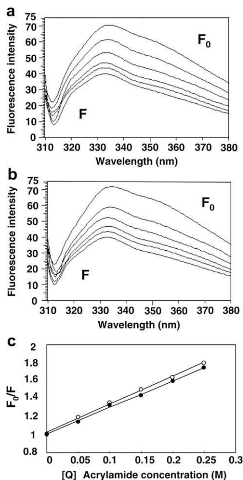
Fig. 8. Quenching of SerR tryptophan fluorescence by acrylamide. (a) Fluorescence spectra in the absence of Mg^{2+} . (b) Fluorescence spectra in the presence of Mg^{2+} . (c) Stern-Volmer plot. The experiment was carried out according to the method described in Section 3.10.
