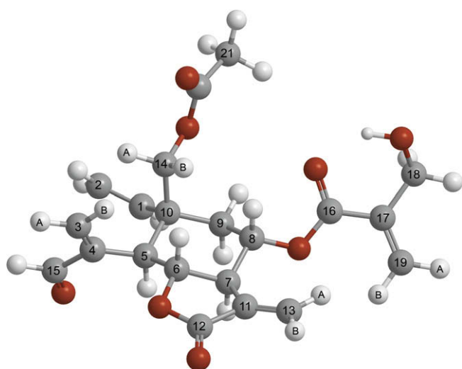
Fig. 4. Model of preferred conformation of 2 [ChemBio3D Ultra, dihedral driver (resolution 1^\circ ) with calculated energy minima (MM2) for each step].
