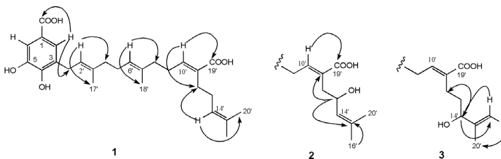
Fig. 1. Selected ^1\text{H} – ^{13}\text{C} (HMBC) correlations for compounds 1–3.
