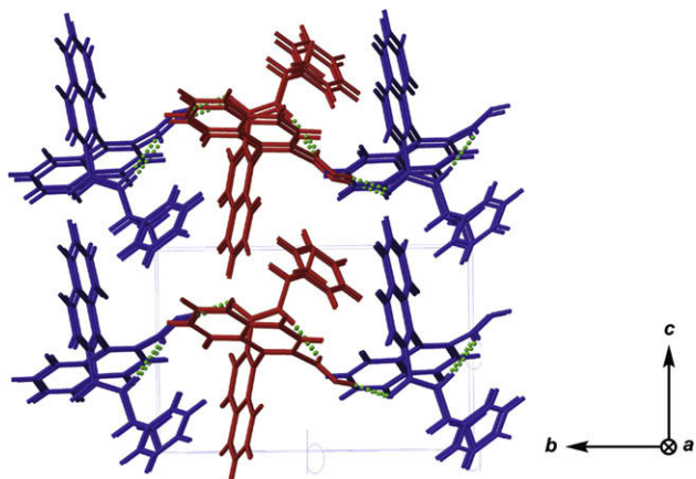
Figure 1. Crystal structure of (R_a,S) -1. Molecules are color-coded according to their orientations. Dotted lines indicate hydrogen bonds.
