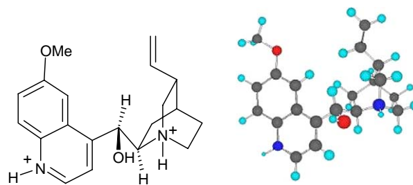
Preferred conformation of protonated epiquinidine 15
