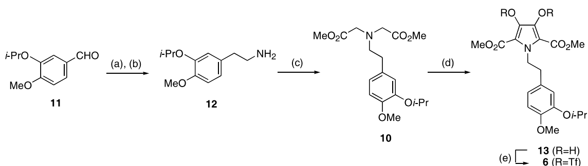
Scheme 2. Synthesis of 3,4-dihydroxypyrrrole bistriflate 6. Reagents and conditions: (a) CH 3 NO 2 , AcO - NH 4 + , AcOH, 100 °C, 6 h (74%); (b) LiAlH 4 , THF, reflux, 7 h (65%); (c) BrCH 2 CO 2 Me, NaHCO 3 , CH 3 CN, reflux, 2 h (83%); (d) (CO 2 Me) 2 , NaH, THF, reflux, 3 h (87%); (e) (CF 3 SO 2 ) 2 O, pyridine, 0 °C, 2 h (91%).
