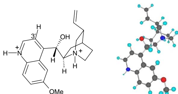
Preferred conformation of protonated quinidine 12
