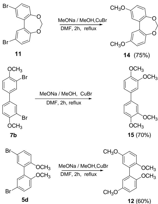
Scheme 3. Methoxylation of halogenated biphenyls.
