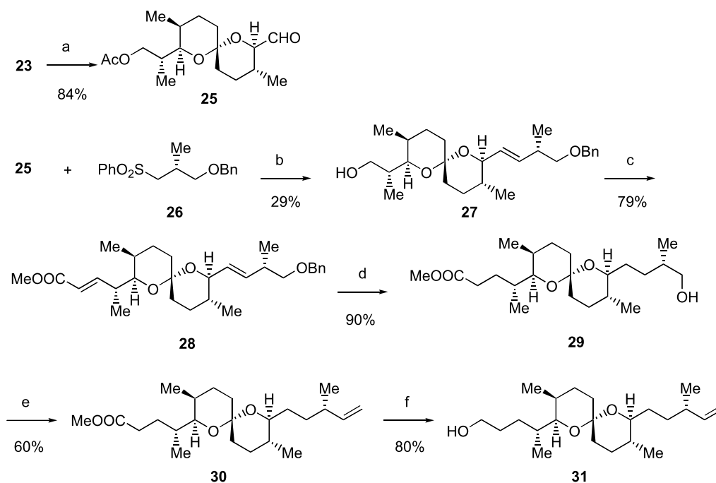
Scheme 5. (a) Dess–Martin oxidn; (b) (i) n -BuLi, THF, -50\text{ }^{\circ}\text{C} (ii) \text{Ac}_2\text{O} , DMAP, pyridine (iii) 5% Na(Hg), MeOH, 50\text{ }^{\circ}\text{C} ; (c) (i) Dess–Martin oxidn (ii) \text{Ph}_3\text{P}=\text{CHCOOMe} , \text{CH}_2\text{Cl}_2 (d) \text{H}_2 , \text{Pd}(\text{OH})_2\text{-C} , MeOH; (e) (i) Dess–Martin oxidn (ii) \text{Ph}_3\text{PMe}^+\text{-Br}^- , n -BuLi, THF, 0\text{ }^{\circ}\text{C} ; (f) \text{LiAlH}_4 , THF, 0\text{ }^{\circ}\text{C} .
