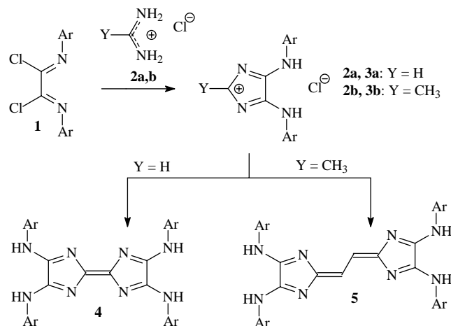
Scheme 1. The cyclization reaction of bis-imidoylchlorides 1 with formamidine and acetamidine.
