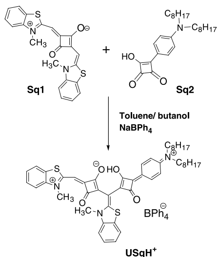
Scheme 1. Synthetic scheme of USqH + .
