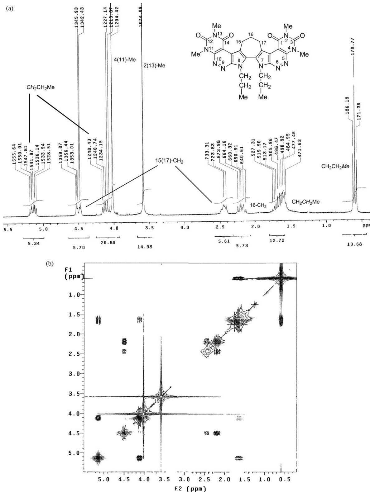
Figure 1. 1 H NMR spectrum of compound 12a . (a) 1 H NMR spectra of compound 12a (CDCl 3 , 300 MHz); (b) 1 H- 1 H COSY NMR spectra of compound 12a .
