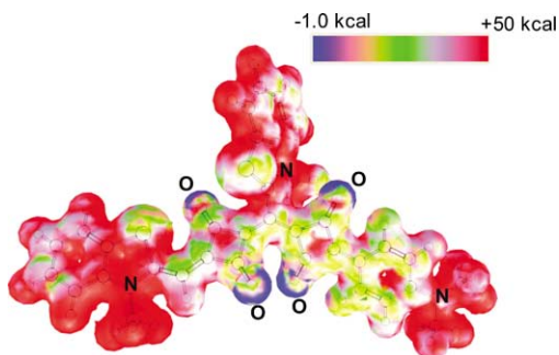
Figure 9. The MESP mapped on to the van der Waals surface of \text{USqH}^+ at BLYP/6-31G* level showing the high negative potential around oxygen atoms and high positive potential around nitrogen atoms revealing the zwitterionic character of the system.
