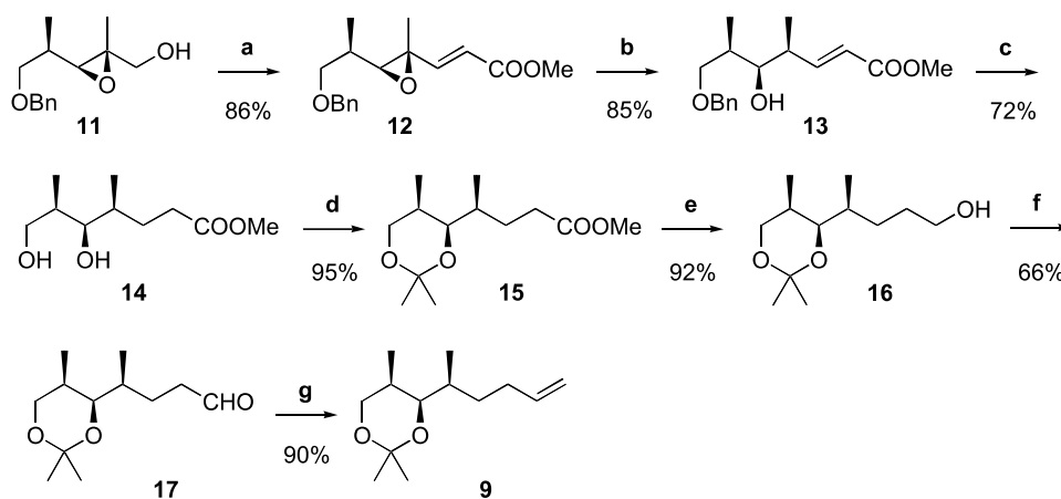
Scheme 3. (a) (i) Dess–Martin oxidn (ii) \text{Ph}_3\text{P}=\text{CHCOOMe} , DMSO; (b) \text{Pd}(\text{dba})_3 , \text{Ph}_3\text{P} , \text{HCOOH} , \text{Et}_3\text{N} , dioxane; (c) \text{H}_2 , \text{Pd}(\text{OH})_2\text{-C} , MeOH; (d) (\text{MeO})_2\text{CMe}_2 , \text{TsOH}\cdot\text{H}_2\text{O} ; (e) DIBAL-H, toluene, -78^\circ\text{C} ; (f) TPAP, NMO, \text{CH}_2\text{Cl}_2 ; (g) \text{Ph}_3\text{PMe}^+\text{Br}^- , n -BuLi, THF.
