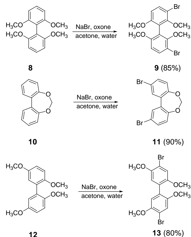
Scheme 2. Selective halogenation of biphenyls.
