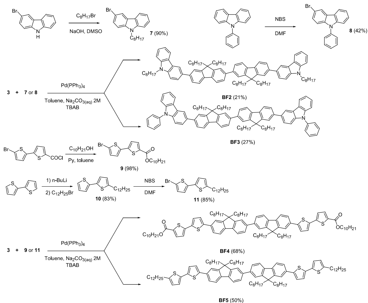
Scheme 2. Synthetic sequences for the preparation of BF2–5 .
