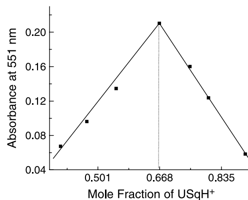
Figure 3. Job plot for the binding of USqH + with \text{Hg}^{2+} .
