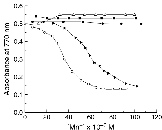
Figure 5. Effect of metal ions on the absorbance at 770 nm for solutions of USqH + ( 11.6 \times 10^{-6} \text{ M} ) in dichloromethane. ( \Delta ) \text{Na}^+ , ( \blacksquare ) \text{Ca}^{2+} , ( \bullet ) \text{Zn}^{2+} , ( \blacktriangleright ) \text{Pb}^{2+} and ( \circ ) \text{Hg}^{2+} containing \text{Na}^+ (0.1 mM) + \text{Ca}^{2+} (0.1 mM) + \text{Zn}^{2+} (0.1 mM).
