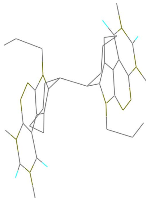
Figure 3. View on the molecule 13a , showing anti -periplanar orientation of the cycloheptyl rings respectively the C(15)–C(15A) bond (without hydrogen atoms).
