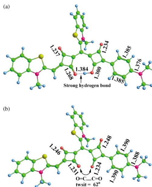
Figure 8. Geometries of (a) \text{USqH}^+ and (b) \text{USq} optimized at BLYP/6-31G(d) level.
