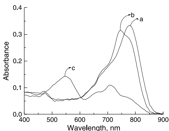
Figure 6. Absorption spectra of \text{USqH}^+ ( 7.9 \times 10^{-6} \text{ M} ) in dichloromethane containing (a) no metal ions (b) 90 \mu\text{M Cu}^{2+} , (c) 29 \mu\text{M Hg}^{2+} + 90 \mu\text{M Cu}^{2+} .
