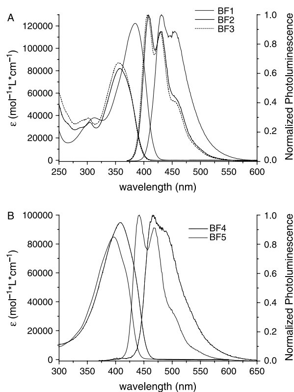
Figure 1. Absorption and emission spectra of BF1–3 (A) and BF4–5 (B) in chloroform solution (concentration: 1.0 \times 10^{-5} M for absorption and 1.0 \times 10^{-6} M for fluorescence).
