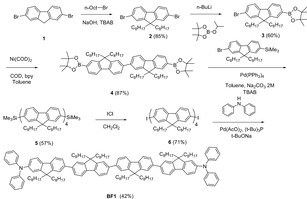
Scheme 1. Synthetic sequence for the obtention of BF1 .
