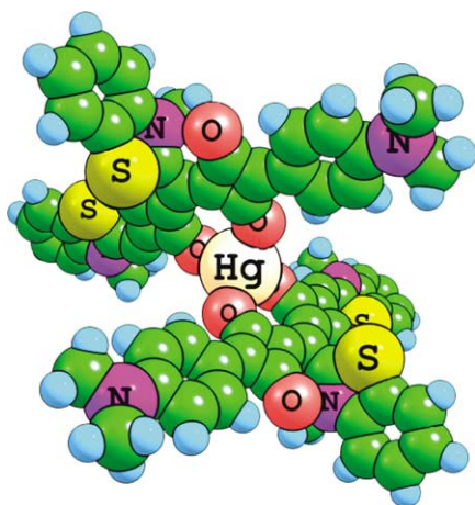
Figure 10. Molecular structures of (\text{USq})_2\text{Hg}^{2+} complex obtained from BLYP/6-31G* level calculation.
