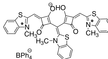
Figure 1. SqH + with counter anion \text{BPh}_4^- .
