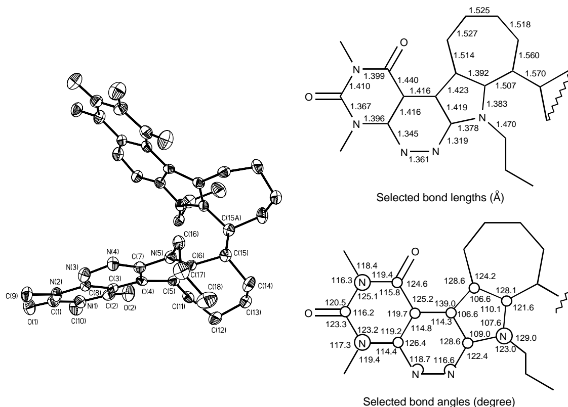
Figure 2. The molecular structure of 13a with crystallographic numbering scheme (hydrogens are omitted for clarity).
