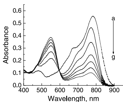
Figure 2. Effect of \text{Hg}^{2+} on the absorption spectrum of USqH + ( 12.9 \times 10^{-6} \text{ M} ) in dichloromethane (a) 0, (b) 25, (c) 28, (d) 31, (e) 34, (f) 38 and (g) 49 \mu\text{M} \text{Hg}^{2+} .
