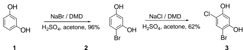
Scheme 1. Selective halogenation of activated aryls.
