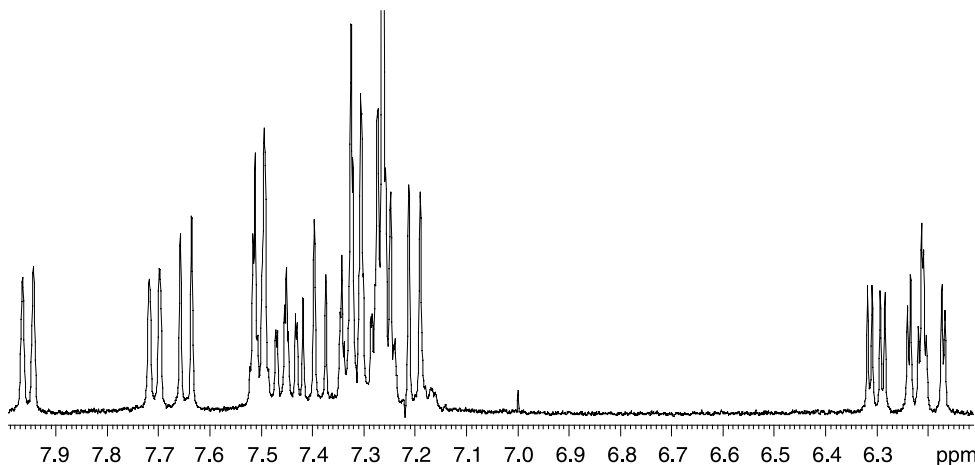
Figure 1. 1 H NMR spectrum (6–8 ppm) of Naphthopyran 13b .
