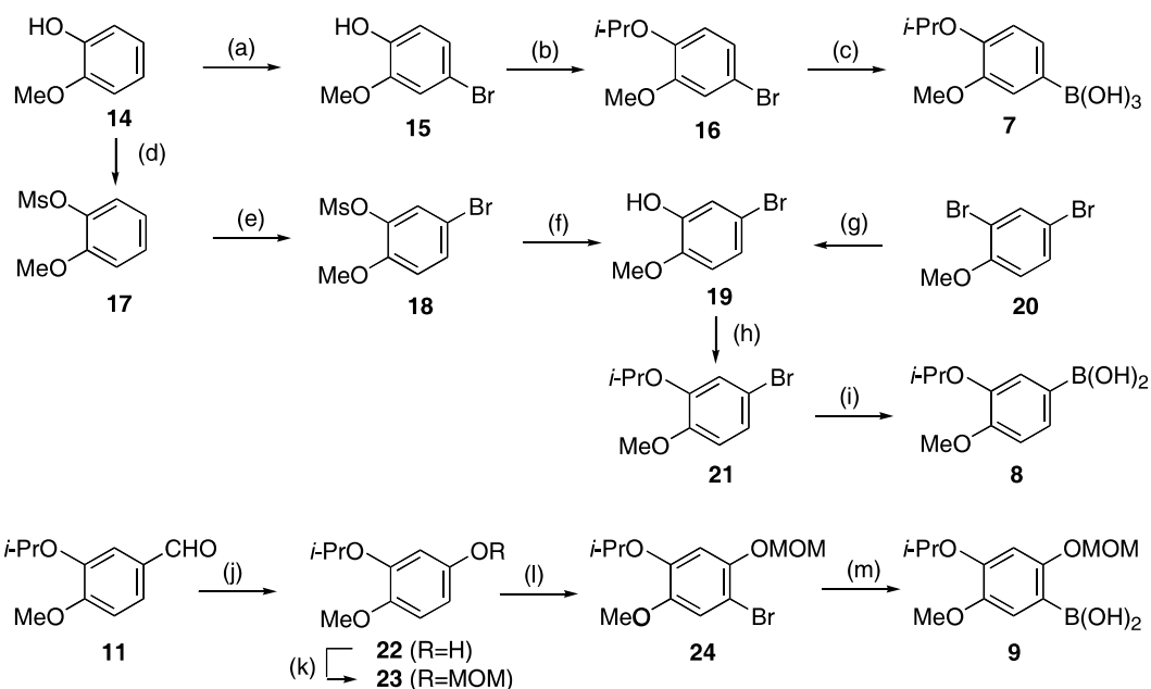
Scheme 3. Synthesis of arylboronic acids 7, 8, and 9. Reagents and conditions: (a) NBS, DMF, 0 °C, 0.5 h (86%); (b) i -PrBr, K 2 CO 3 , DMSO, 55 °C, 2 h (84%); (c) (1) t -BuLi, THF, -78 °C, 1 h, (2) B(OMe) 3 , -78 °C, 1 h, then rt, 1 h (56%); (d) CH 3 SO 2 Cl, Et 3 N, CH 2 Cl 2 , 0 °C, 0.5 h (96%); (e) NBS, DMF, rt, 24 h (96%); (f) LDA, THF, 0 °C, 5 min (91%); (g) (1) n -BuLi, Et 2 O, -78 °C, 1 h, (2) B(OMe) 3 , -78 °C, 1 h, then rt, 1 h, (3) 30% H 2 O 2 , AcOH, rt, 16 h (91%); (h) i -PrBr, K 2 CO 3 , DMSO, 55 °C, 2 h (96%); (i) (1) t -BuLi, THF, -78 °C, 1 h, (2) B(OMe) 3 , -78 °C, 1 h, then rt, 1 h (81%); (j) (1) m CPBA, CH 2 Cl 2 , 0 °C, 3 h, (2) K 2 CO 3 , MeOH, rt, 1 h (86%); (k) MOMCl, NaH, THF, 0 °C, 2 h, then rt, 1 h (68%); (l) NBS, DMF, 0 °C, 0.5 h, (98%); (m) (1) t -BuLi, THF, -78 °C, 1 h, (2) B(OMe) 3 , -78 °C, 1 h, then rt, 1 h (87%).
