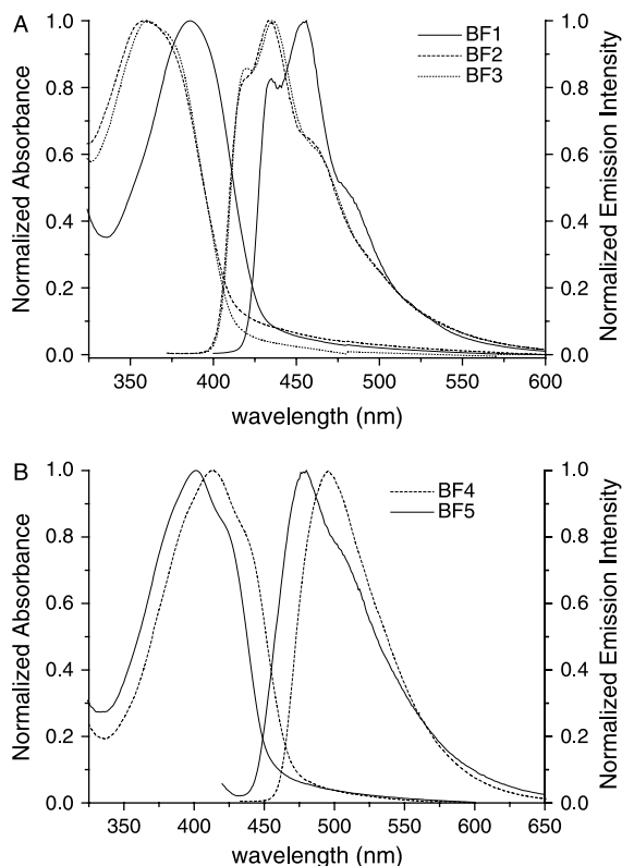
Figure 2. Absorption and emission spectra of BF1–3 (A) and BF4–5 (B) in the solid state (films obtained by spin coating from 5 mg/ml chloroform solutions).
