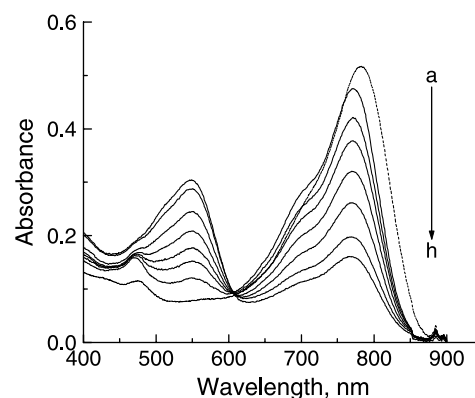
Figure 4. Effect of \text{Pb}^{2+} on the absorption spectrum of USqH + ( 12 \times 10^{-6} \text{ M} ) in dichloromethane (a) 0, (b) 36, (c) 47, (d) 53, (e) 59, (f) 68, (g) 82, (h) 93 \mu\text{M} \text{Pb}^{2+} .
