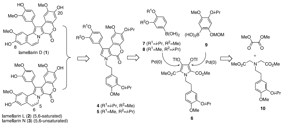
Scheme 1. Retrosynthetic analysis of lamellarins D (1), L (2), and N (3).
