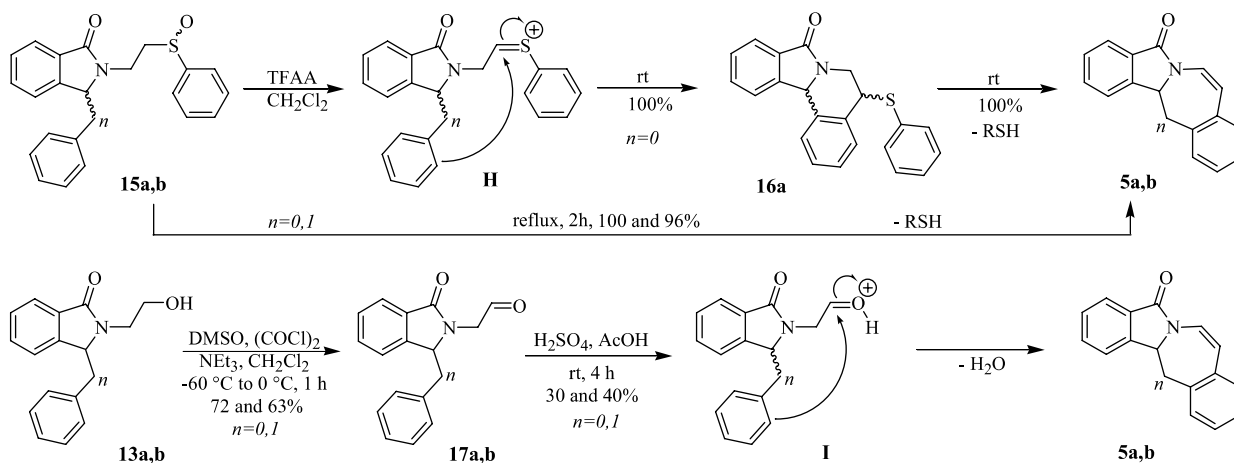
Scheme 4. The \pi -cationic cyclization of sulfoxides 15a,b and corresponding formyl derivatives 17a,b into isoindolinones 5a,b under acidic conditions.
