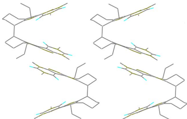
Figure 4. The cut of the crystal packing of compound 13a (without hydrogen atoms).
