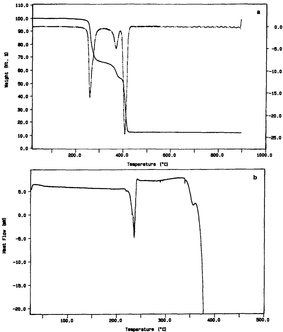
Fig. 3. \text{CuBenz}_4(\text{NO}_3)_2 : (a) — TG curve, - - - DTG curve; (b) — DSC curve; scanning rate: 10^{\circ}\text{C min}^{-1} ; air flow 50\text{--}100\text{ mL min}^{-1} .
