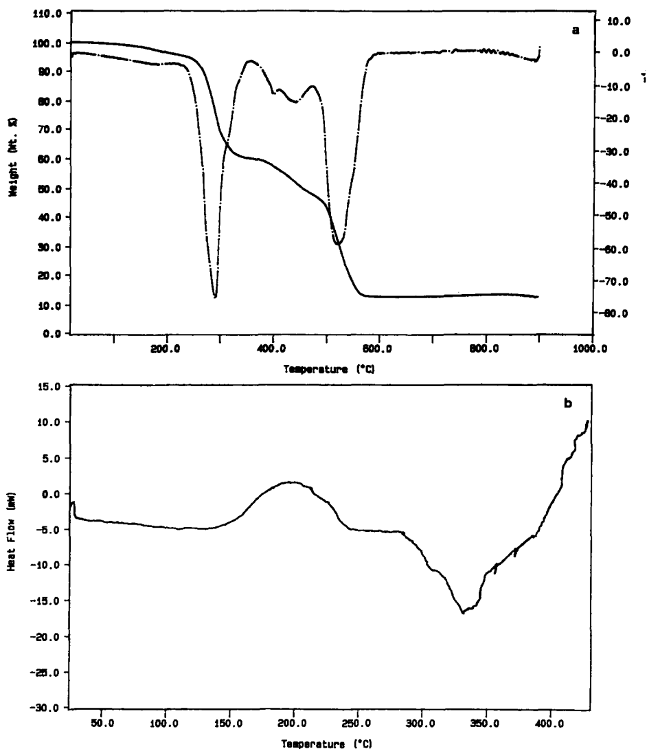
Fig. 4. \text{CuBenz}_4\text{SO}_4 : (a) — TG curve, - - - DTG curve; (b) — DSC curve; scanning rate: 10^{\circ}\text{C min}^{-1} ; air flow 50\text{--}100\text{ mL min}^{-1} .
