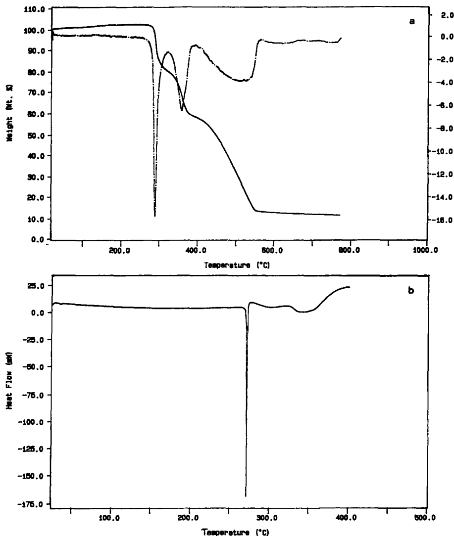
Fig. 5. \text{CuBenz}_4(\text{ClO}_4)_2 (a) — TG curve, - - - DTG curve; (b) — DSC curve; scanning rate: 10^\circ\text{C min}^{-1} ; oxygen flow 50\text{--}100\text{ mL min}^{-1} .
