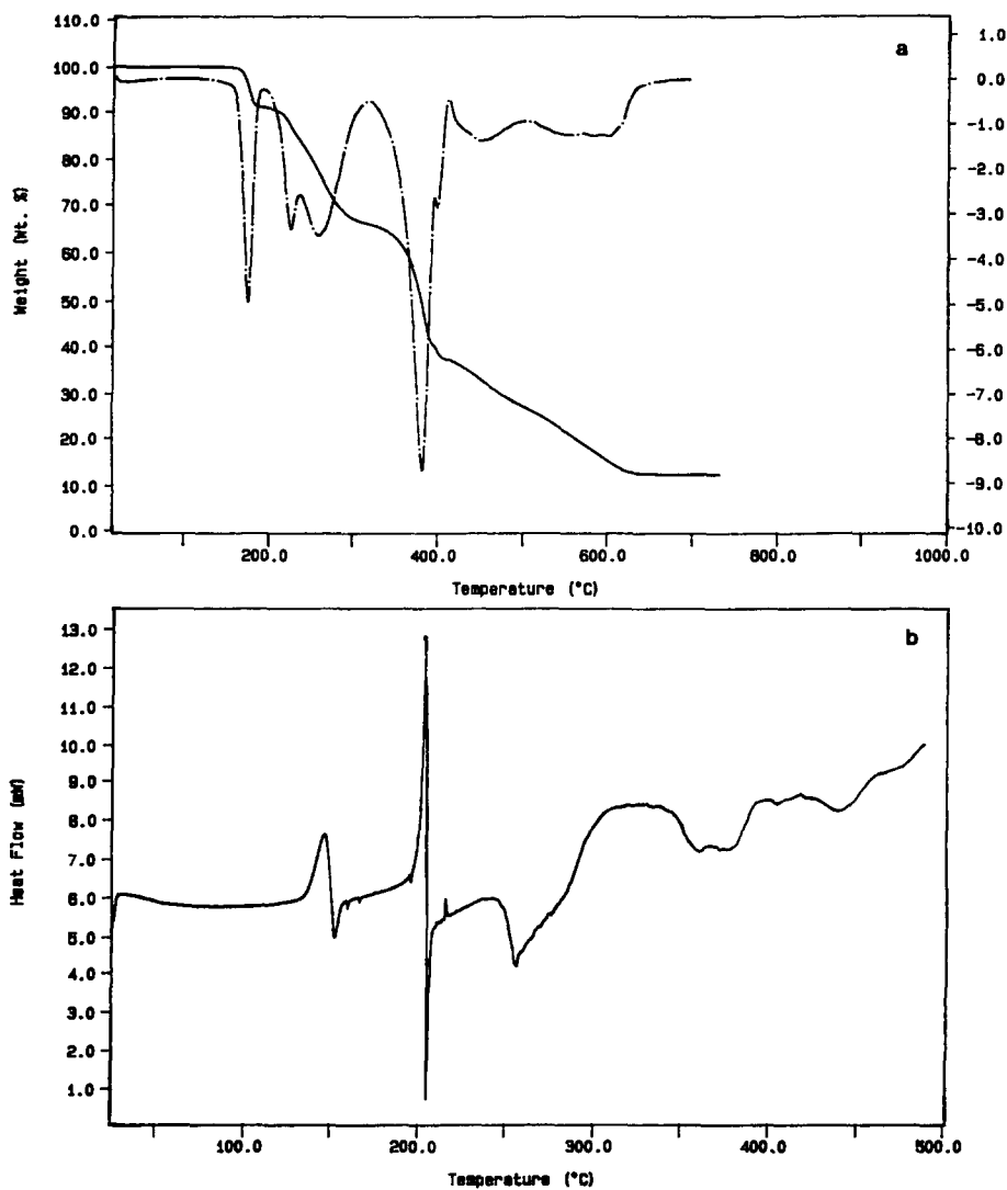
Fig. 1. \text{CuBenz}_4\text{Cl}_2 \cdot 3\text{H}_2\text{O} : (a) — TG curve, --- DTG curve; (b) — DSC curve; scanning rate: 10^{\circ}\text{C min}^{-1} , air flow 50\text{--}100\text{ ml min}^{-1} .
