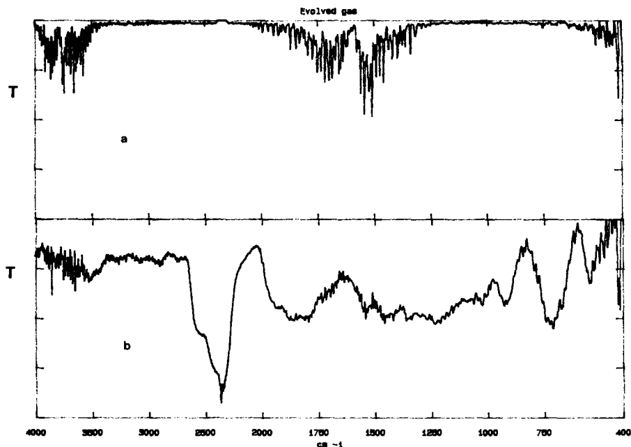
Fig. 7. TG-FTIR spectra: infrared spectra of the gas evolved during the TG steps; resolution: 4\text{ cm}^{-1} .
