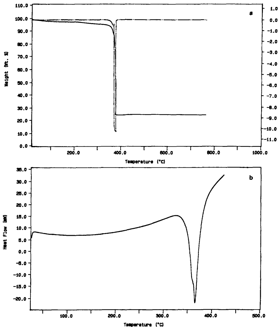
Fig. 6. CuBenz 2 : (a) — TG curve, --- DTG curve; (b) — DSC curve; scanning rate: 10°C min -1 ; oxygen flow 50–100 mL min -1 .
