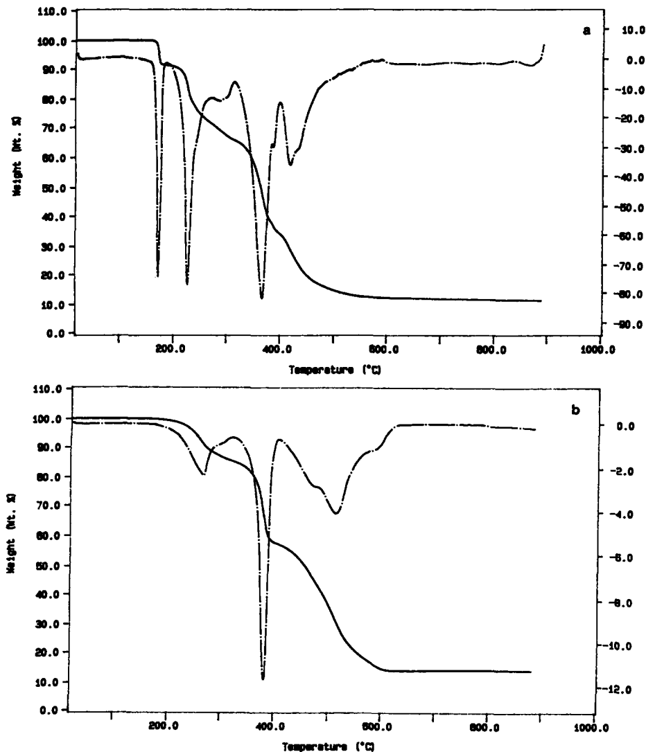
Fig. 8. (a) \text{CuBenz}_4\text{Cl}_2 \cdot 3\text{H}_2\text{O} (dimeric): (a) — TG curve, - - - DTG curve; (b) \text{CuBenz}_4\text{Cl}_2 (monomeric): — TG curve, - - - DTG curve; scanning rate: 10^\circ\text{C min}^{-1} ; oxygen flow 50\text{--}100\text{ mL min}^{-1} .
