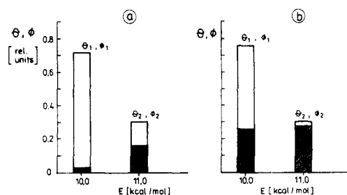
Fig. 7. Schematic diagrams of the discrete-energy spectra of the defect sites \phi(E) and the degree of occupation of the defect sites by inert gas introduced at: (a) labelling pressure p=0.5 relative units; and (b) labelling pressure p = 10 relative units. The effective activation energies E and corresponding degrees of occupation of the defect sites used are: E_1=10 \text{ kcal mol}^{-1} , \phi=0.7 and E_2=11 \text{ kcal mol}^{-1} , \phi=0.3 .
