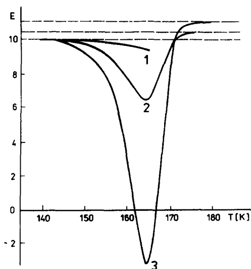
Fig. 6. Temperature dependences of the effective activation energy E_{ef} of the inert gas diffusion calculated at every point of the model TIGRA curves corresponding to the discrete energetic spectrum characterized by Fig.4 (curves 1–3 correspond to the schemes (a)–(c) respectively).
