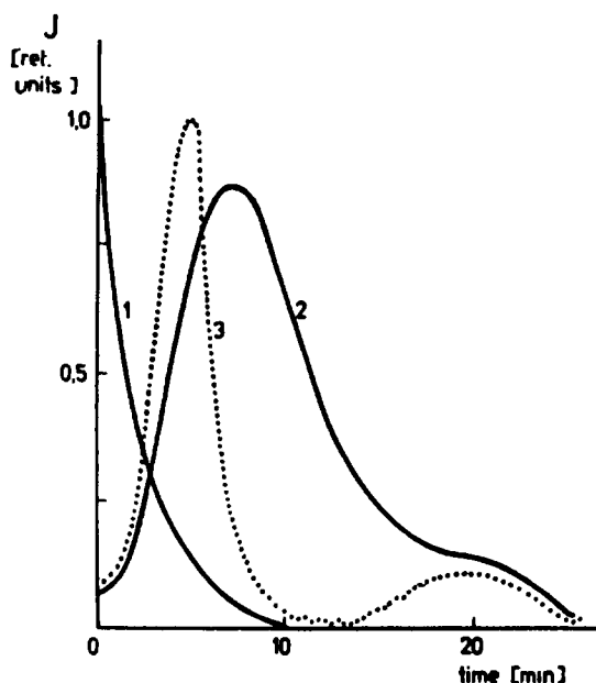
Fig. 10. The reconstruction of the experimentally obtained TIGRA curve of a polypropylene foil in the temperature range from -196 to +400^{\circ}\text{C} (heating rate 4\text{ min}^{-1} ) which was labelled with ^{222}\text{Rn} : curve (1)-the apparatus response to the "one second pulse", curve (2) - the experimentally obtained TIGRA curve; curve (3)-the reconstructed TIGRA curve.
