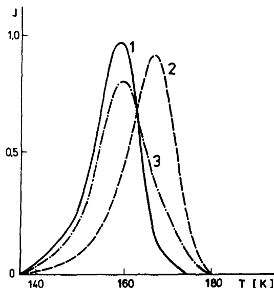
Fig. 5. Model curves of the temperature dependences of the thermostimulated inert gas release (TIGRA curves) for the selected cases of the discrete energy spectra of the single energy value E_1=10.0 and 10.5 kcal mol ^{-1} , respectively: curve 3 corresponds to the spectrum characterized by two discrete energy values E_1=10.0 kcal mol ^{-1} and E_2=10.5 kcal mol ^{-1} . In the modelling, the heating rate 2.0 Ks ^{-1} and the pre-exponential factor 10^{13} s ^{-1} were considered.
