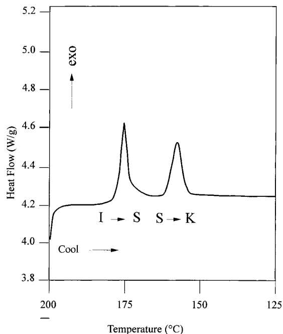
Fig. 2. Cooling scans of BB8 recorded on a power-compensation instrument (Perkin-Elmer DSC 7, 10^{\circ}\text{C}/\text{min} ). In the cooling scan, the transitions are well separated.
