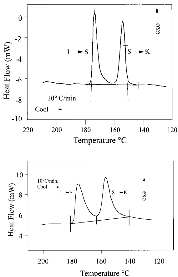
Fig. 3. (a) Cooling scan of BB8 at -10^{\circ}\text{C}/\text{min} on Setaram DSC 141 (power-compensation instrument, wt. 8.98 mg). The transitions are well separated. (b) Cooling scan of BB8 on Setaram DSC 92 (heat-flux instrument, wt. 8.78 mg) at -10^{\circ}\text{C}/\text{min} . There is some overlap.
