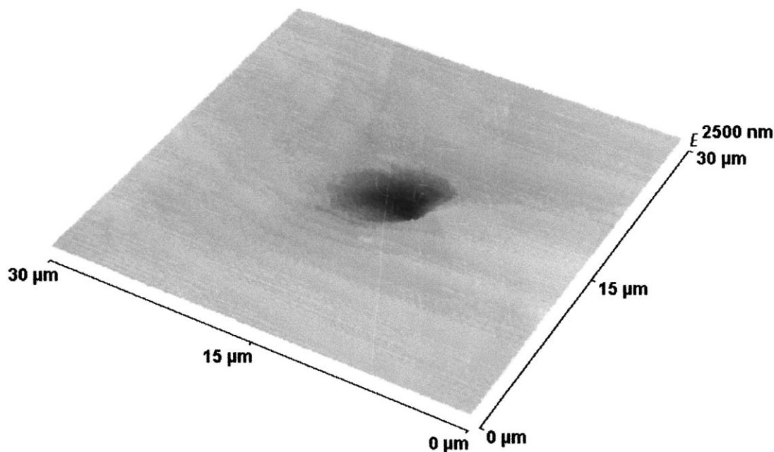
Fig. 2. Three-dimensional perspective view of a pyrolysis crater on a poly(methyl methacrylate) sheet.
