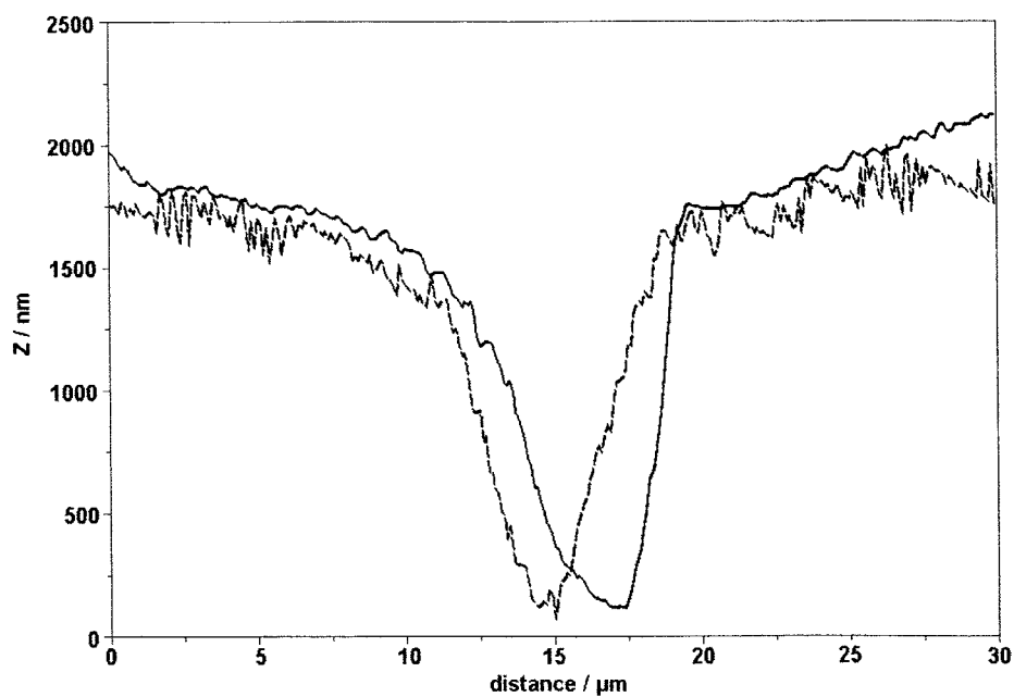
Fig. 3. Line profiles horizontally (—) and vertically (---) across the crater in Fig. 2.
