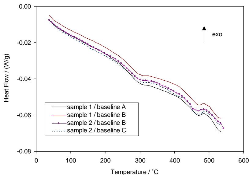
Fig. 1. Sample run minus baseline run of the Al-1.3 at.%Mg-0.4 at.%Mn-0.07 at.%Cu 10% deformation samples aged for 21 days at 170 °C. Four measurements are shown, which are formed from combinations of two DSC runs on the alloy samples and three different baselines.
