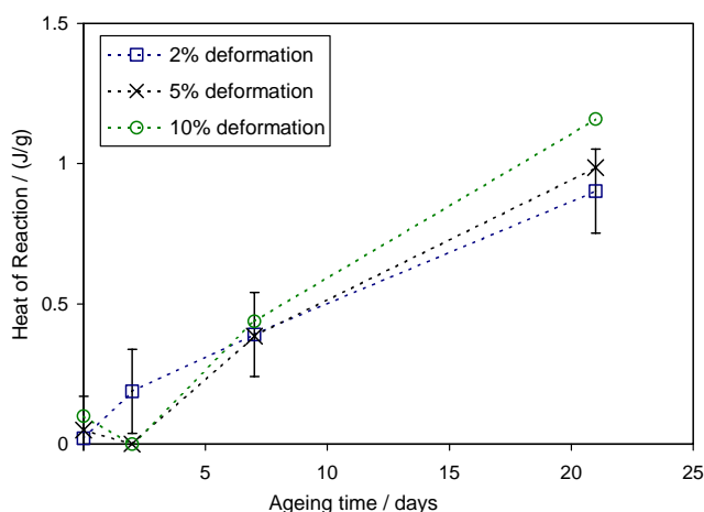
Fig. 5. Heat content of the exothermic effect with peak at 300 °C for the aged Al–1.3 at.% Mg–0.4 at.% Mn–0.07 at.% Cu with three levels of cold deformation.
