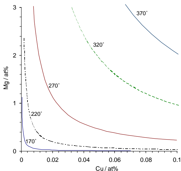
Fig. 6. Solvi of S phase at 170, 220, 270, 320 and 370 °C.
