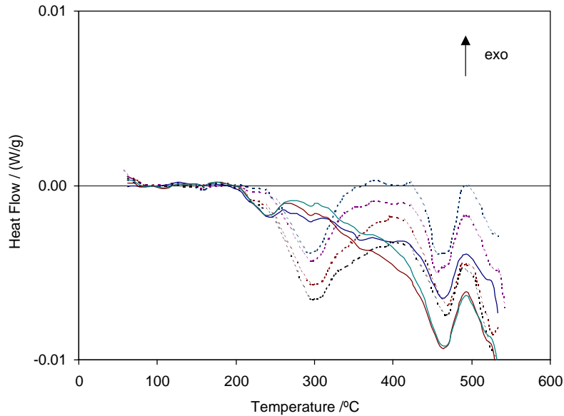
Fig. 3. Thermograms corrected for baseline run and heat capacity (linear function) of the Al–1.3 at.%Mg–0.4 at.%Mn–0.07 at.%Cu 10% deformation samples aged for 2 days (solid lines) and for 21 days (dotted lines) at 170 °C.
