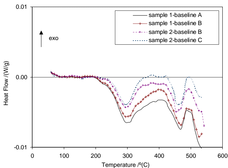
Fig. 2. Thermograms corrected for baseline run and heat capacity (linear function) of the Al-1.3 at.%Mg-0.4 at.%Mn-0.07 at.%Cu 10% deformation samples aged for 21 days at 170 °C. Four measurements are shown, which are formed by two samples and two baselines for each sample.
