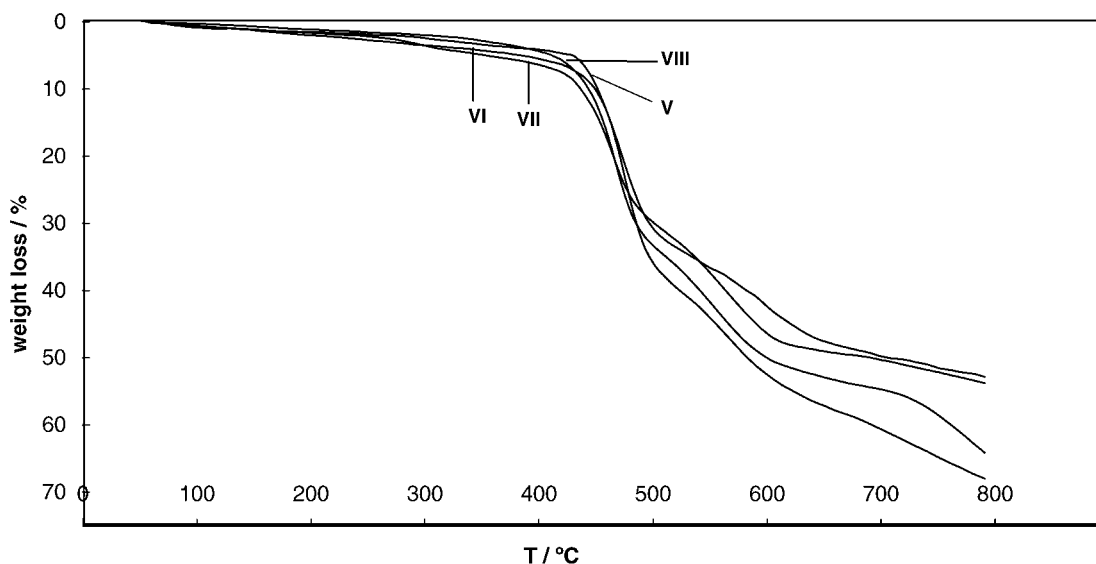
Fig. 2. Thermogravimetric curves for poly(esters) V–VIII.
