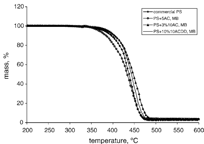
Fig. 12. TGA analysis for nanocomposites prepared melt blending.
