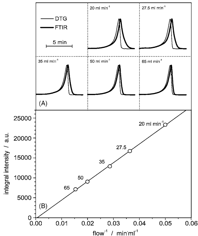
Fig. 7. (A) Pinhole calibration of ethanol with varying carrier flow rate, sample size: 25 mg, heating rate: 10 K min -1 , DTG (thin) and FTIR (thick lines). (B) The relationship between the integral intensity and the reciprocal of the flow rate defined as the ratio of injected volume (1 ml) to the flow rate of carrier gas (ml min -1 ), which are marked on the data.
