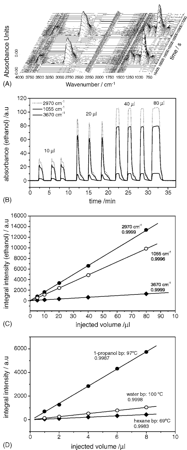
Fig. 3. (A) 3D FTIR-diagram of the calibration of ethanol (one pulse: 5 \mu l). (B) Ethanol traces due to different integration methods at three characteristic wavelengths for ethanol (1055, 2970 and 3670 \text{cm}^{-1} ). (C) Linear dependence between the integral intensity of the FTIR signals on the amount of injected ethanol. (D) Linear dependence between the intensity of the FTIR signals on the amount of injected liquids (1-propanol, water and hexane).
