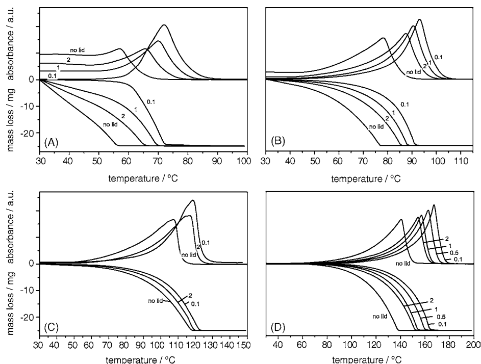
Fig. 6. Pinhole calibration of acetone (A), ethanol (B), water (C) and hexanol (D), sample mass: 25 mg, heating rate: 10 K min -1 , flow rate: 50 ml min -1 , pinhole diameters are indicated on the curves.
