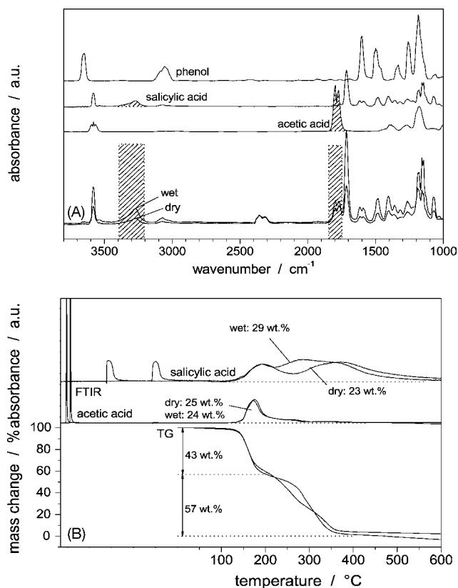
Fig. 10. (A) Extracted spectra recorded during decomposition of aspirin at approximately 260^\circ\text{C} under wet (thick line) and dry conditions. The window of the characteristic wavelength is marked and used for further time-resolved traces. (B) Acetic acid and salicylic acid traces recorded during decomposition of 21.5 mg aspirin under wet and dry conditions and calibration pulses injected before decomposition: Injections were done after the TA, immediately before the FTIR-transfer-line.
