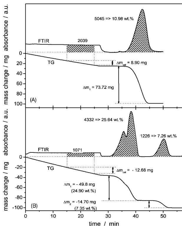
Fig. 9. Differential calibration: water-traces recorded during decomposition of 200 mg \text{NaHCO}_3 (A) and 200 mg \text{CuSO}_4 \cdot 5\text{H}_2\text{O} (B). Heating rate: 10 \text{ K min}^{-1} , carrier gas: 25 \text{ ml min}^{-1} (A), 50 \text{ ml min}^{-1} (B). The mass of water used for the calibration at 50^\circ\text{C} was ca. 25 mg (A) and 35 mg (B). Interval time: 10 min. Crucible diameter: 7.5 mm.
