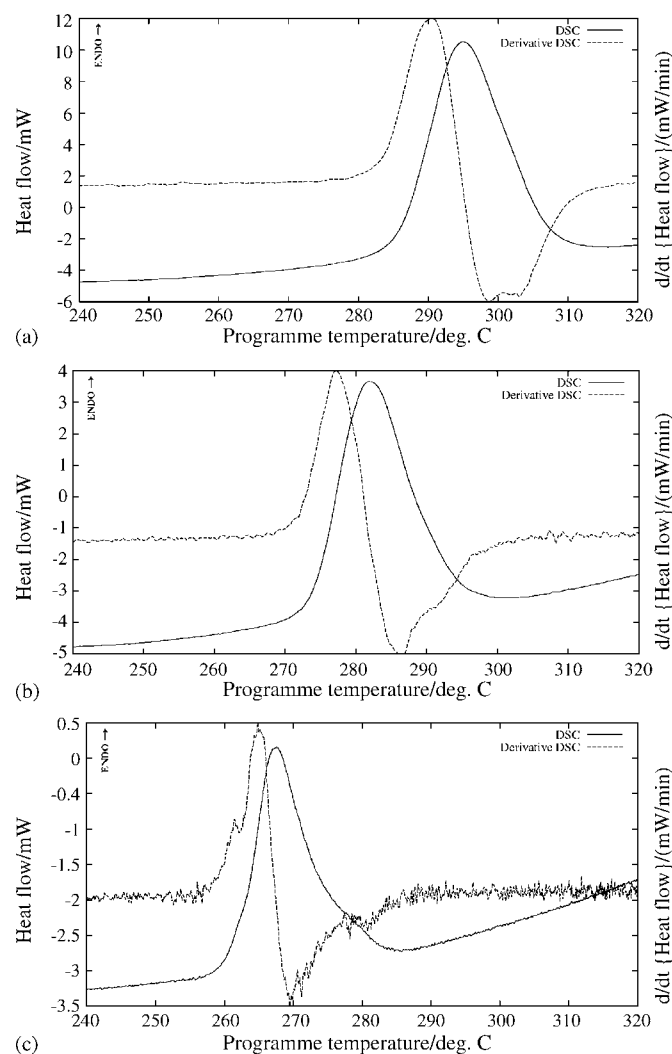
Fig. 8. DSC curves for copper(II) oxalate heated under argon ( 25 \text{ mL min}^{-1} ) from 25 to 360^\circ\text{C} at: (a) 10^\circ\text{C min}^{-1} ; (b) 5^\circ\text{C min}^{-1} ; (c) 2^\circ\text{C min}^{-1} .
