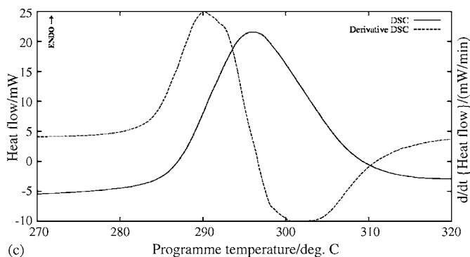
Fig. 10. DSC curves for copper(II) oxalate heated under argon from 25 to 360 °C at 10 °C min -1 at various flow rates: (a) 33 mL min -1 ; (b) 25 mL min -1 ; (c) 17 mL min -1 .
