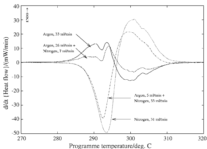
Fig. 7. Derivative DSC curves of copper(II) oxalate (see Fig. 6), heated in crimped aluminium pans, in various mixed argon–nitrogen atmospheres from 25 to 350 °C at 10 °C min -1 . Samples were of similar masses (4 mg). The derivatives were smoothed using a simple 11-point boxcar algorithm.
