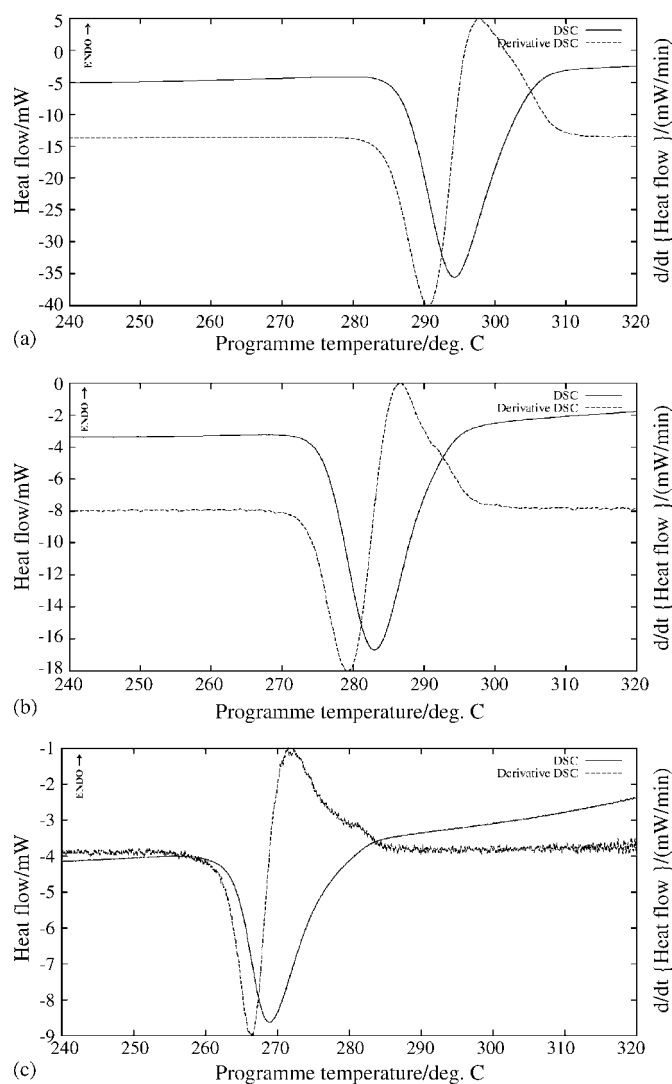
Fig. 9. DSC curves for copper(II) oxalate heated under nitrogen ( 25 \text{ mL min}^{-1} ) from 25 to 360^\circ\text{C} at: (a) 10^\circ\text{C min}^{-1} ; (b) 5^\circ\text{C min}^{-1} ; (c) 2^\circ\text{C min}^{-1} .
