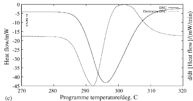
Fig. 11. DSC curves for copper(II) oxalate heated under nitrogen from 25 to 360 °C at 10 °C min -1 at various flow rates: (a) 30 mL min -1 ; (b) 24 mL min -1 ; (c) 15 mL min -1 .
