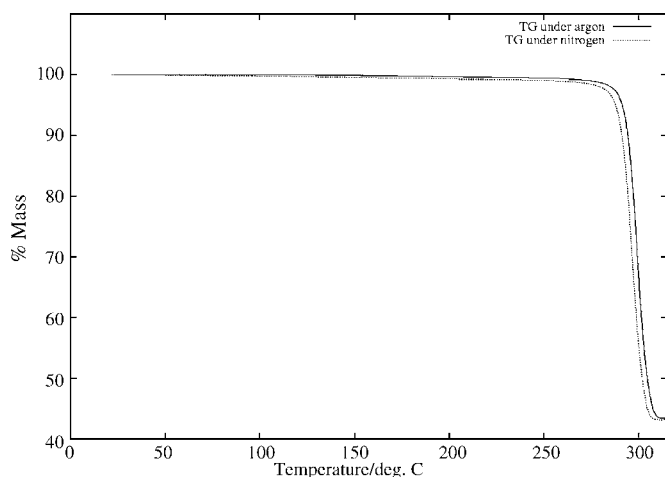
Fig. 2. The TG curves for copper(II) oxalate heated from 25 to 315 °C at 10 °C min -1 under argon and nitrogen atmospheres.
