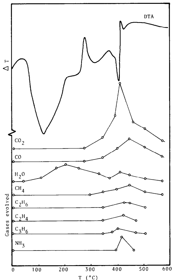
Fig. 4. Thermal and chromatographic behaviour of Na 4 -PDTA.
