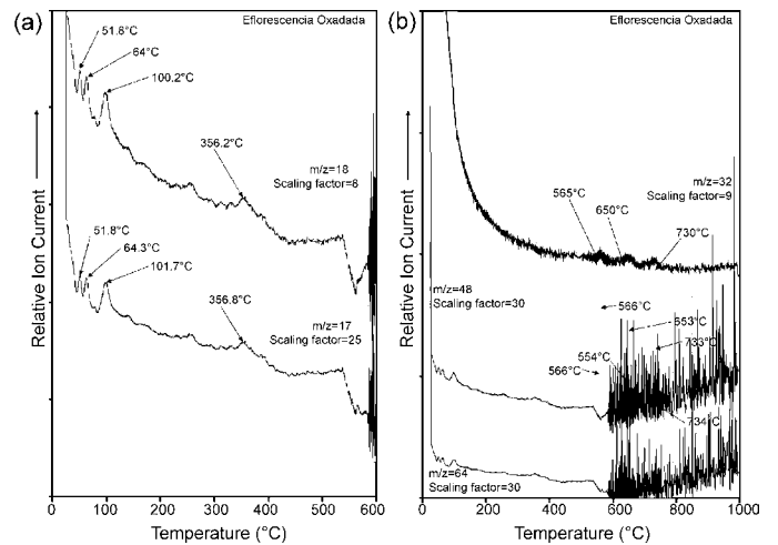
Fig. 5. Ion current curves for (a) m/z = 17 and 18, and (b) m/z = 32, 48 and 64 for the thermal decomposition of the eflorescencia oxadada sample from the El Jaroso Ravine, Spain.
