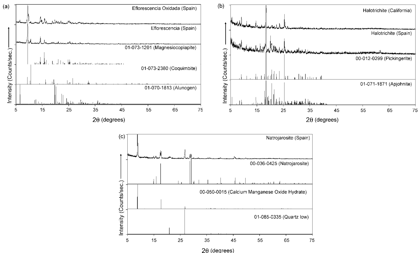
Fig. 1. X-ray diffraction patterns of the (a) evaporite minerals samples from the El Jaroso Ravine, Spain together with possible mineral components, (b) halotrichites from California and Spain together with known standards and (c) jarosite from Spain together with known standards.
