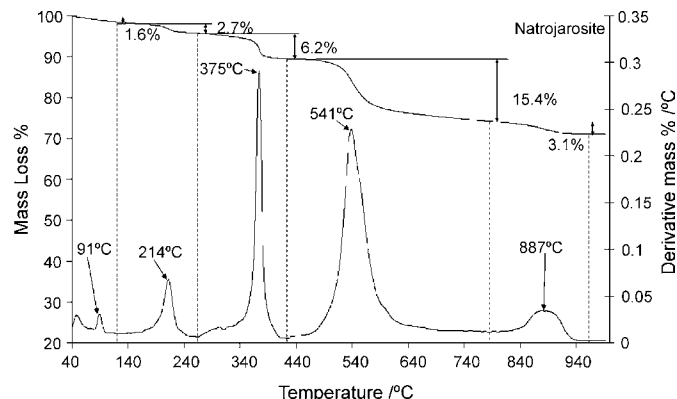
Fig. 6. TG and DTG patterns of Na-jarosite from the El Jaroso Ravine, Spain.
