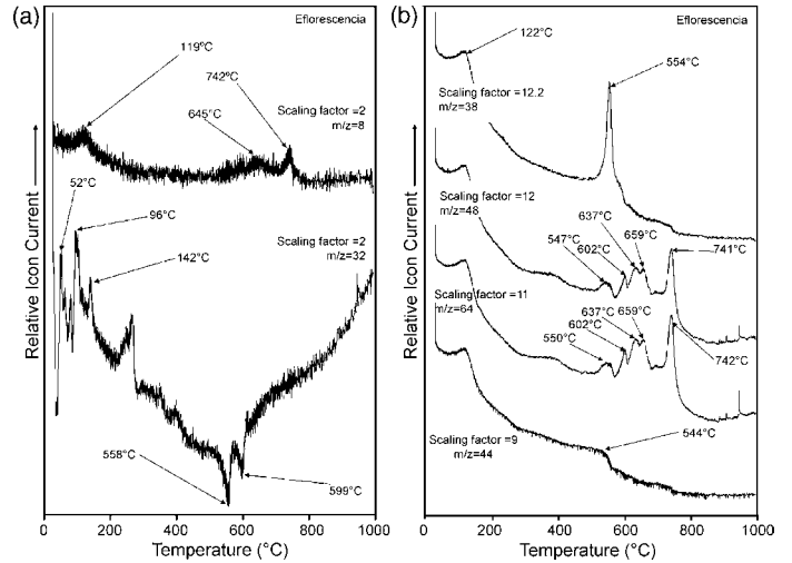
Fig. 3. Ion current curves for (a) m/z = 18 and 32, and (b) m/z = 38, 44, 48 and 64 for the thermal decomposition of the eflorescencia sample from the El Jaroso Ravine, Spain.
