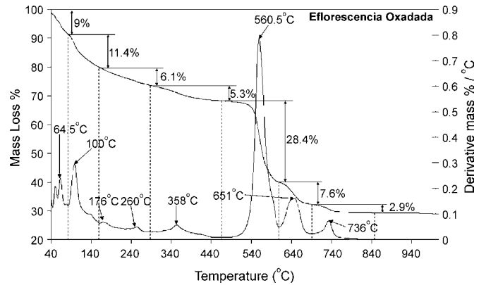
Fig. 4. TG and DTG patterns for the eflorescencia oxadada sample from the El Jaroso Ravine, Spain.
