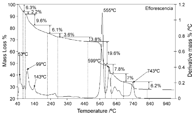
Fig. 2. TG and DTG patterns for the eflorescencia sample from the El Jaroso Ravine, Spain.
