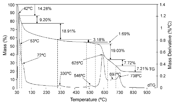
Fig. 7. TG and DTG patterns of a natural halotrichite.
