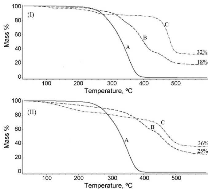
Fig. 10. Comparative TGA profiles of (I) CaAl and (II) MgAl in nitrogen environment at 20 °C/min of pristine: PMMA (A), insoluble PMMA/6%LDH after extraction with acetone and (C) LDH.
