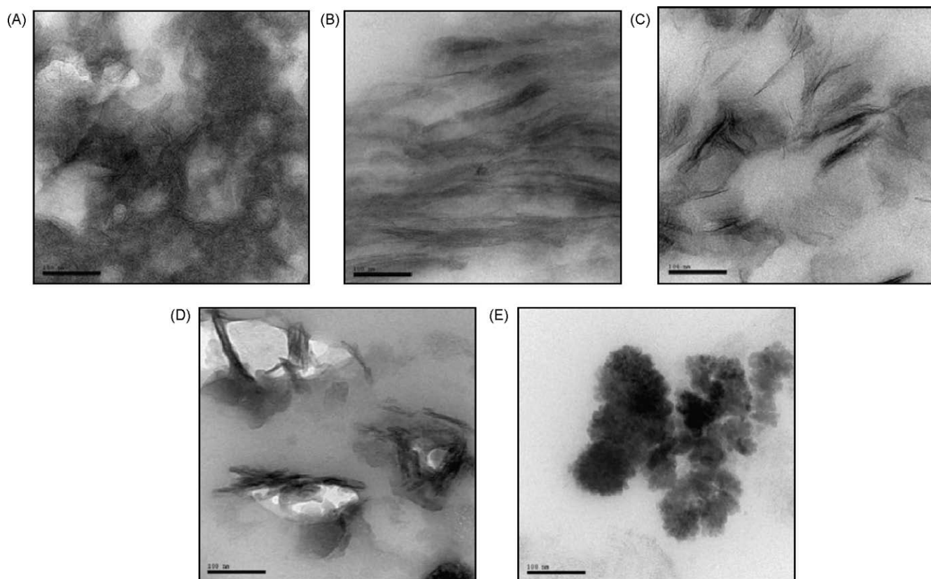
Fig. 8. TEM images of PMMA/LDH systems at high magnification. (A) PMMA/3%NiAl; (B) PMMA/3%MgAl; (C) PMMA/3%CoAl; (D) PMMA/3%CaAl; (E) PMMA/3%CuAl.
