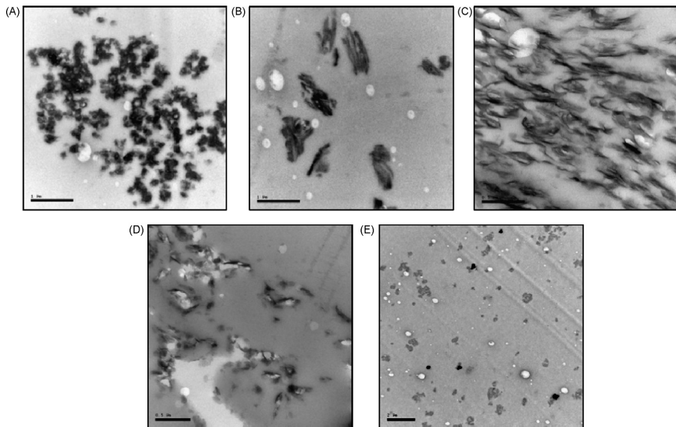
Fig. 7. TEM images of PMMA/LDH systems at low magnification. (A) PMMA/3%NiAl; (B) PMMA/3%MgAl; (C) PMMA/3%CoAl; (D) PMMA/3%CaAl; (E) PMMA/3%CuAl.
