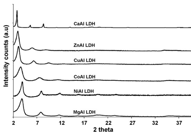
Fig. 1. XRD patterns of the undecenoate-containing LDHs of MgAl, NiAl, CoAl, CuAl and ZnAl.
