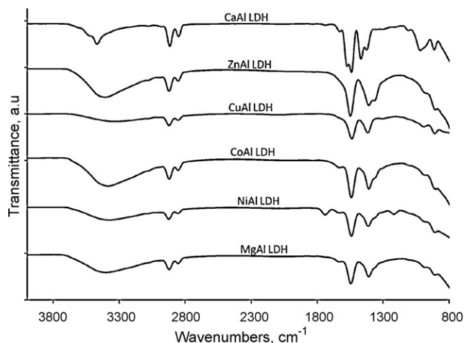
Fig. 2. IR spectra of the undecenoate-containing LDHs of MgAl, NiAl, CoAl, CuAl and ZnAl.
