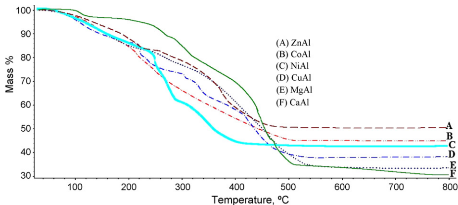
Fig. 4. TGA curves of undecenoate-LDHs in air environment at 20 °C/min from 30 to 800 °C.
