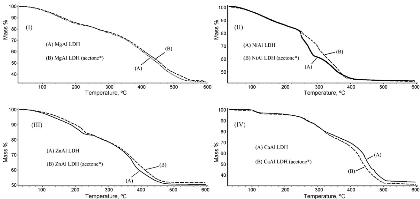
Fig. 5. TGA curves in air of undecenoate-LDHs before and after washing LDHs in a Soxhlet extraction apparatus with acetone for 2 days.
