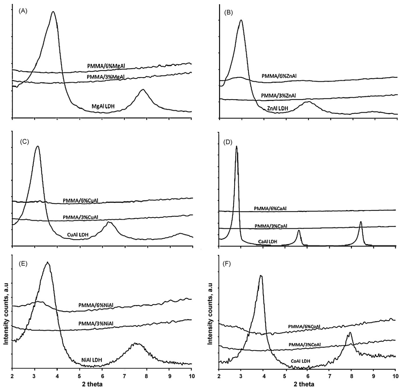
Fig. 6. XRD traces of various PMMA/LDH systems, loadings of 3 and 6%. (A) PMMA/MgAl; (B) PMMA/ZnAl; (C) PMMA/CuAl; (D) PMMA/CaAl; (E) PMMA/NiAl and (F) PMMA/CoAl.
