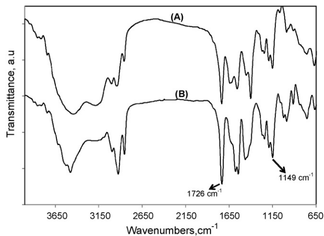
Fig. 11. FT-IR spectra of insoluble materials of (A) PMMA/6%MgAl and (B) PMMA/6%CaAl after extraction with the acetone.
