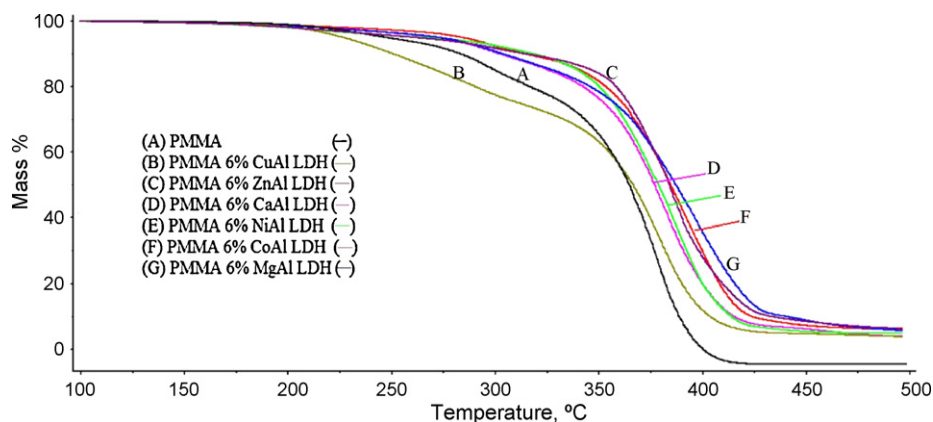
Fig. 9. TGA curves of PMMA and its LDH composites at 6% additive (wt%) loading.
