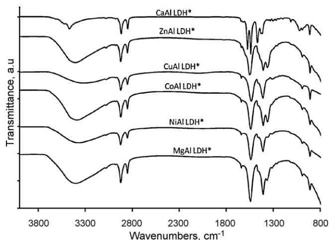
Fig. 3. IR spectra of the undecenoate-containing LDHs (*) (after Soxhlet extraction with acetone for 2 days) of MgAl, NiAl, CoAl, CuAl and ZnAl.
