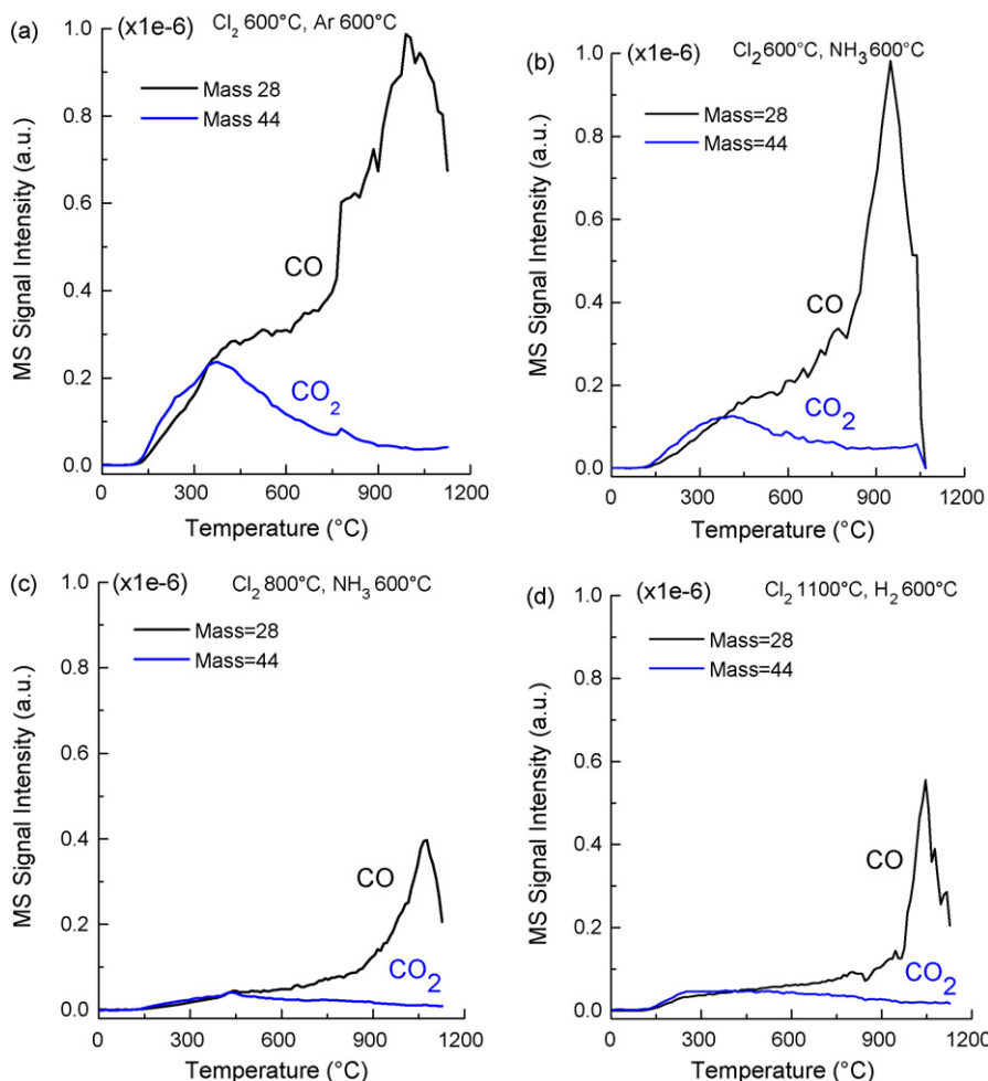
Fig. 7. CO and CO 2 profiles of the 600 °C CDC post-treated under Ar (a) and NH 3 (b) and 800 °C CDC post-treated under NH 3 (c) and 1100 °C CDC post-treated under H 2 (d).
