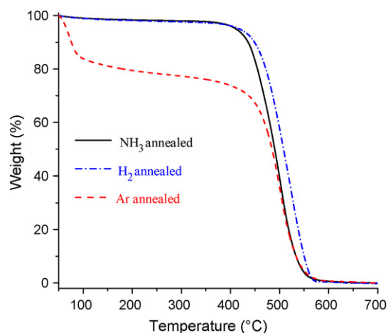
Fig. 4. TGA of CDCs synthesized at 600 °C, annealed in Ar, H 2 and NH 3 . Heating rate 2 °C/min.
