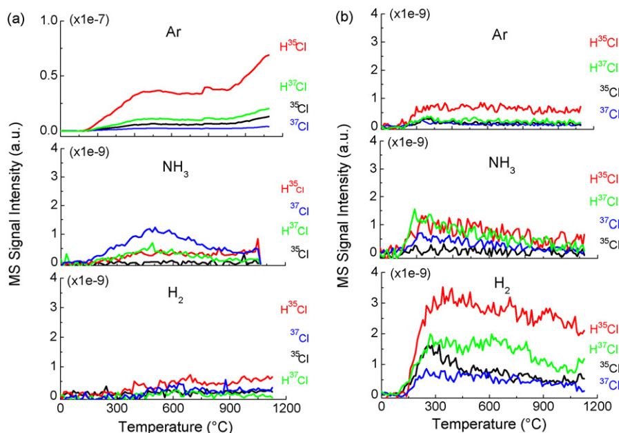
Fig. 5. TPD profiles of HCl and Cl evolved from CDCs chlorinated at 600 °C (a) and 1100 °C (b) and post-treated in Ar, NH 3 and H 2 . Except for the 600 °C CDC annealed in Ar, there is no conservation of ratios characteristic to natural 35 Cl and 37 Cl (3:1) abundance suggesting limited desorption of Cl and HCl (note the difference in scale for Ar-600 °C sample).
