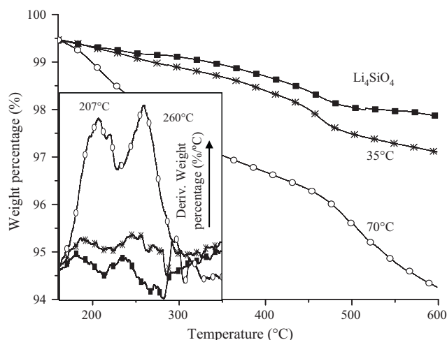
Fig. 5. TGA curves of the \text{Li}_4\text{SiO}_4 samples after humidity treatment: \text{Li}_4\text{SiO}_4 without any thermal treatment, sample previously treated at 35^\circ\text{C} and sample previously treated at 70^\circ\text{C} . The inset shows the derivative curve of thermogravimetric data for the three samples. All the samples were normalized in mass, after the water desorption, at 150^\circ\text{C} .
