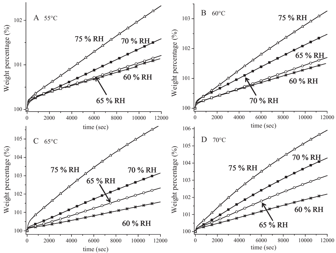
Fig. 7. Isotherms obtained at different RH levels and at different temperatures: (A) 55 °C, (B) 60 °C, (C) 65 °C and (D) 70 °C.
