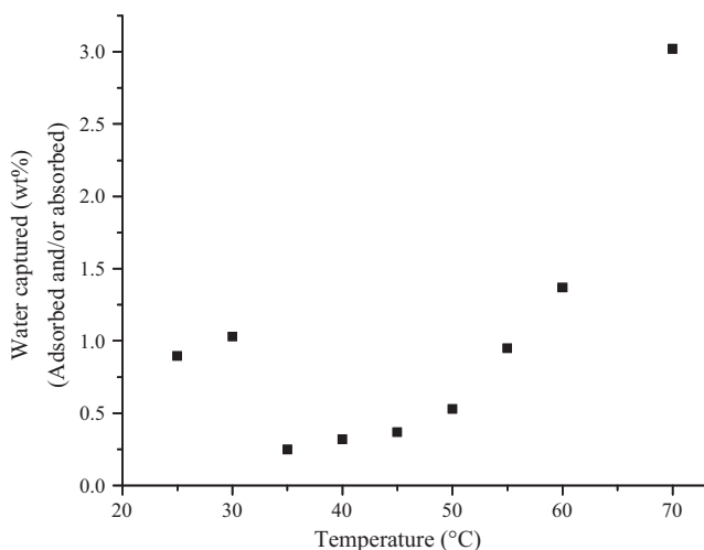
Fig. 3. Total water captured after sorption–desorption cycles at different temperatures.
