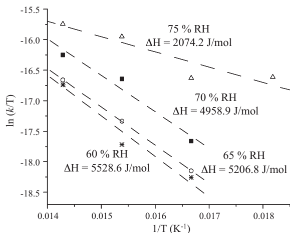
Fig. 9. Eyring's plots for the rate constants ( k ) of water absorption at different RH.
