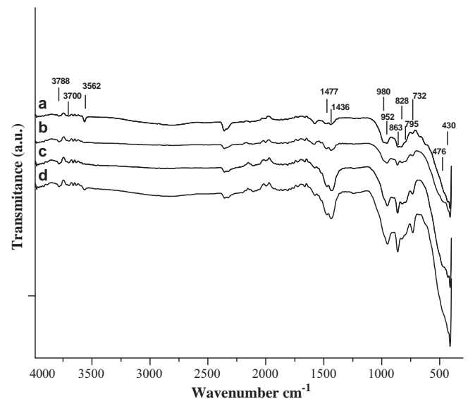
Fig. 4. Infrared spectra of the \text{Li}_4\text{SiO}_4 samples recorded after humidity treatment: (a) \text{Li}_4\text{SiO}_4 without any treatment, (b) heat treated at 35^\circ\text{C} , (c) at 60^\circ\text{C} and (d) and at 70^\circ\text{C} .
