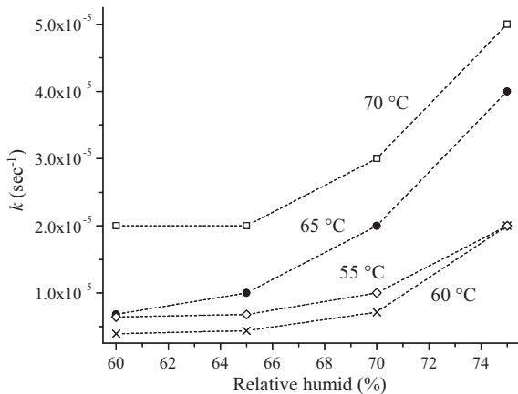
Fig. 8. Rate constants ( k ) calculated from the equation 3 as a function of the RH at different temperatures.
