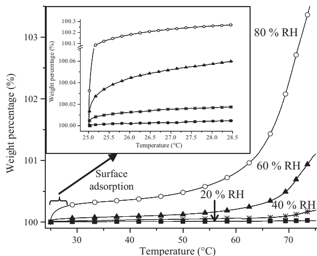
Fig. 6. Water absorbed by \text{Li}_4\text{SiO}_4 particles in a dynamic process at different relative humid (RH) conditions.
