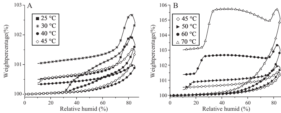
Fig. 2. Water adsorption/desorption isotherms on \text{Li}_4\text{SiO}_4 generated at different temperatures.
