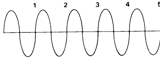
Same Frequency (same pitch) Greater Amplitude (greater volume)
