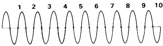
Greater Frequency (higher pitch) Same Amplitude (same volume)
