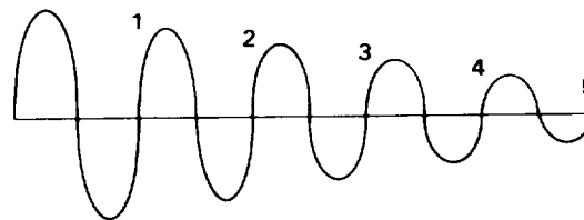
Same Frequency (same pitch) Decreasing Amplitude (decrescendo)
