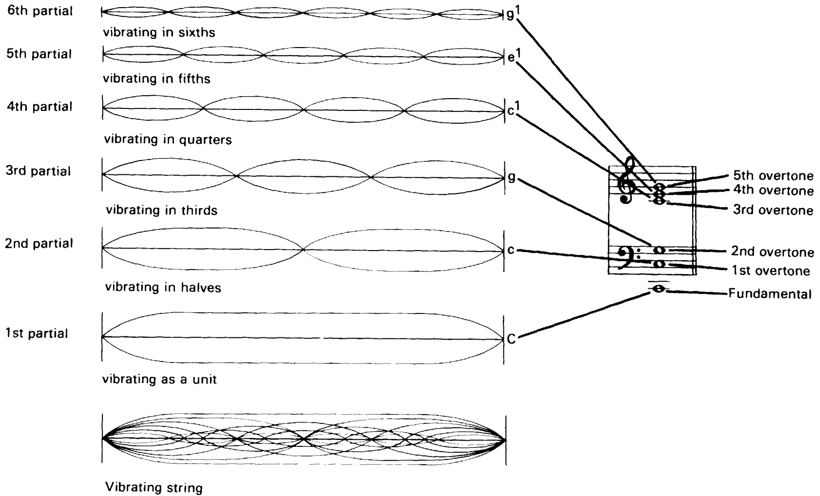
Figure 12.1: Characteristics of a Vibrating String.
