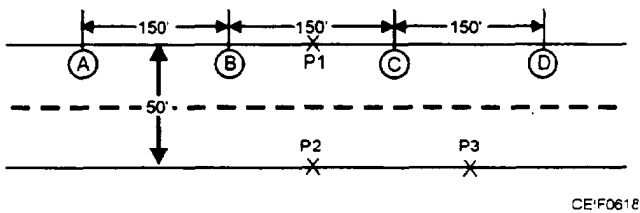
Figure 6-18.—Streetlight layout.
