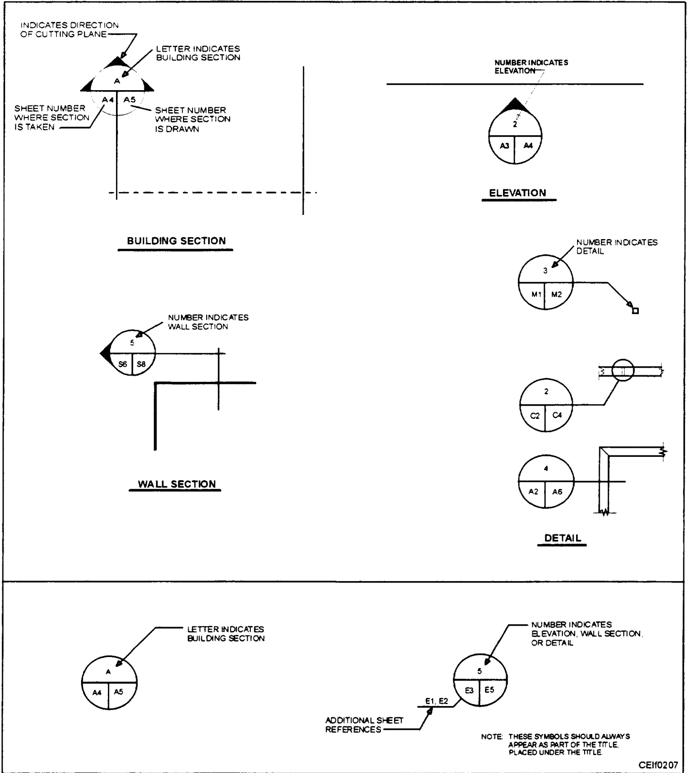
Figure 2-7.—Title symbols.
