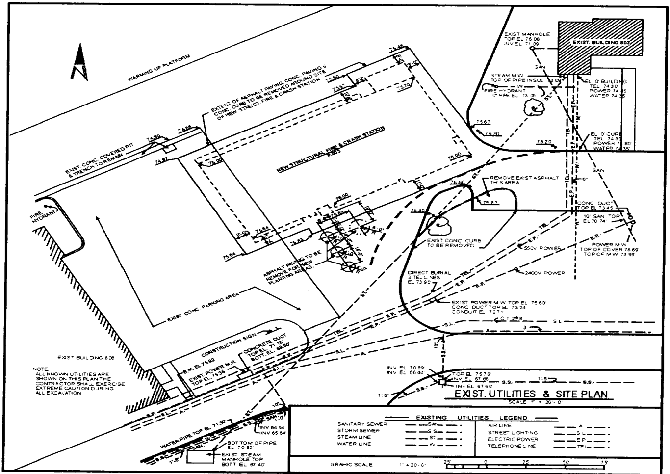
Figure 2-9.—Plot plan, contours, and symbols.
