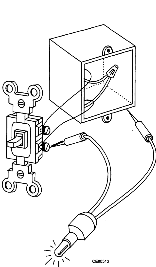
Figure 5-13.—Checking a switch in the ON position for proper operation.
