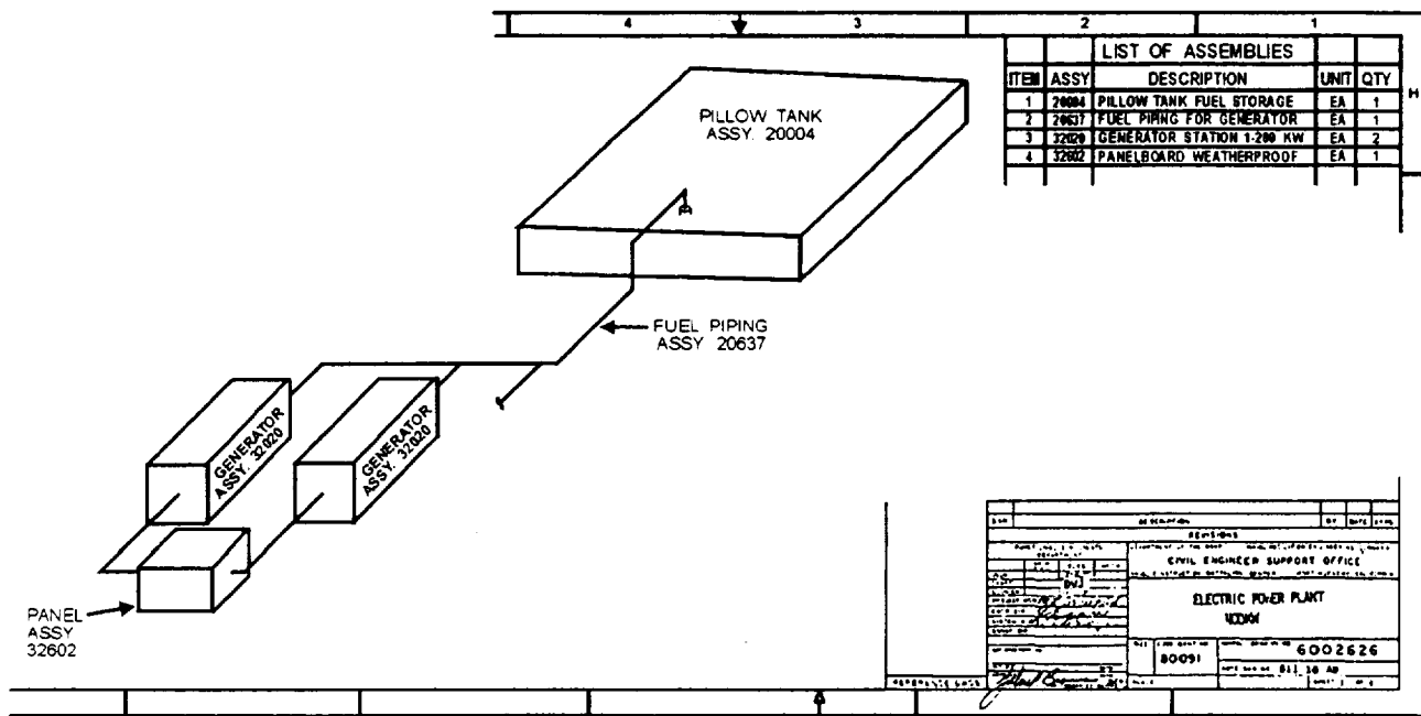
Figure 1-10.—Layout drawing for a 400-kilowatt electrical power plant.
