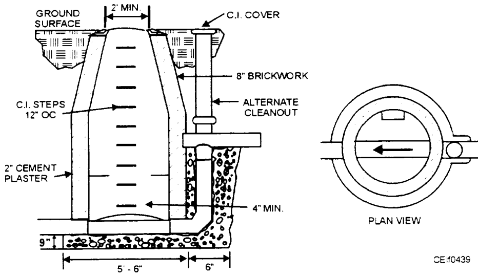
Figure 4-39.—Typical manholes.
