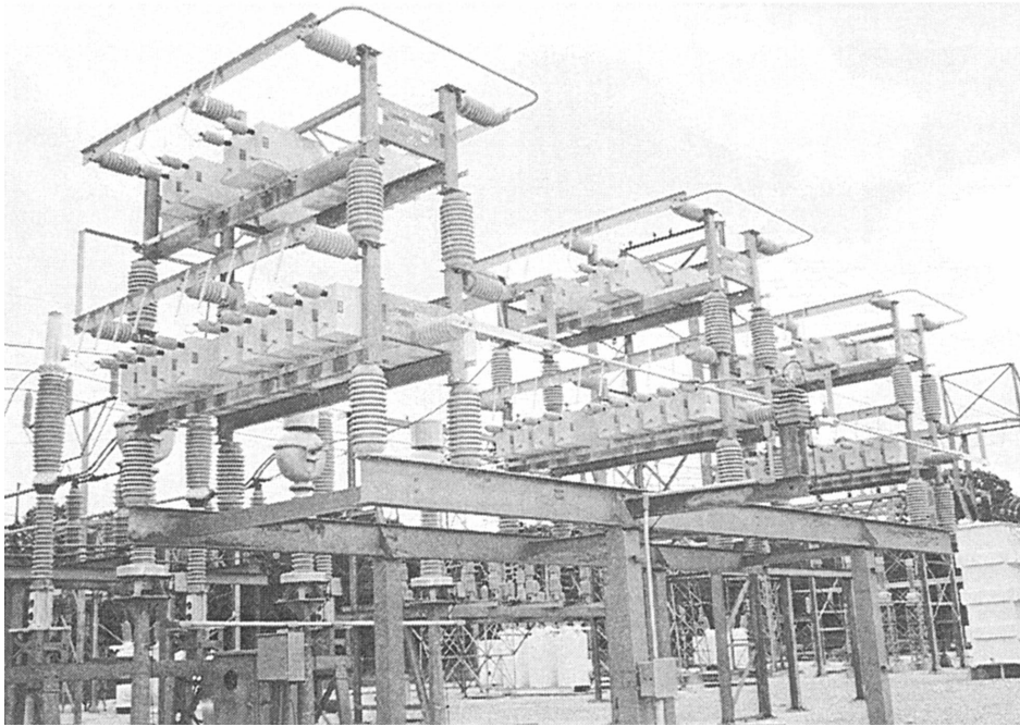
Figure 4-29.—Capacitors, open-rack installation.
