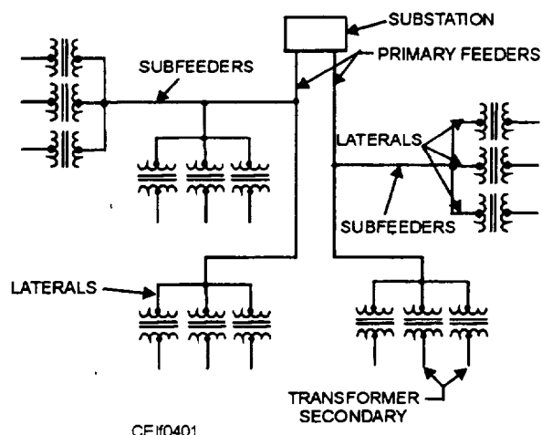
Figure 4-1.—Radial distribution system.
