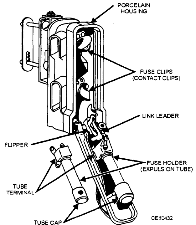
Figure 4-32.—Enclosed primary cutout assembly.
