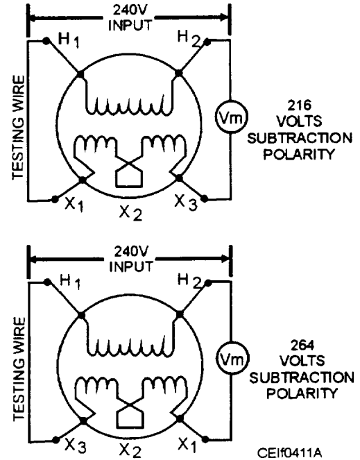
Figure 4-11.—Polarity tests.
