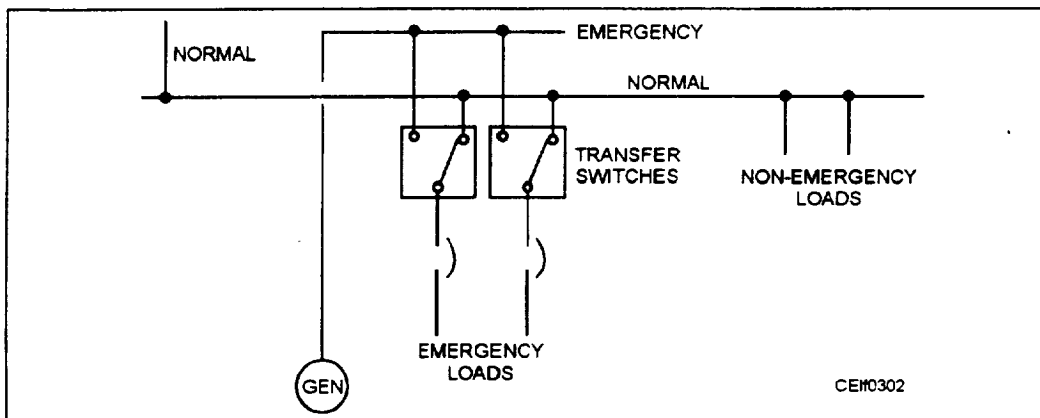
Figure 3-2.—Multiple-transfer switches.
