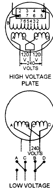
Figure 4-19.—Shows connections for 120/240-volt three-wire, 240-volt three-wire, and 120-volt two-wire services.
