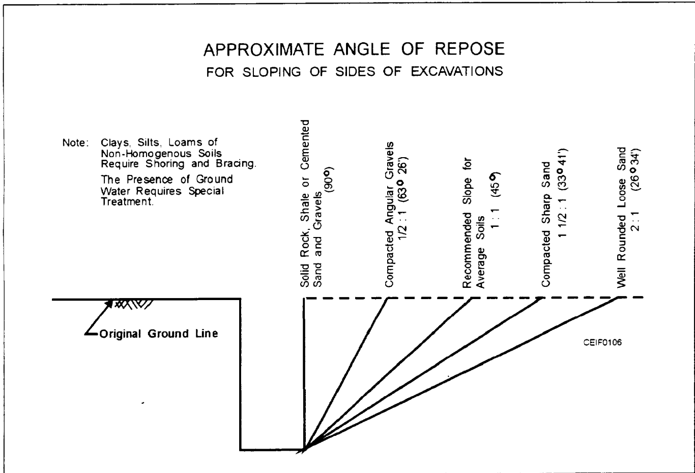
Figure 1-6.—Approximate angle of repose.
