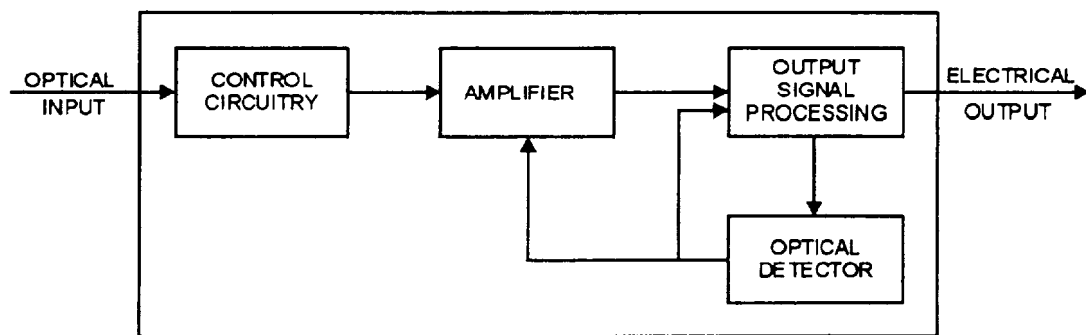
Figure 6-2.—Block diagram of a typical fiber-optic receiver.
