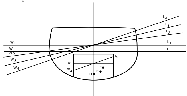
Figure 12-28. Effects of free surface.
