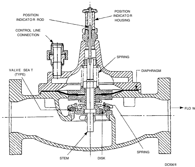
Figure 6-11. Hycheck valve.
