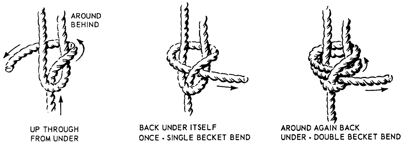
Figure 3-13.--Tying single and double becket bends.
