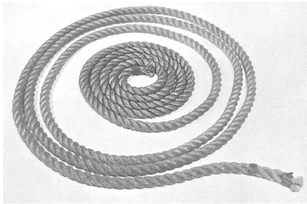
Figure 3-5.—Partially finished line.
