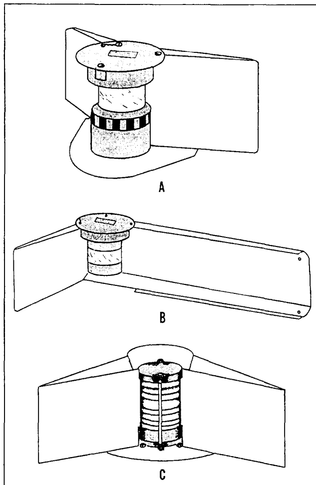
Figure 2-16.— Running lights.
