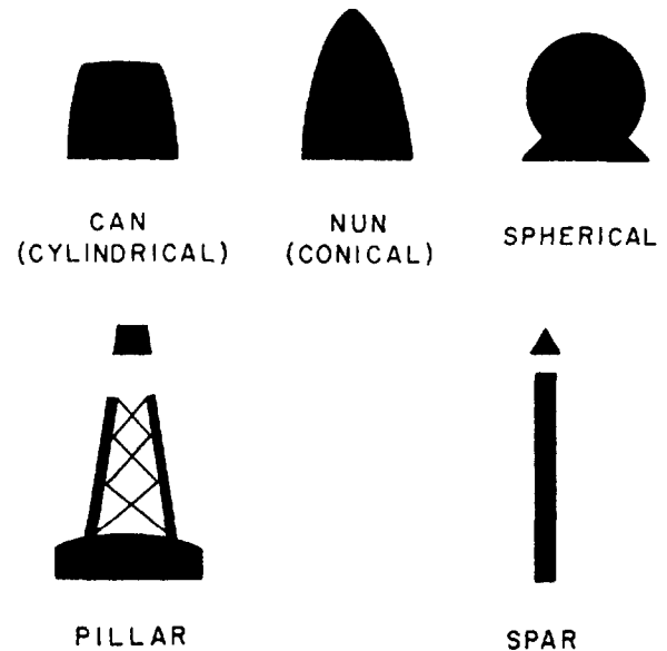
Figure 5-20.—Basic buoy shapes.
