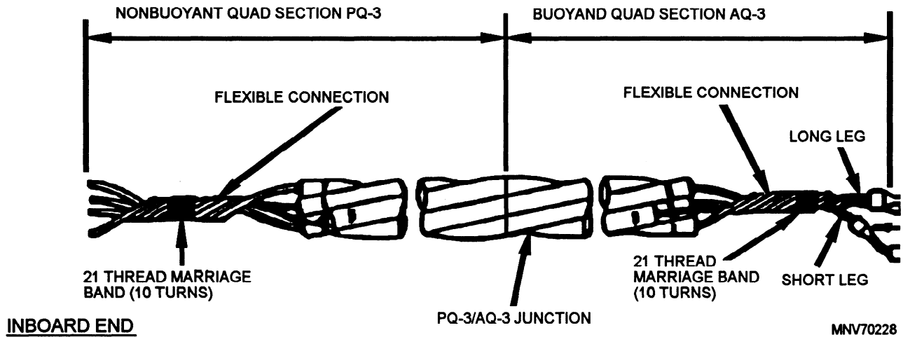
Figure 10-2.—Q-3 cable.
