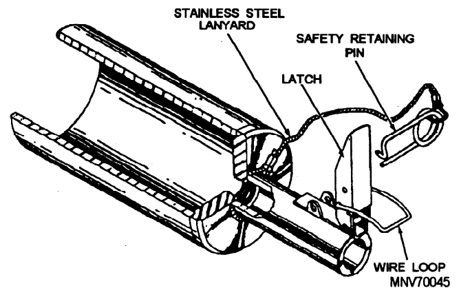
Figure 2-32.—Launcher.
