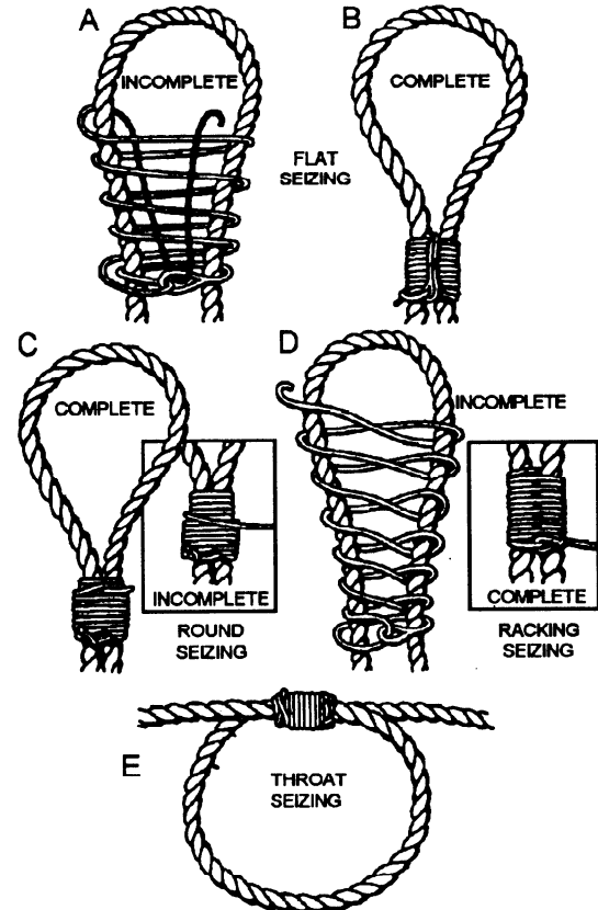
Figure 4-25.—Seizings.
