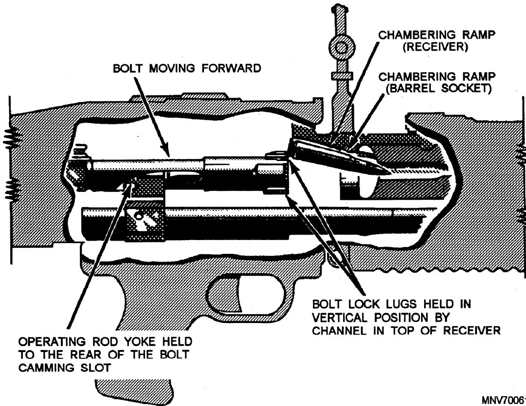
Figure 2-48.—Chambering.
