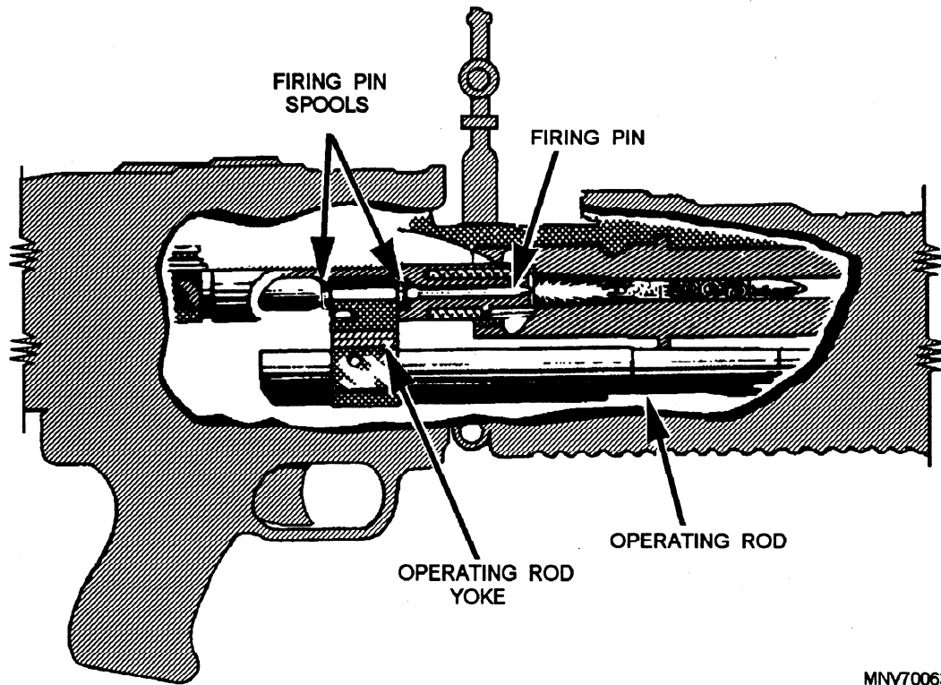
Figure 2-50.—Firing.
