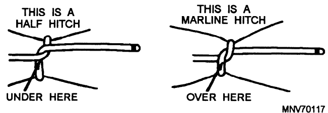
Figure 4-21.—Difference between a marline hitch and a half hitch. MNV70117
