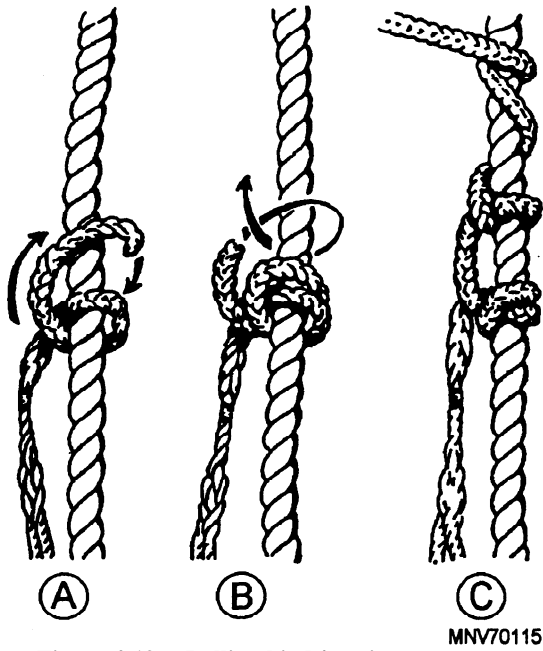
Figure 4-19.—Rolling hitch/passing a stopper. MNV70115
