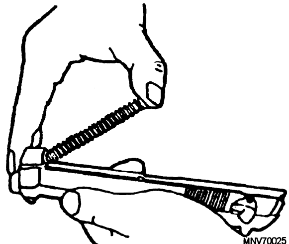
Figure 2-12.—Removing the recoil spring and spring guide.
