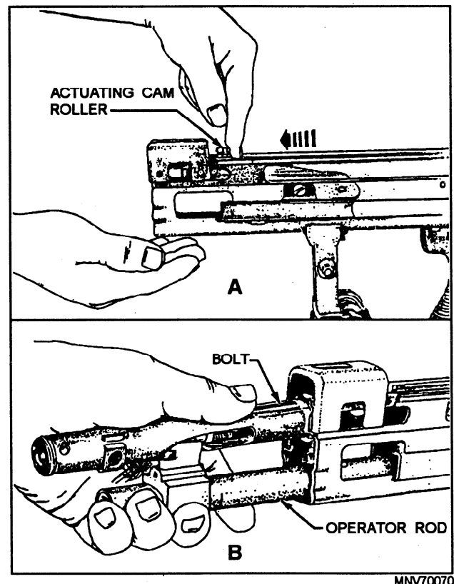
Figure 2-57.—Removing the operating group.
