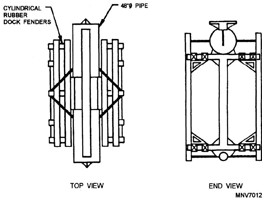
Figure 5-3.—Camels.
