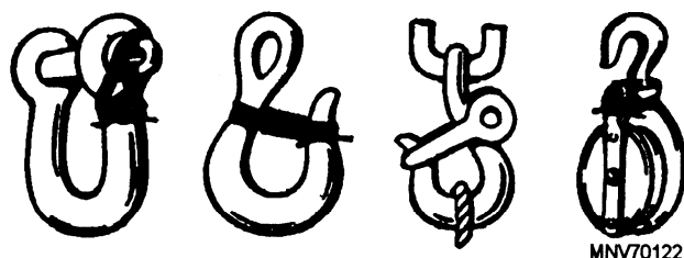
Figure 4-26.—Methods of mousing.
