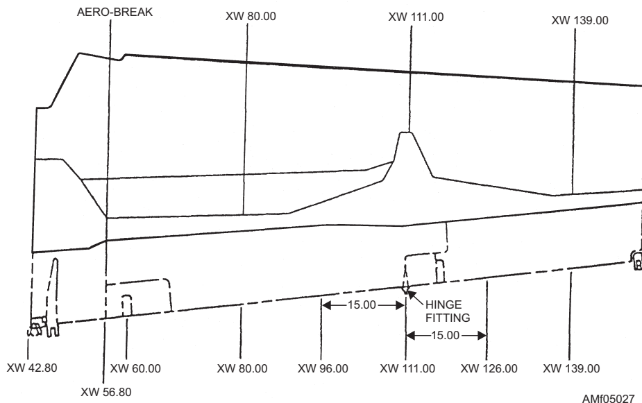
Figure 5-27.—Repair zones.
