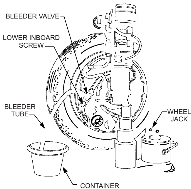
Figure 14-18.—Bleeding brake system (top-down method).
