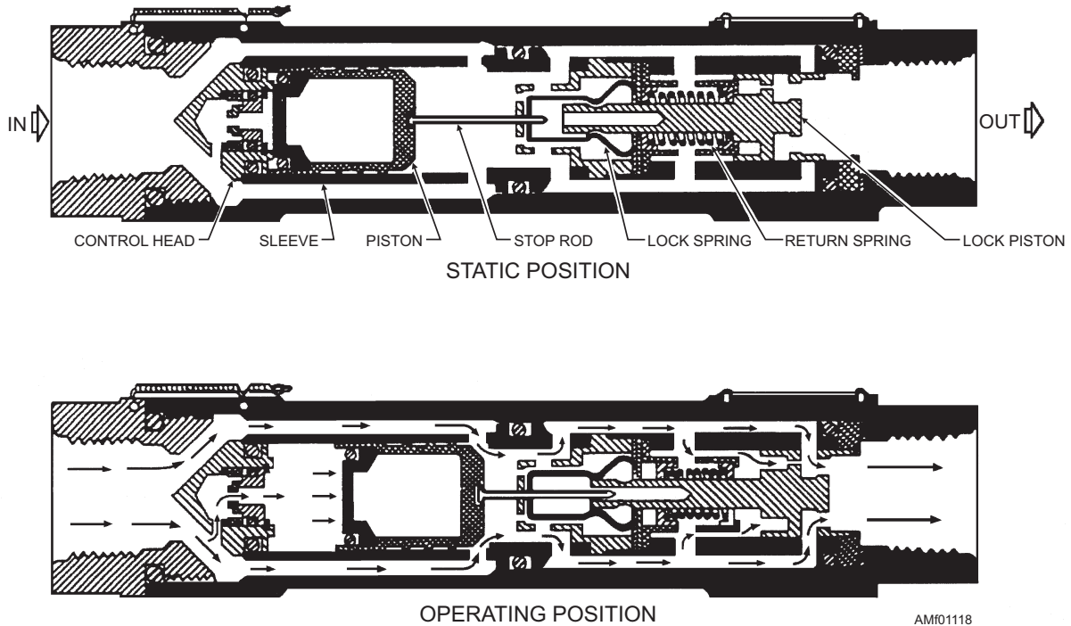
Figure 11-18.—Fuse, operational view.
