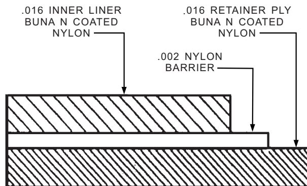
Figure 4-75.—Bladder cell construction.
