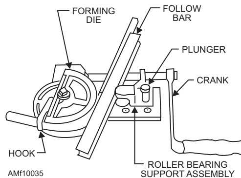
Figure 10-35.—Mechanically operated tube bender.
