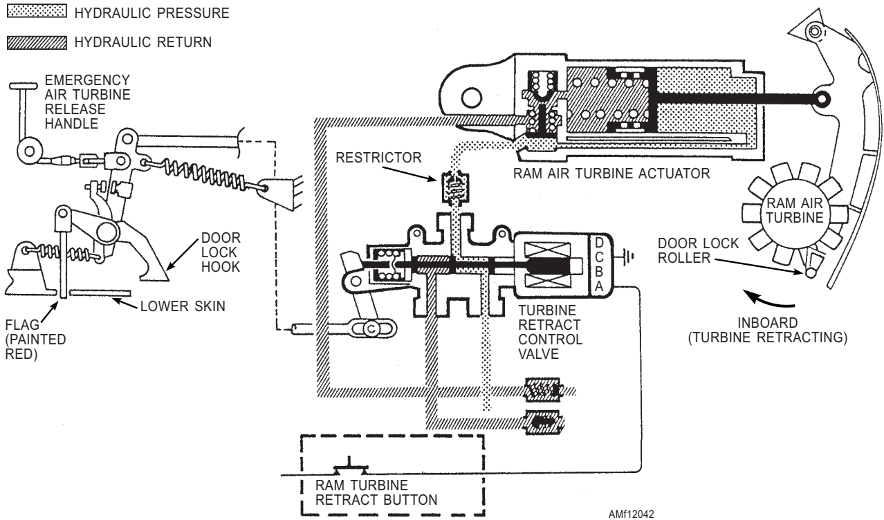
Figure 12-42.—Ram air turbine-control system schematic.
