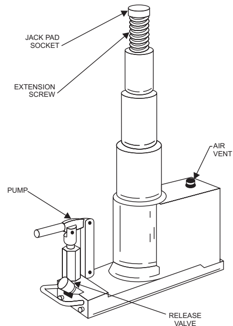
Figure 1-26.—Hand carried axle jack.
