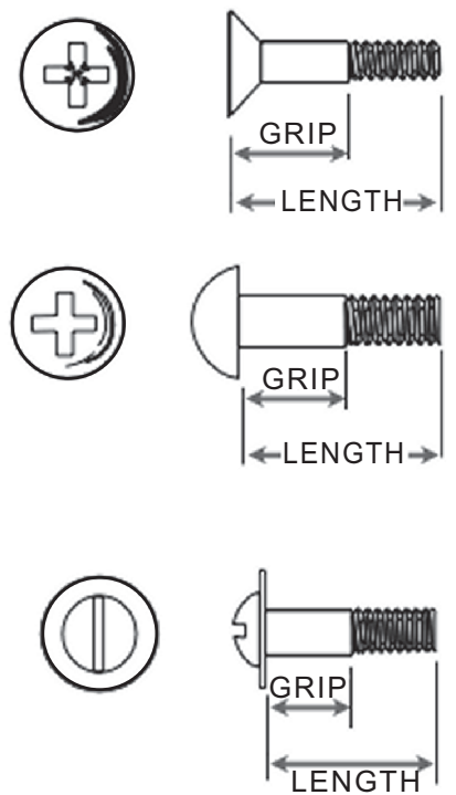
Figure 3-21.—Structural screws.
