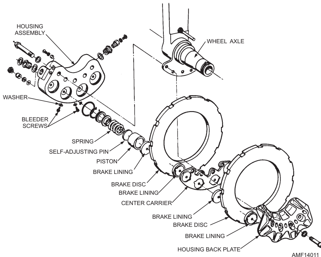
Figure 14-11.—Dual disc brake.
