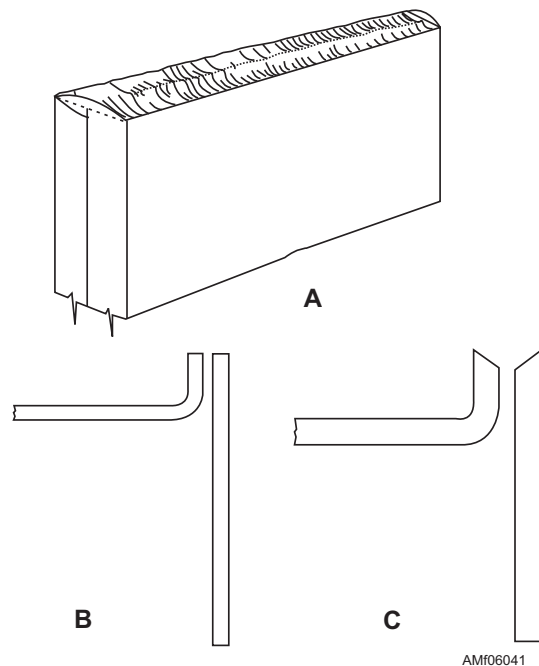
Figure 6-41.—Edge joints for light sheets and plates.
