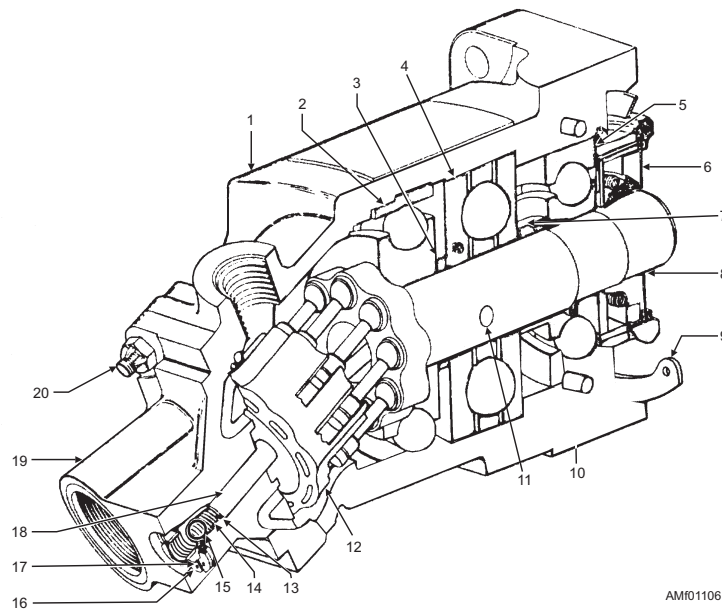
Figure 11-6.—Typical hydraulic motor.
