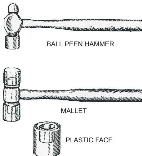
Figure 4-1.—Hammers.
