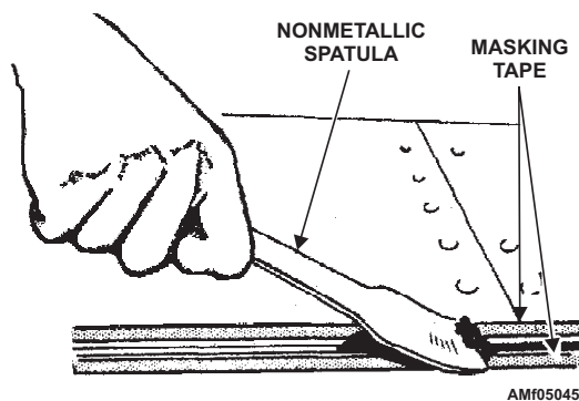
Figure 5-45.—Applying sealant.
