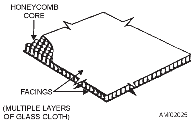
Figure 2-25.—Reinforced plastic.
