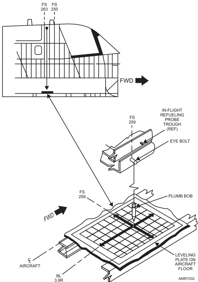
Figure 1-32.—Aircraft leveling.
