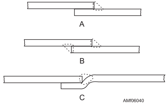
Figure 6-40.—Lap joints.
