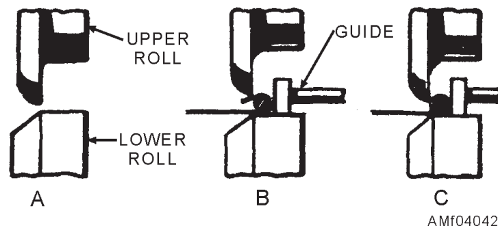
Figure 4-42.—Wiring operation.
