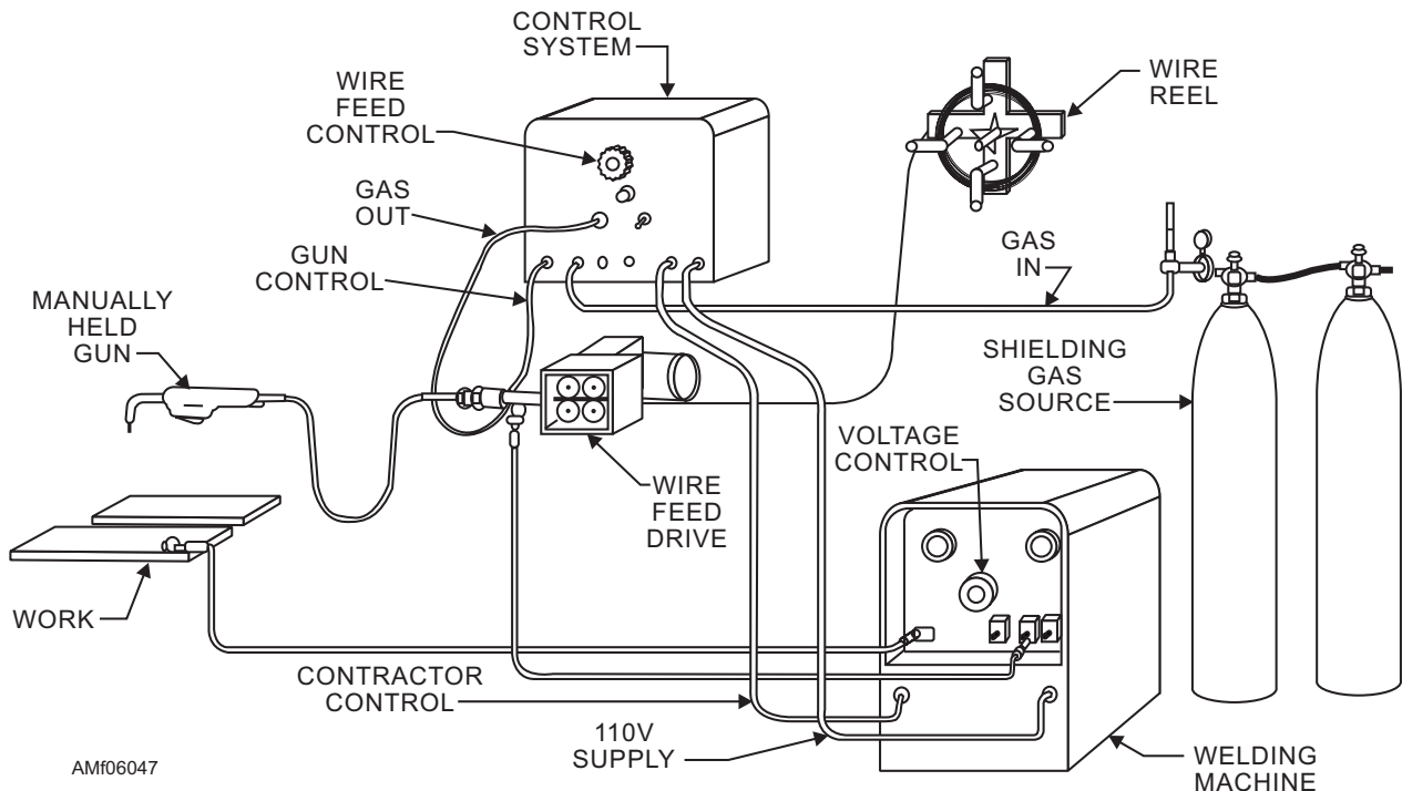
Figure 6-47.—GMA welding equipment.
