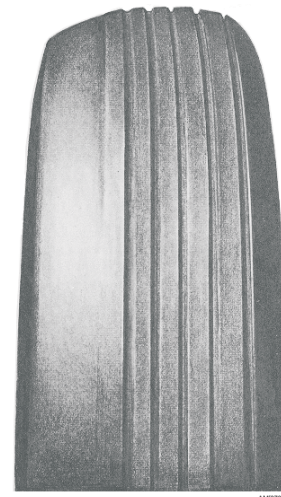
Figure 7-28.—Rapid tread wear caused by misalignment.
