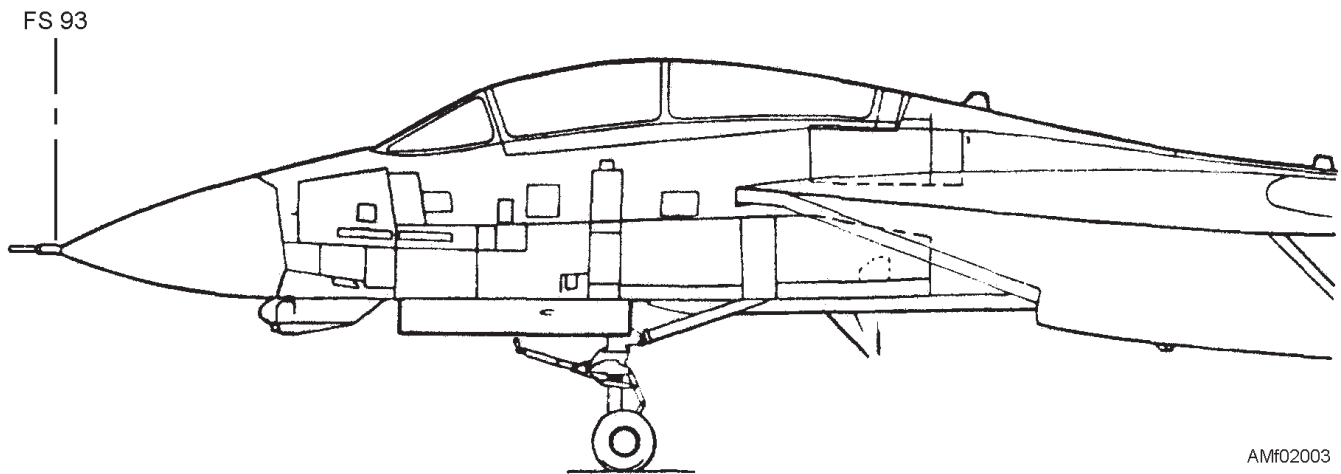
Figure 2-3.—Typical nose station diagram.
