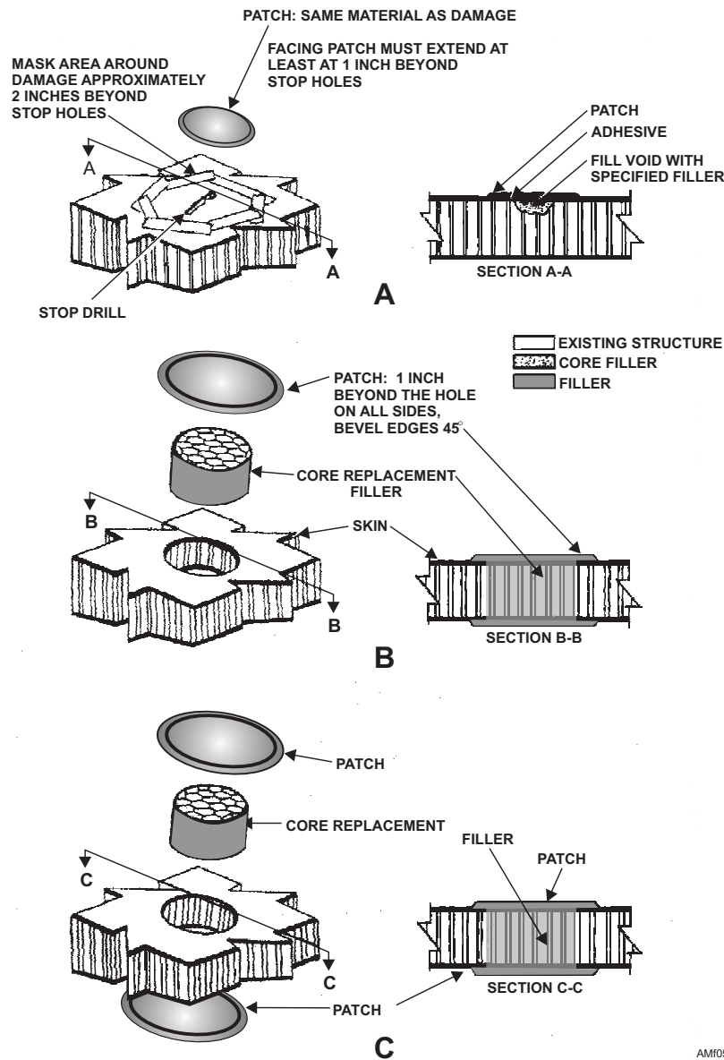
Figure 5-16.—Sandwich construction puncture repair (honeycomb core).
