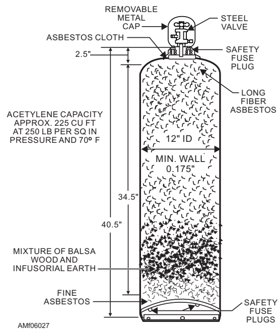
Figure 6-27.—Acetylene cylinder.
