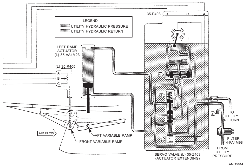
Figure 15-14.—Ramp servo and actuator.
