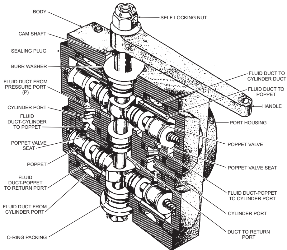
Figure 11-7.—Poppet-type selector valve.
