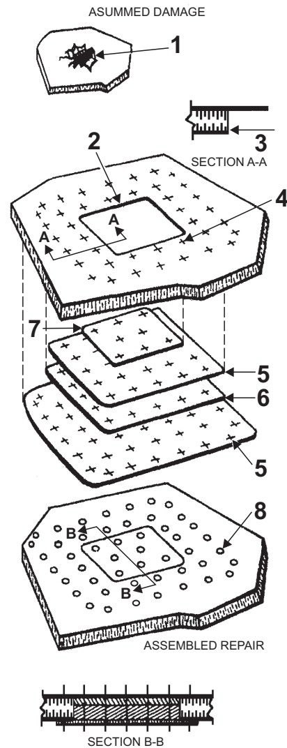
Figure 5-18.—Balsa wood repair with flush patch.
