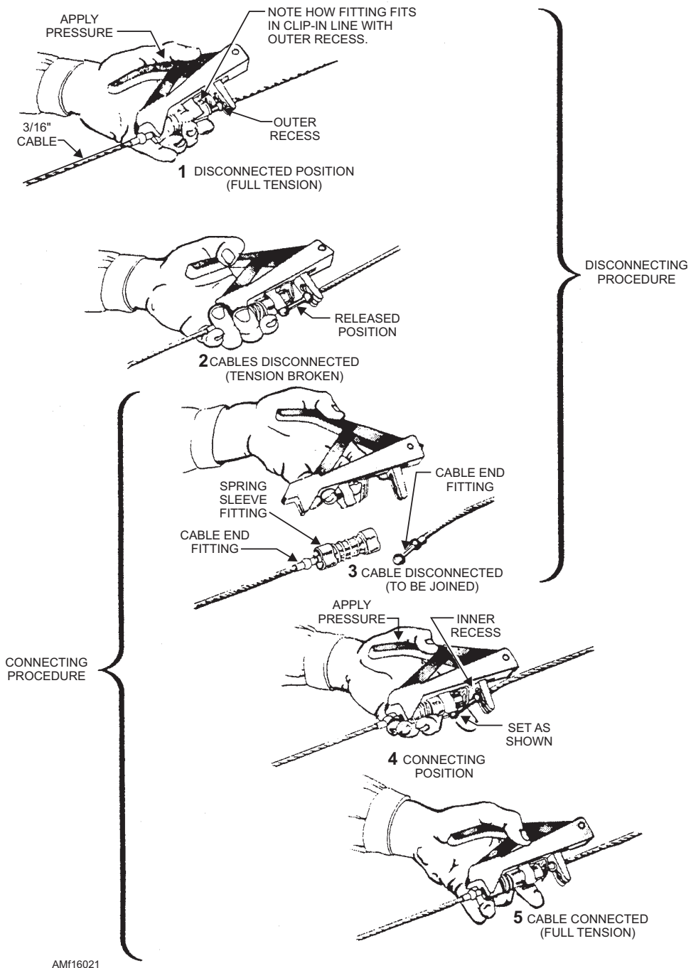
Figure 16-21.—Quick-disconnect procedures.
