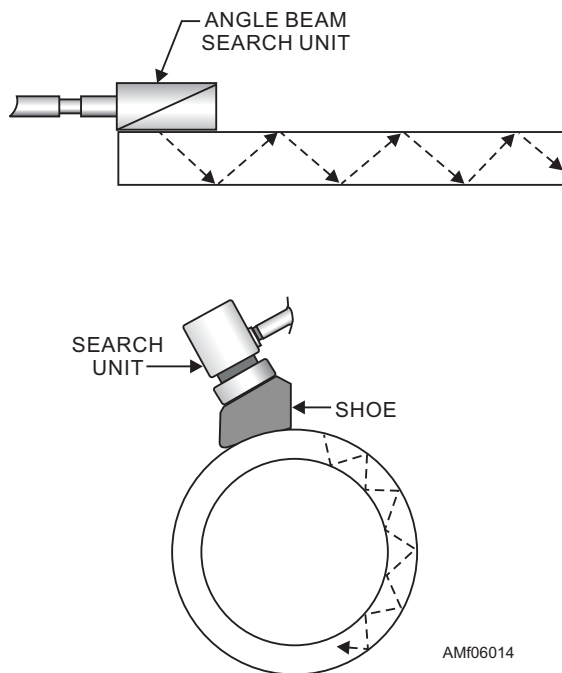
Figure 6-14.—Angle-beam inspection.
