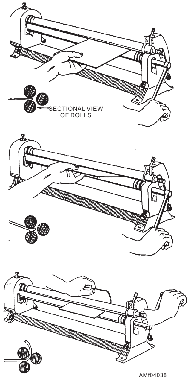
Figure 4-38.—Forming a cylinder.
