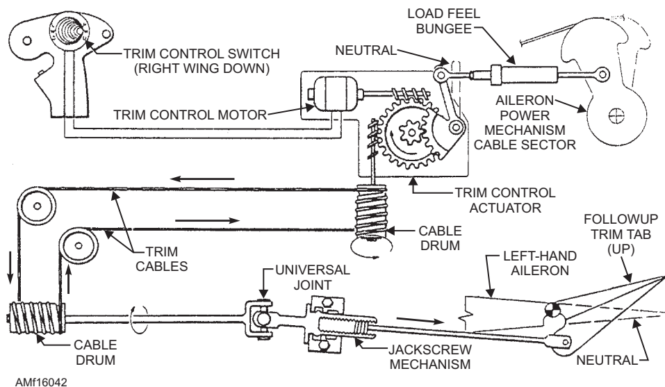
Figure 16-42.—Aileron trim control system.
