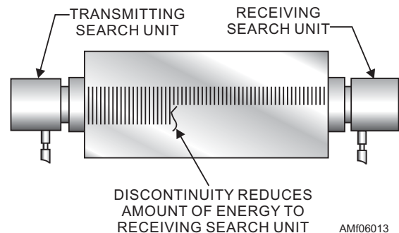
Figure 6-13.—Through-transmission inspection.
