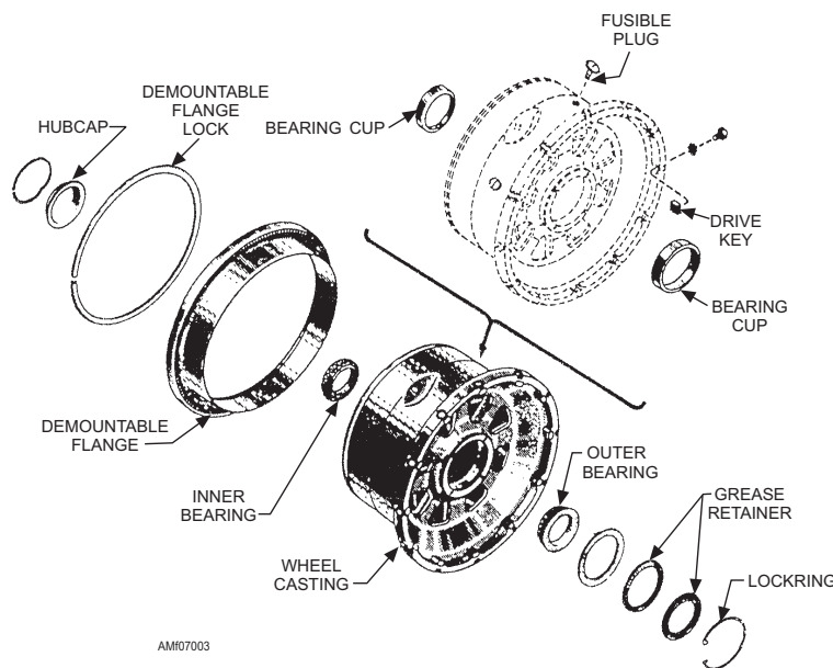
Figure 7-3.—Typical wheel assembly.
