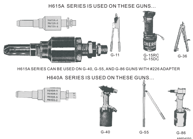
Figure 4-50.—Cherrylock guns.
