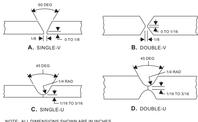
Figure 6-37.—Butt joints in heavy sections.
