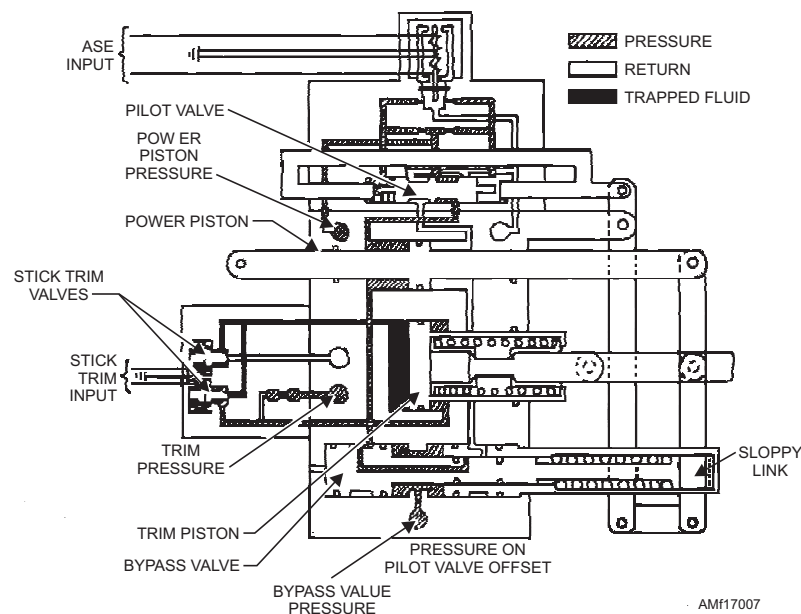
Figure 17-7.—Auxiliary servo cylinder.
