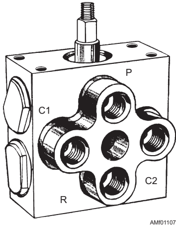
Figure 11-7.—Poppet-type selector valve.
