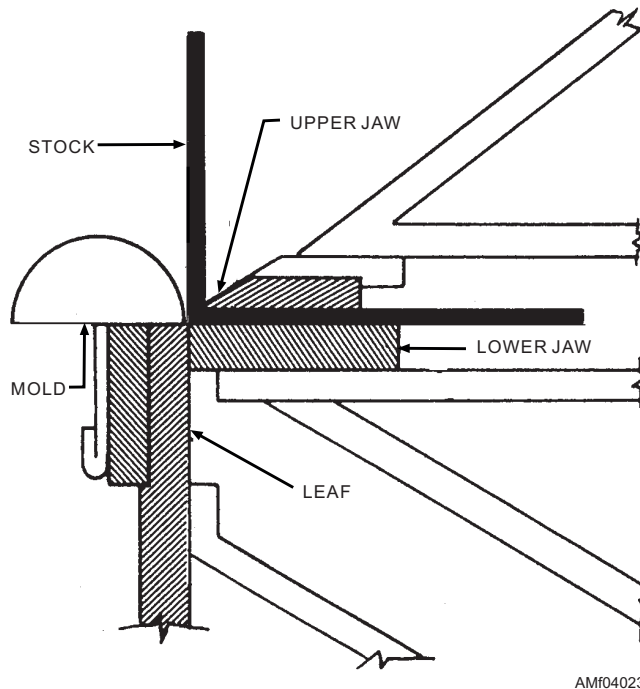
Figure 4-23.—Cornice brake with mold and stock.
