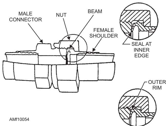
Figure 10-54.—Dynatube fitting.
