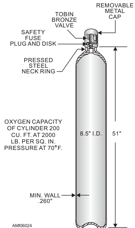
Figure 6-24.—Typical oxygen cylinder.
