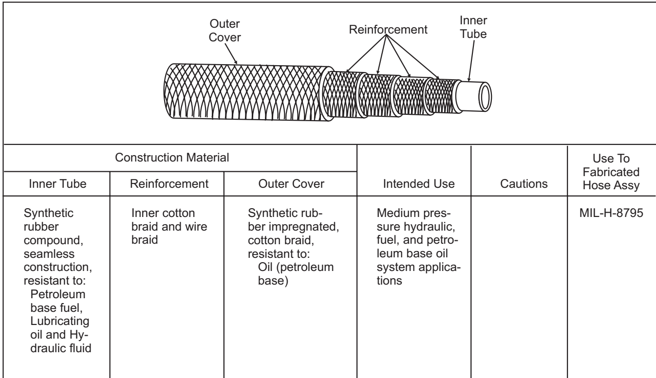
Figure 10-1.—Medium pressure synthetic rubber hose, MIL-H-8794.
