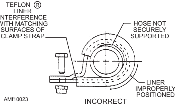
Figure 10-23.—Clamp installation.
