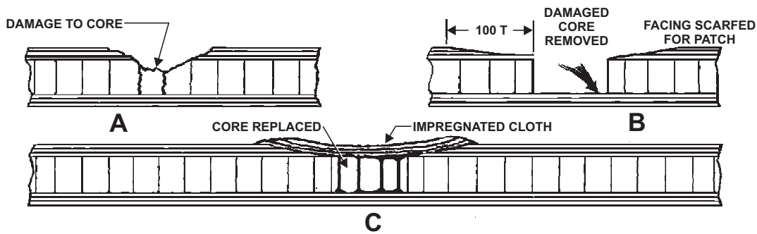
Figure 5-11.—Honeycomb-type core repair.
