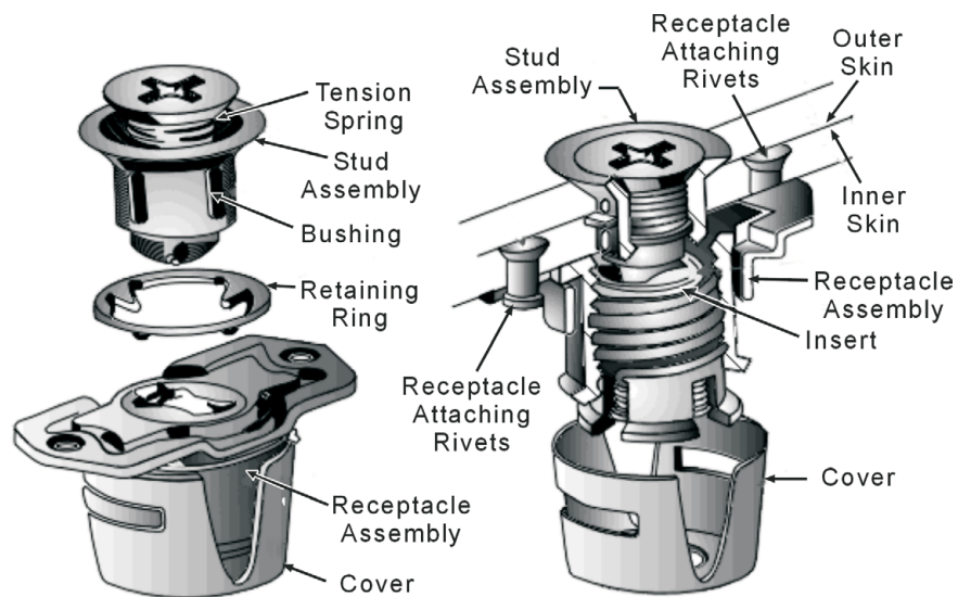
Figure 3-24.—Camloc high-stress panel fastener.
