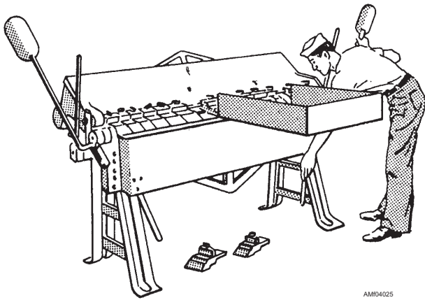
Figure 4-25.—Box and pan brake being used to form box.
