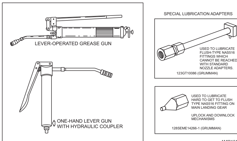
Figure 1-12.—Types of grease guns.
