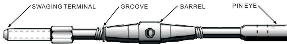
Figure 3-35.—Typical turnbuckle assembly.
