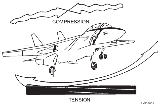
Figure 2-24.—Bending action occurring during carrier landing.
