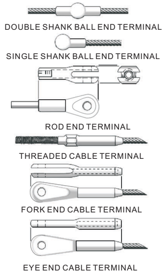
Figure 3-33.—Types of cable terminal fittings.
