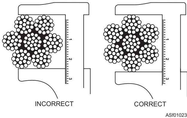
Figure 1-23.—Measuring the diameter of a wire rope.
