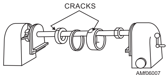
Figure 6-7.—Using a central conductor to circularly magnetize ringlike parts.
