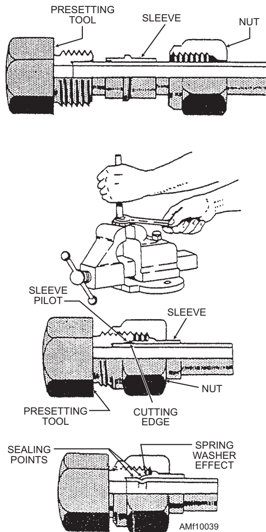
Figure 10-39.—Presetting flareless-tube assembly.
