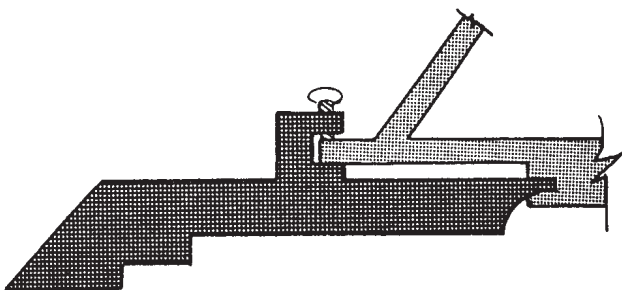
Figure 4-26.—Finger secured in box and pan brake.
