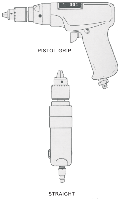
Figure 4-12.—Pneumatic drills.
