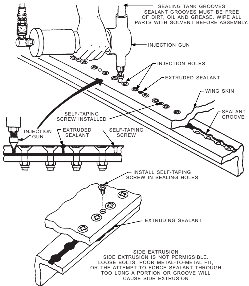
Figure 4-77.—Injection of sealing compound.
