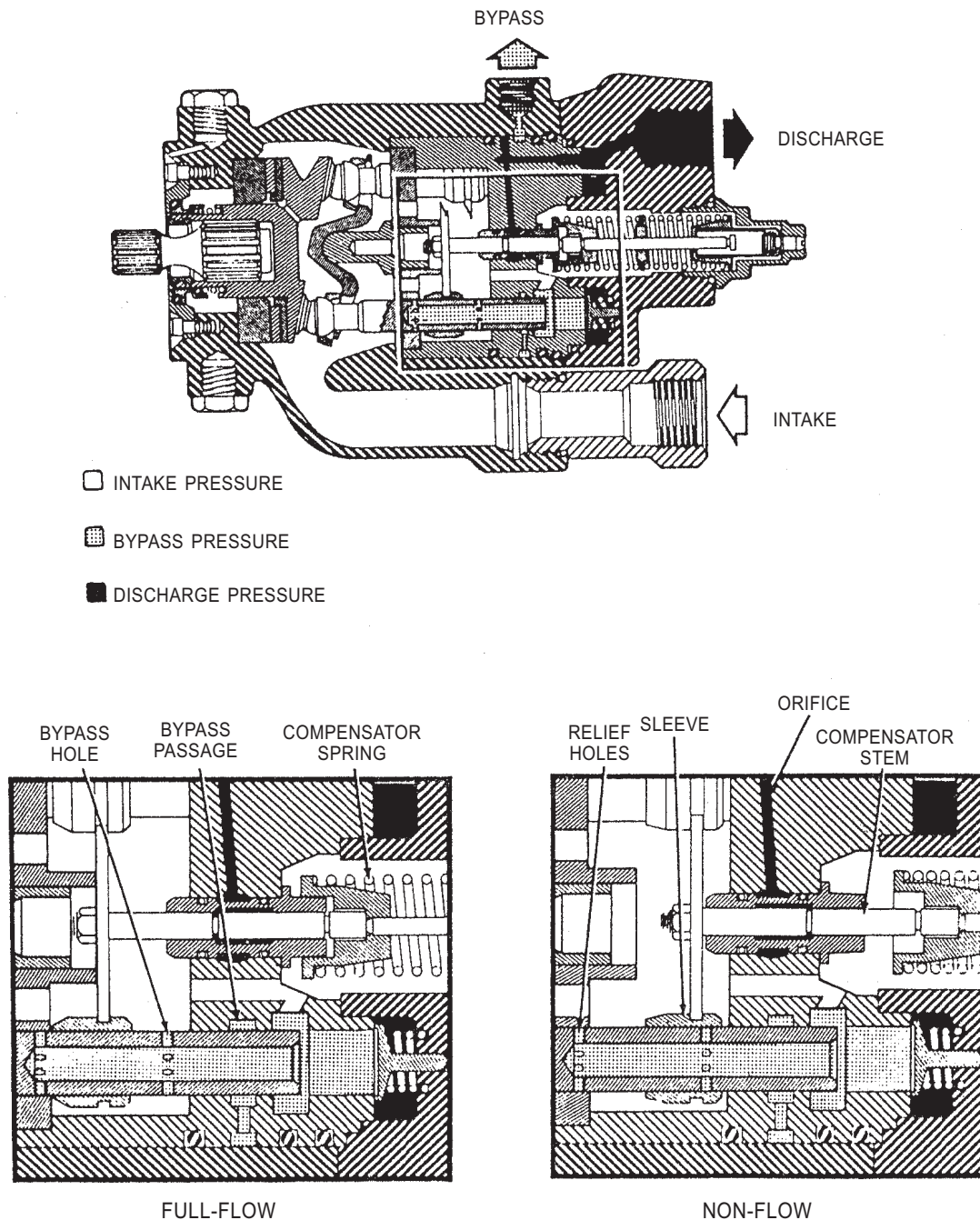
Figure 12-20.—Fluid flow.
