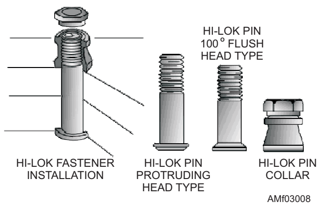
Figure 3-8.—Hi-lok fastener.
