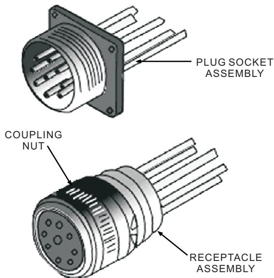
Figure 3-39.—Connector assembly.
