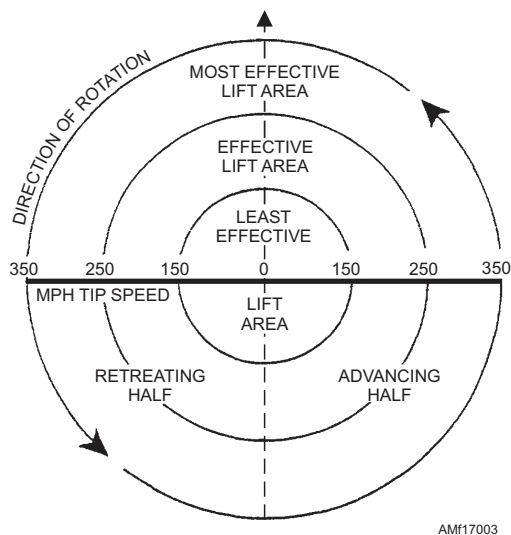
Figure 17-3.—Symmetry of lift.
