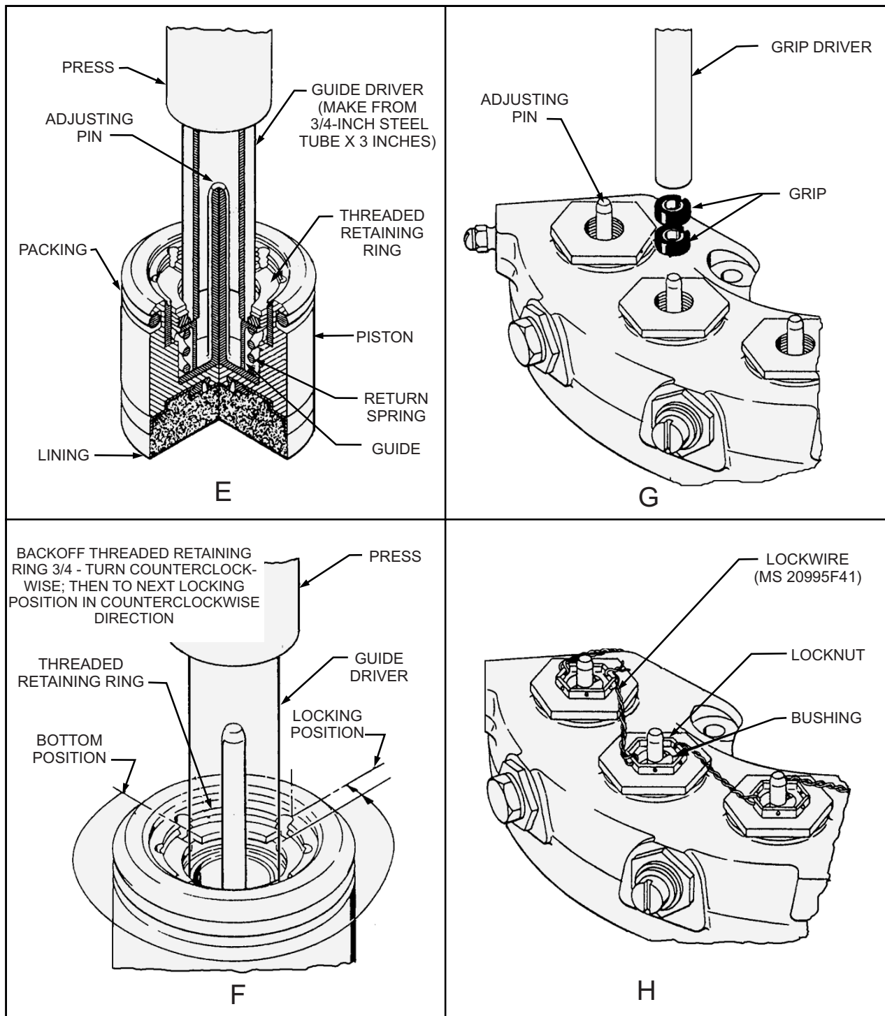
Figure 14-31.—Seal replacement and piston return adjustment—Continued.
