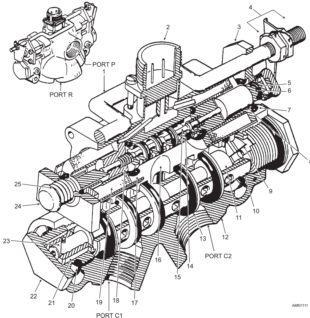
Figure 11-11.—Solenoid-operated selector valve.
