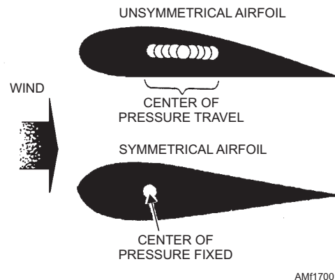
Figure 17-1.—Center of pressure.
