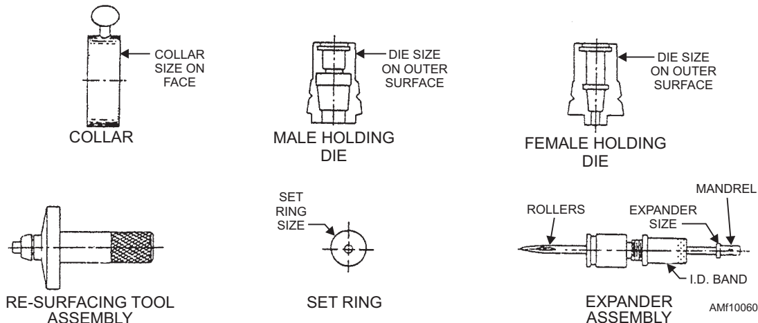
Figure 10-60.—Swaging and repair tool kit.
