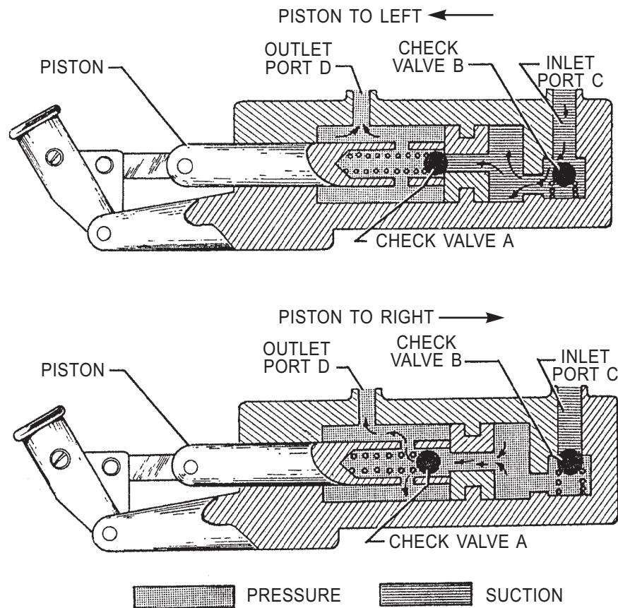
Figure 12-13.—Double-action hydraulic hand pump.
