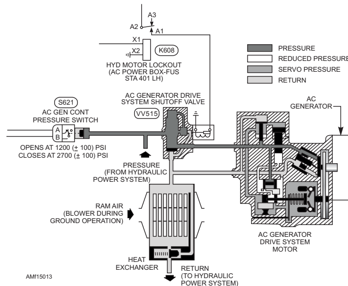
Figure 15-13.—AC generator drive system.
