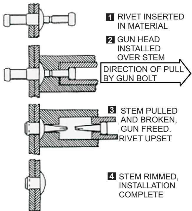
Figure 3-4.—Self-plugging rivet (friction lock).
