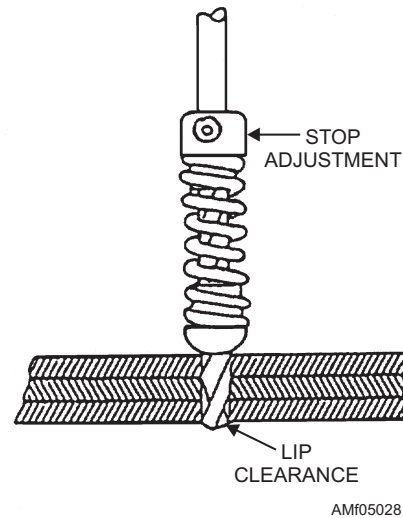
Figure 5-28.—Drill stop.
