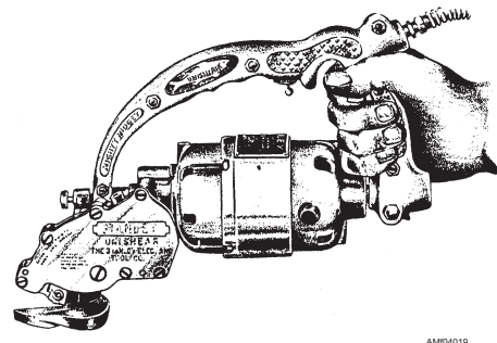
Figure 4-19.—18-gauge Unishear.
