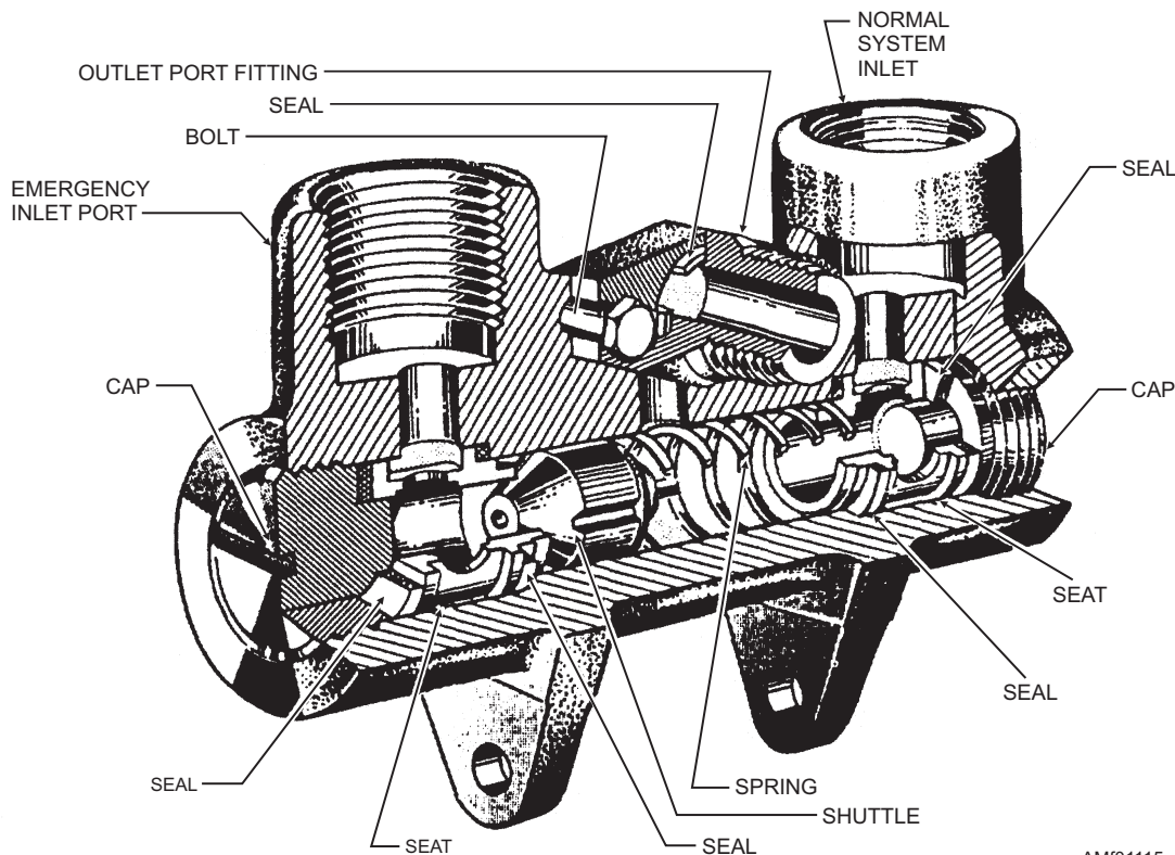
Figure 11-15.—Shuttle valve.
