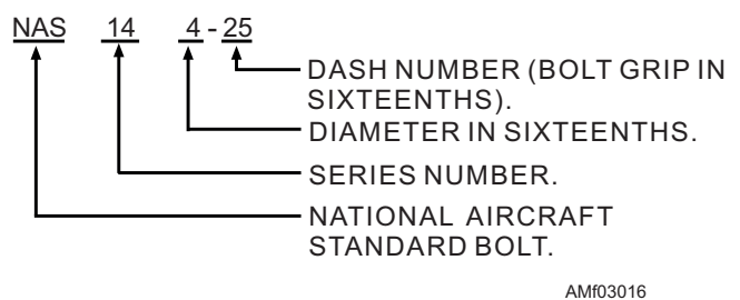
Figure 3-16.—NAS bolt part number breakdown.
