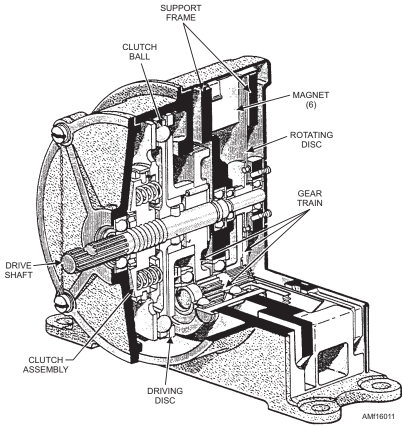
Figure 16-11.—Eddy current damper.
