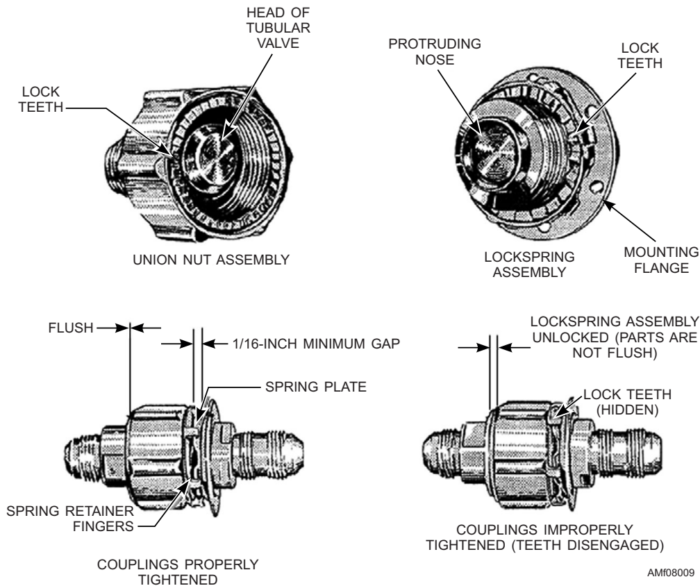
Figure 8-9.—Quick disconnects properly and improperly connected.
