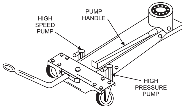
Figure 1-28.—T-Bar axle jack.
