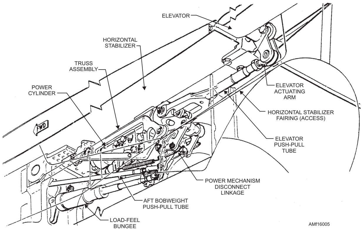
Figure 16-5.—Elevator power mechanism.
