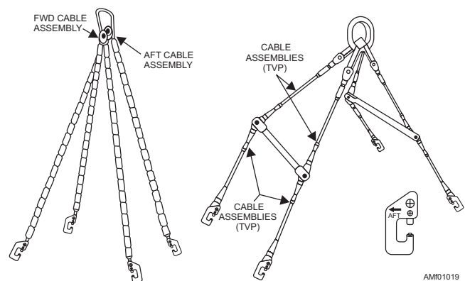
Figure 1-19.—Wire rope slings.
