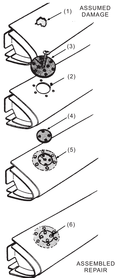
Figure 4-60.—Repair of small holes in skin with flush patch.
