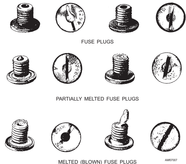
Figure 7-7.—Fuse plugs.
