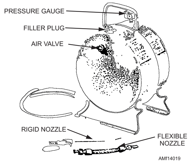
Figure 14-19.—Bleeder bomb.
