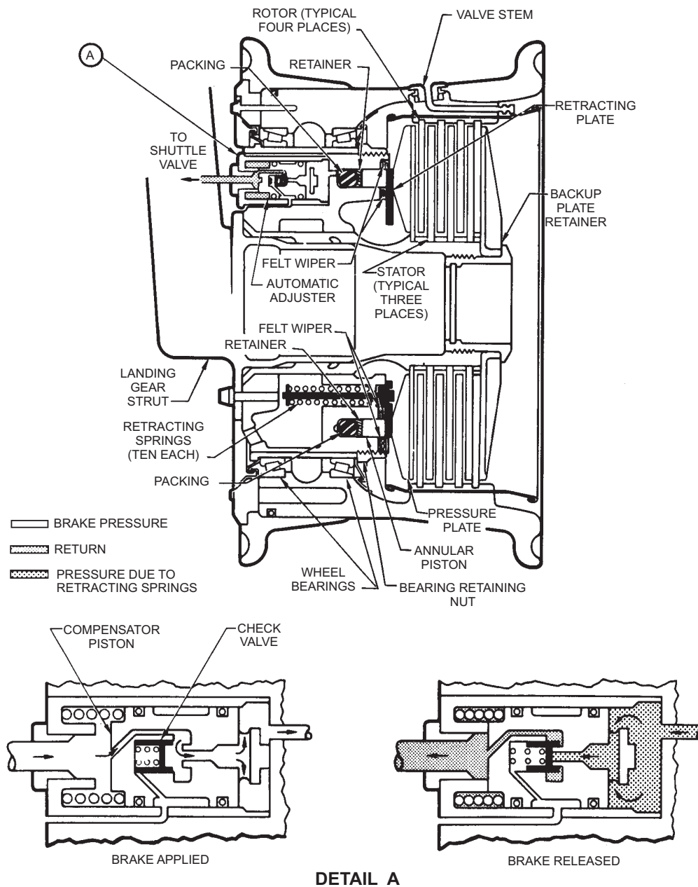
Figure 14-12.—Cross-sectional view of multiple disc brake.
