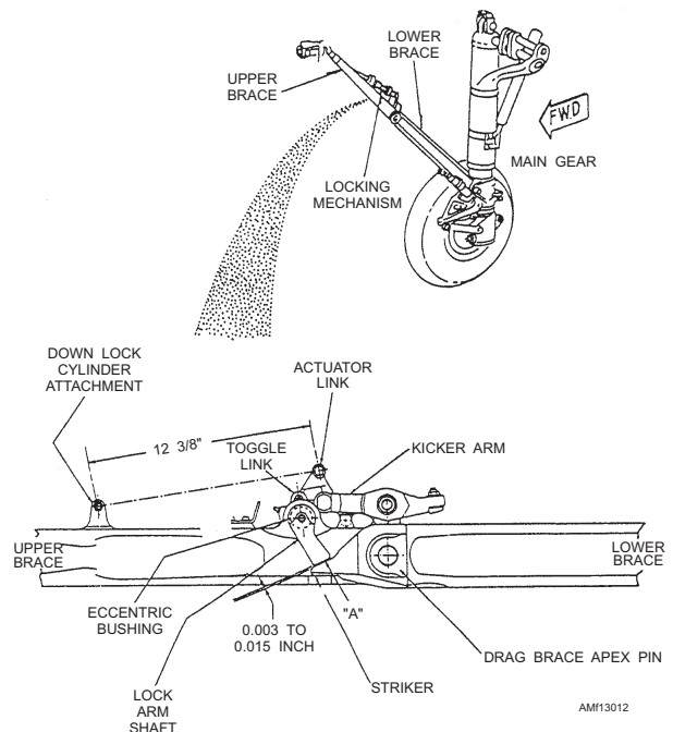
Figure 13-12.—Landing gear drag brace adjustment.
