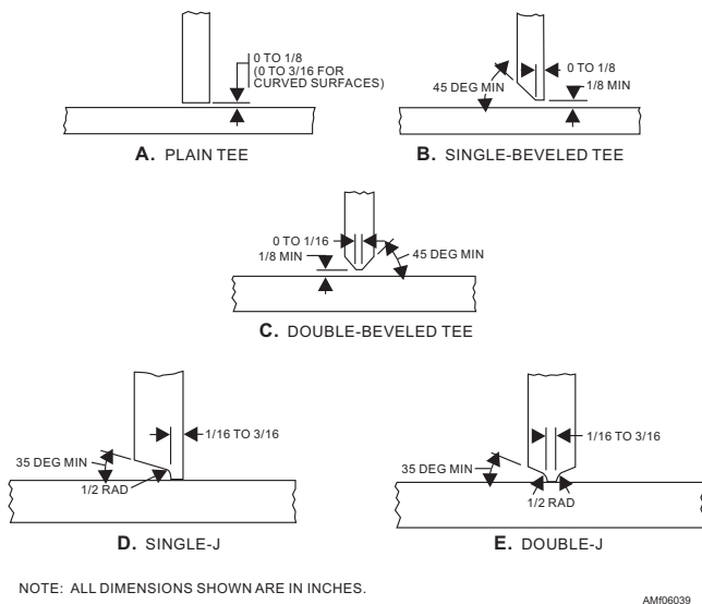
Figure 6-39.—Edge preparations for tee joint.
