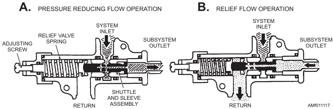
Figure 11-17.—Pressure-reducing valve operational schematic.
