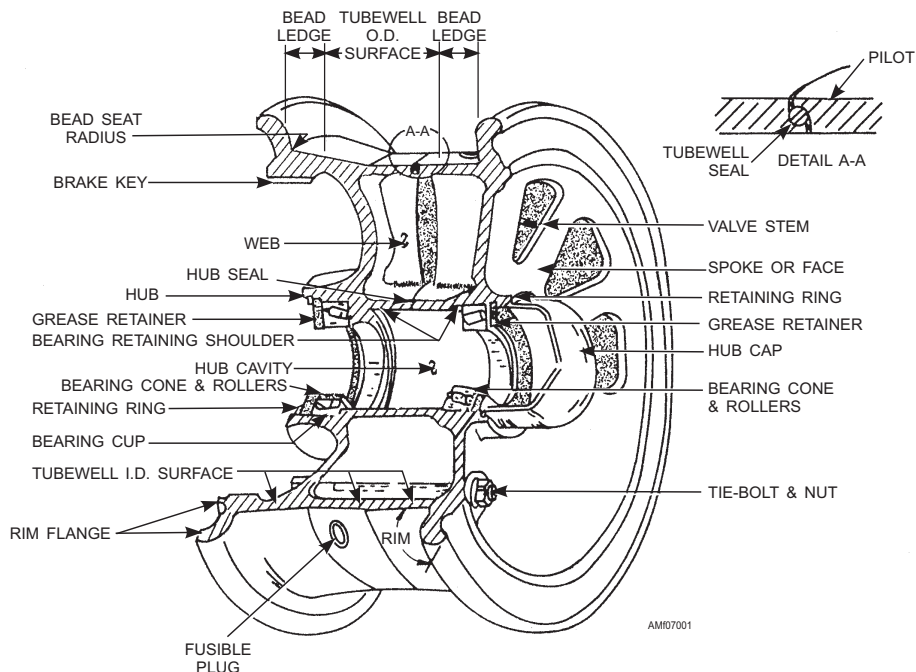
Figure 7-1.—Typical divided (split) wheel assembly.
