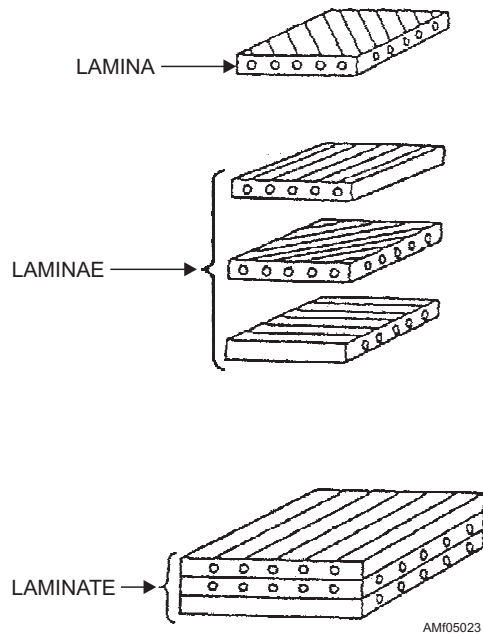
Figure 5-23.—Laminae stacking.
