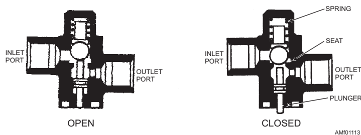
Figure 11-13.—Typical sequence valve.
