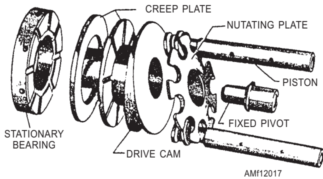
Figure 12-17.—Mechanical drive.
