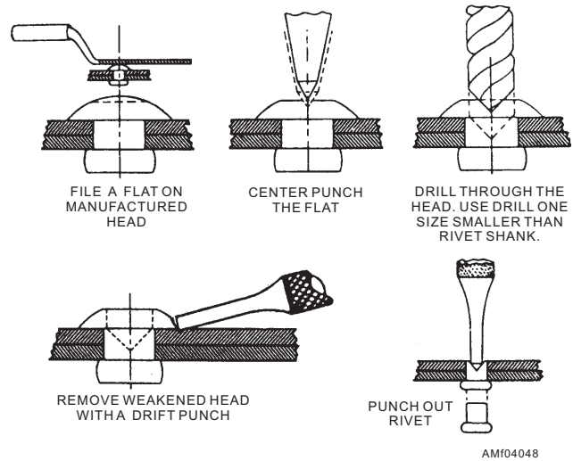
Figure 4-48.—Removal of rivets.
