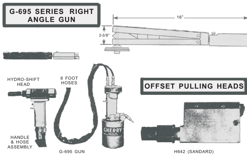
Figure 4-52.—Special use heads.
