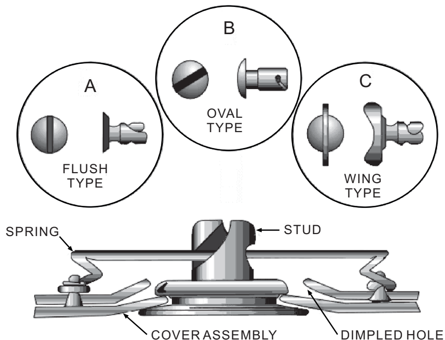
Figure 3-25.—Dzus fastener.
