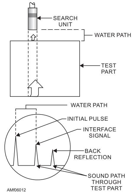
Figure 6-12.—Immersion method.
