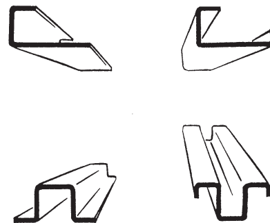
Figure 4-37.—Types of bends on a bar folder.
