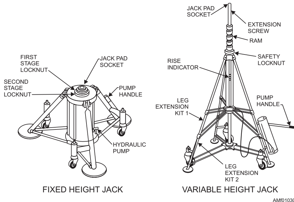
Figure 1-30.—Airframe (tripod) jacks.
