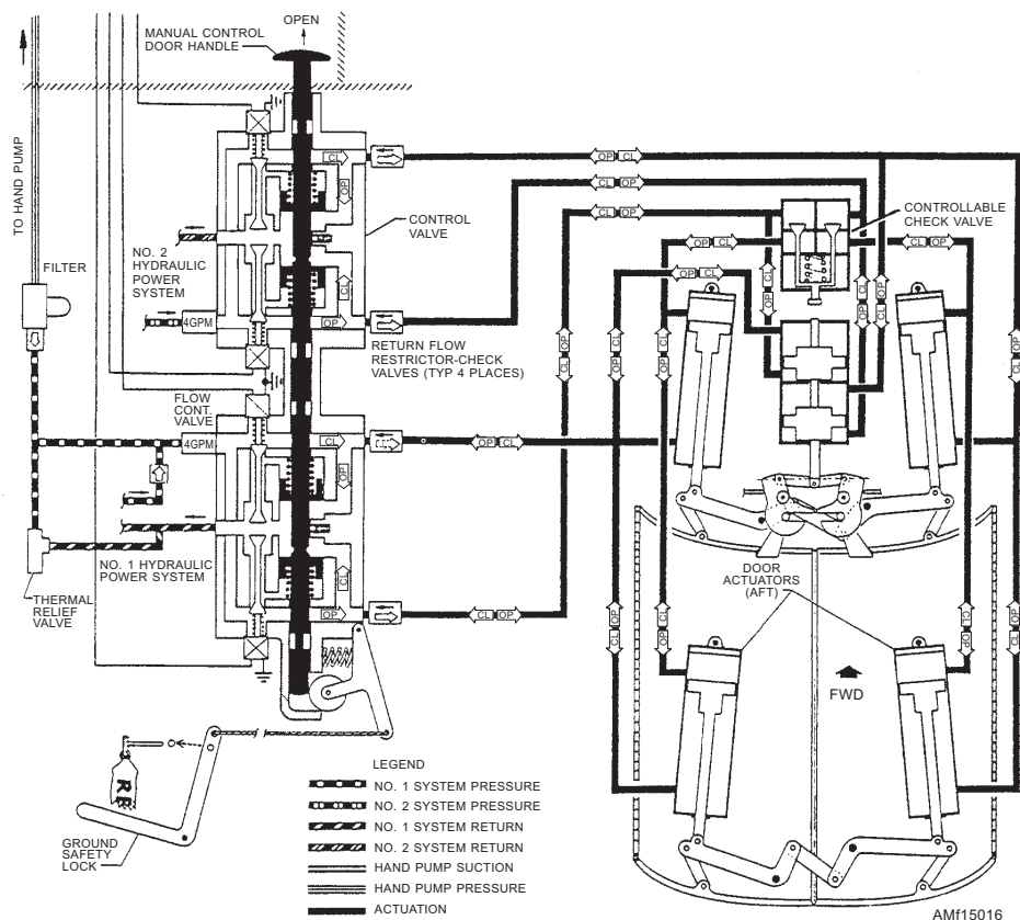
Figure 15-16.—Bomb bay door hydraulic schematic.
