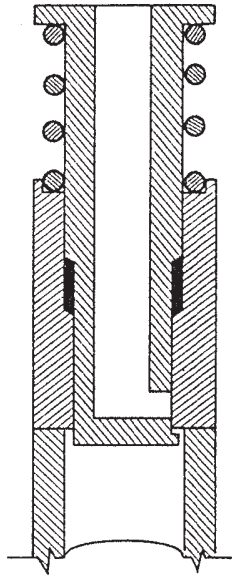
Figure 12-6.—Manual air bleed valve.
