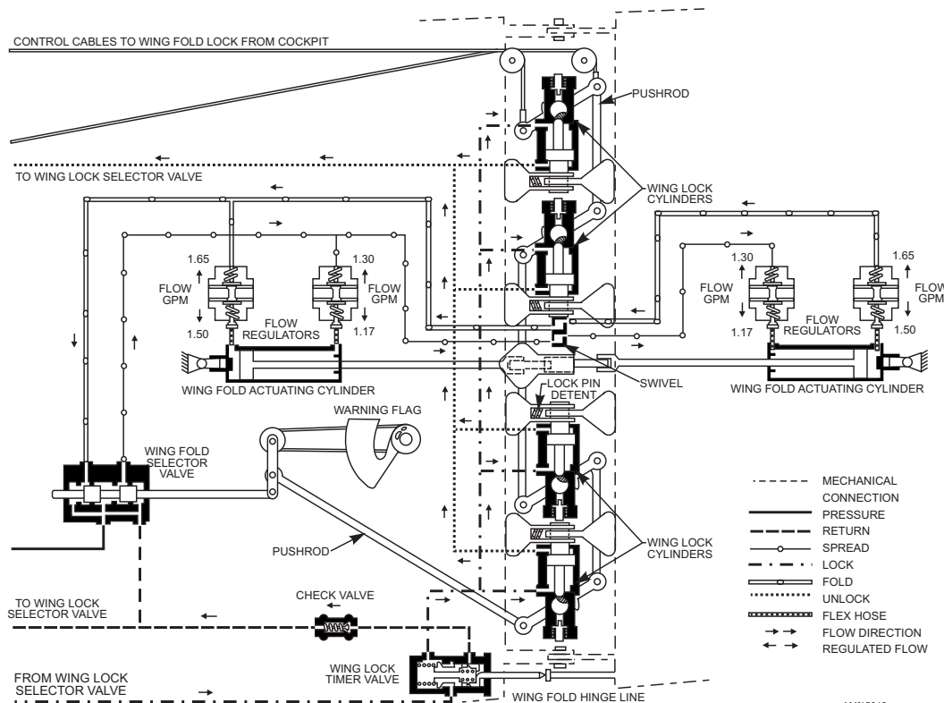
Figure 15-12.—Wing fold schematic (spread and locked condition).
