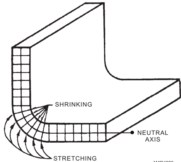
Figure 4-29.—Neutral axis.
