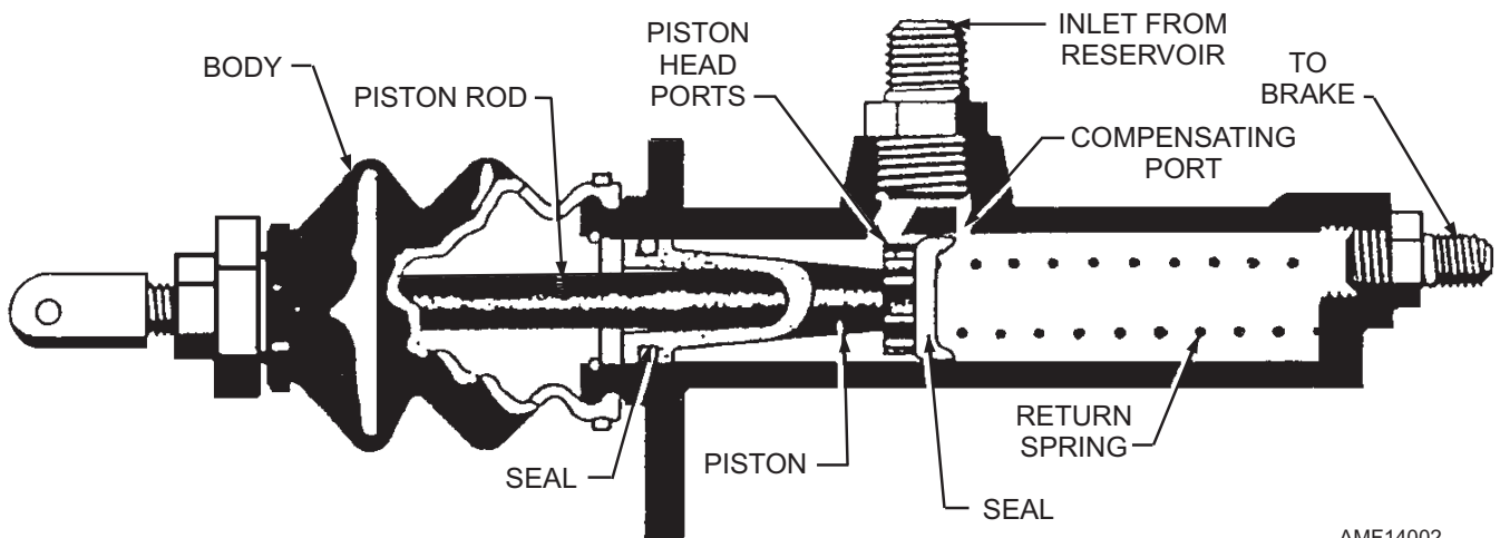
Figure 14-2.—Goodyear master brake cylinder.
