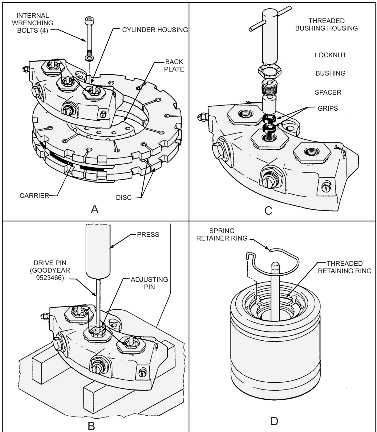
Figure 14-31.—Seal replacement and piston return adjustment.
