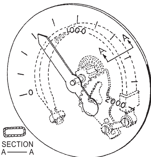
Figure 12-36.—Bourdon tube.
