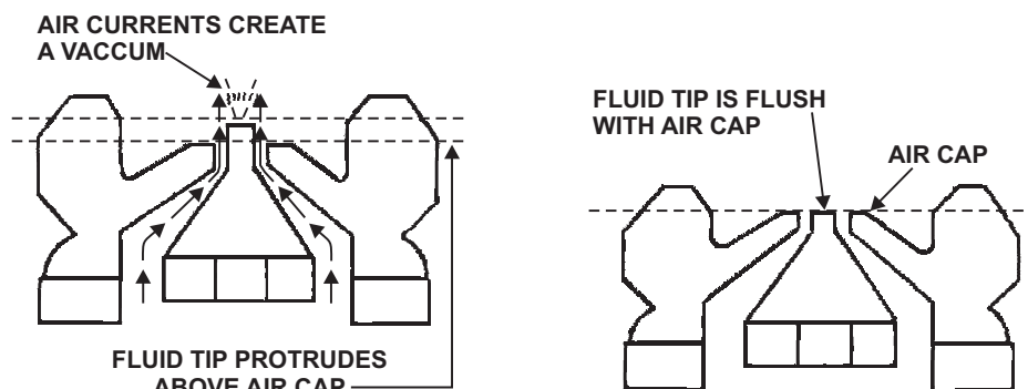
Figure 5-34.—Suction and pressure fluid tips and air caps.
