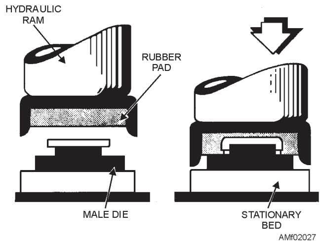
Figure 2-27.—Guerin process.
