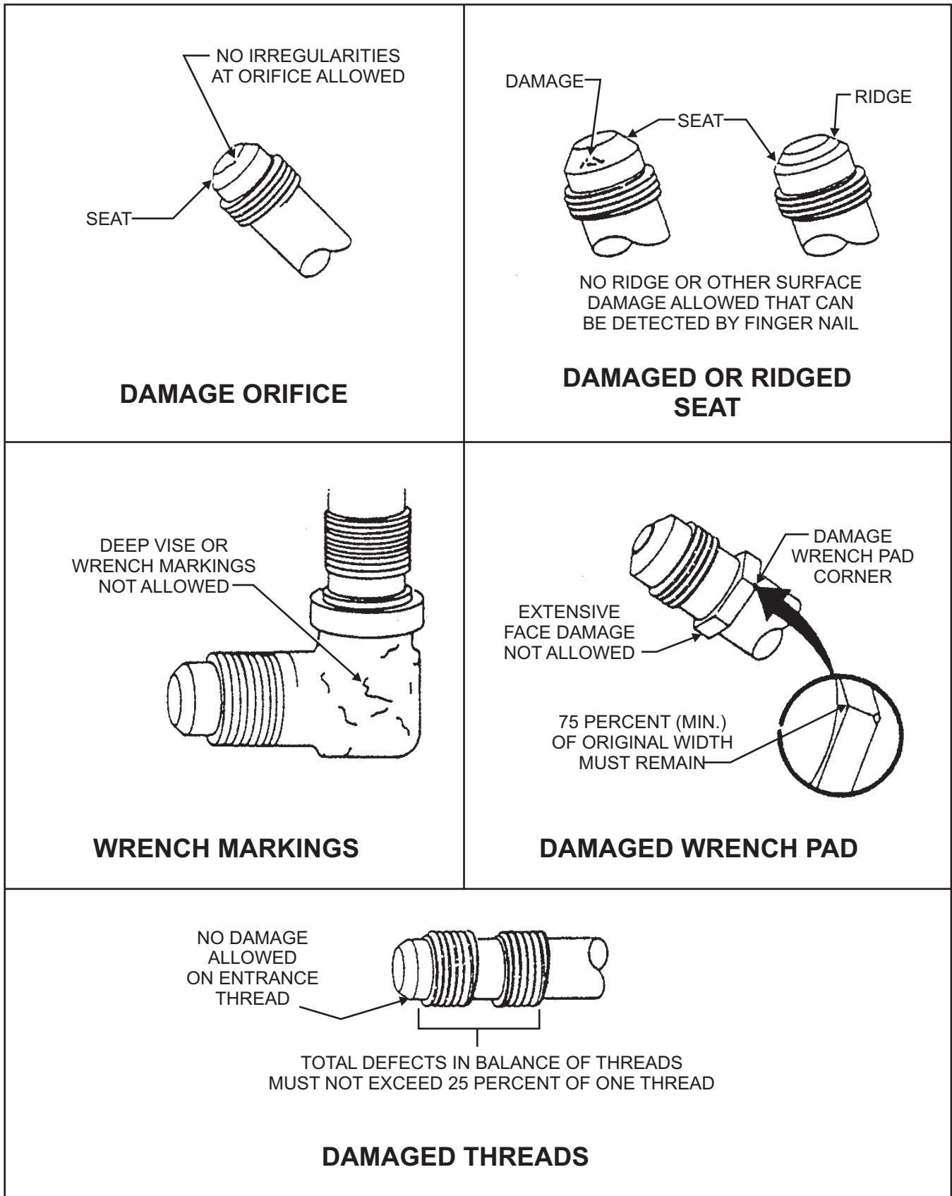
Figure 10-44.—Damaged fittings.
