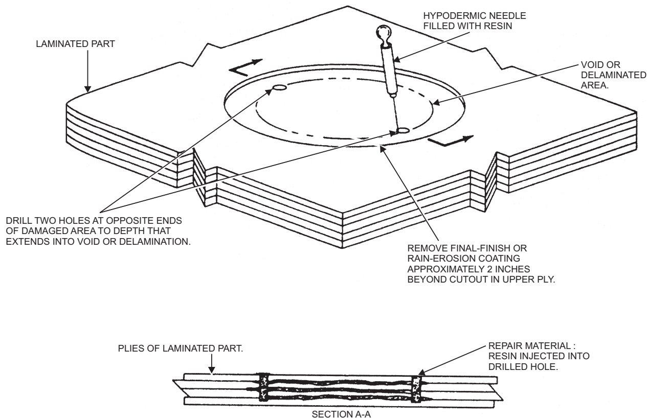
Figure 5-10.—Delaminated ply repair.
