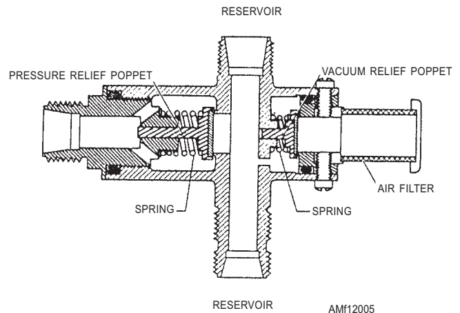
Figure 12-5.—Pressure and vacuum relief valve.
