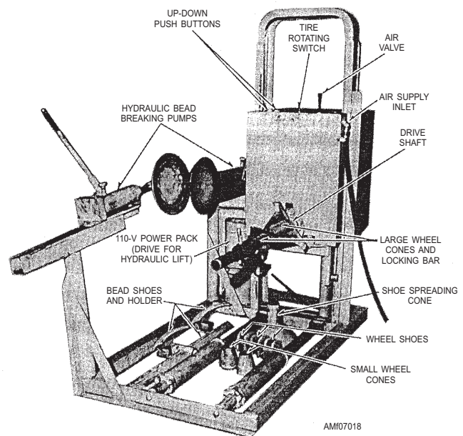
Figure 7-18.—Aircraft wheel holder and tire bead-breaking machine.
