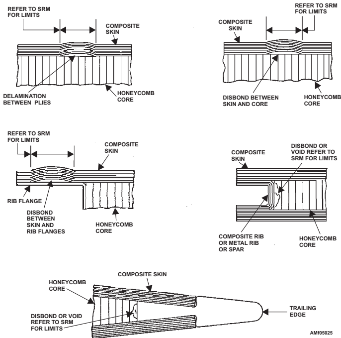
Figure 5-25.—Example of negligible damage on composite material.
