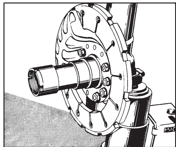
Figure 14-9.—Typical single disc brake installation.
