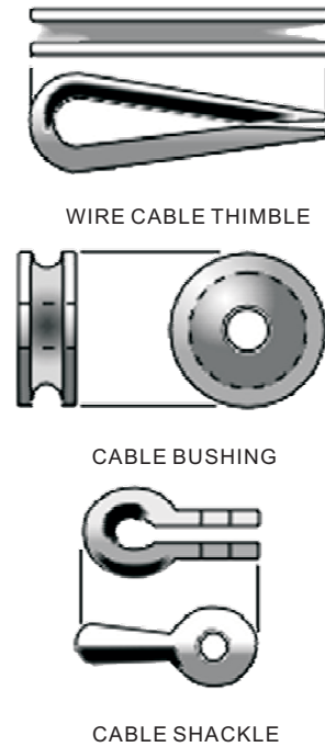
Figure 3-34.—Thimble, bushing, and shackle fittings.
