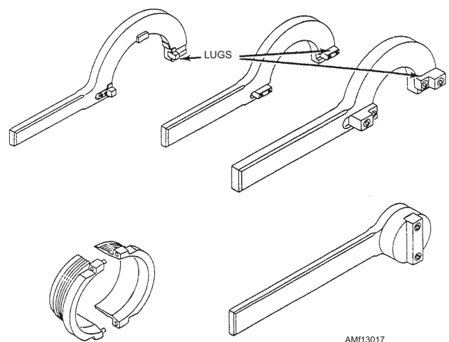
Figure 13-17.—Landing gear shock strut tools.
