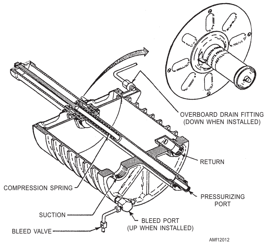
Figure 12-12.—Typical fluid-pressurized reservoir.
