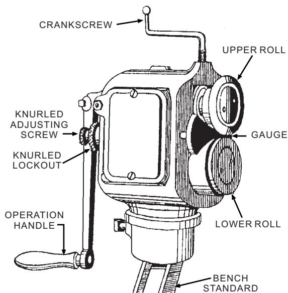
Figure 4-28.—Rotary machine.
