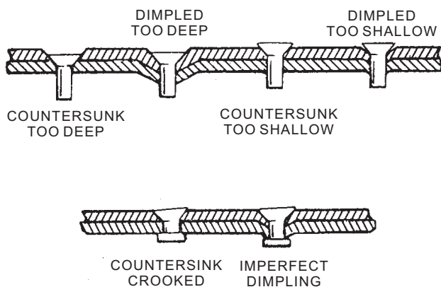
Figure 4-45.—Incorrect countersinking.
