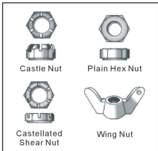
Figure 3-17.—Nuts.
