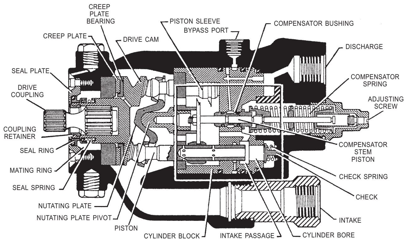
Figure 12-16.—Internal features of the Stratopower pump.
