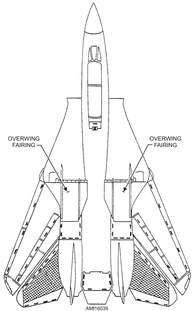
Figure 16-39.—Wing oversweep position—manual control.
