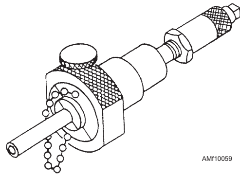
Figure 10-59.—Dynatube swaging process.
