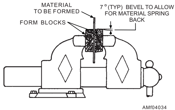
Figure 4-34.—Preparation for straight bend by hand.
