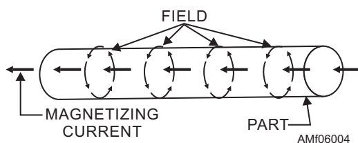
Figure 6-4.—Magnetic field in part used as a conductor.
