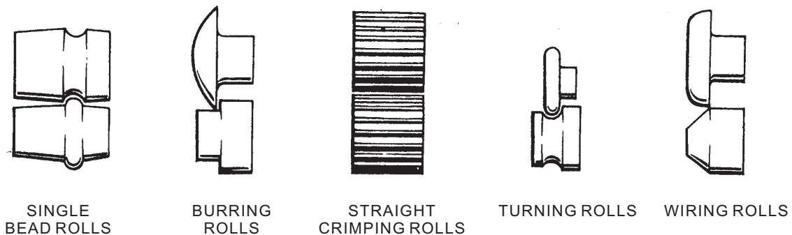
Figure 4-41.—Roll dies used on a rotary machine.
