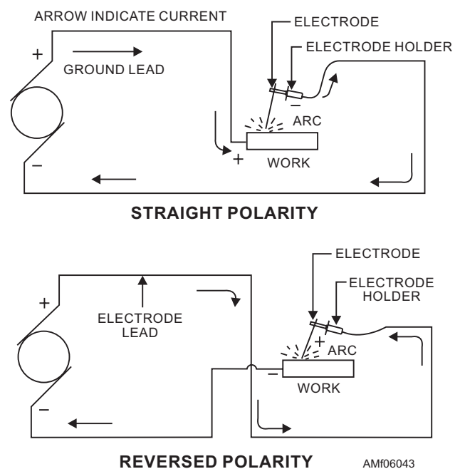
Figure 6-43.—Straight and reverse polarity in electric welding. AMf06043
