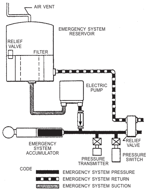
Figure 12-40.—Schematic diagram of typical emergency power system (electric-motor driven).
