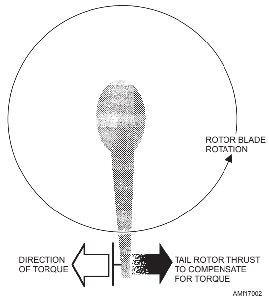
Figure 17-2.—Torque reaction.
