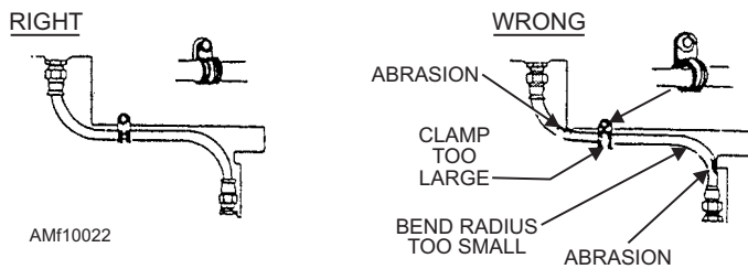
Figure 10-22.—Hose clamp mounting.
