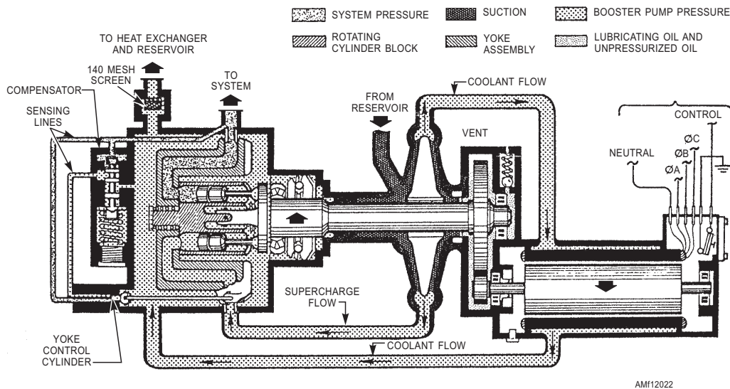
Figure 12-22.—Motor-driven variable displacement piston pump schematic.
