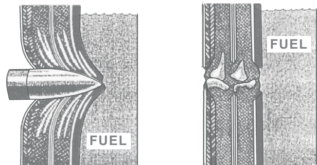
Figure 4-73.—Bullet-sealing action.
