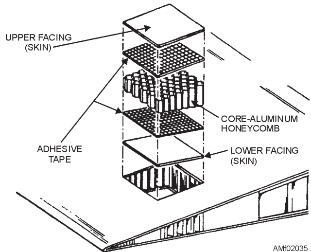
Figure 2-35.—Sandwich construction.
