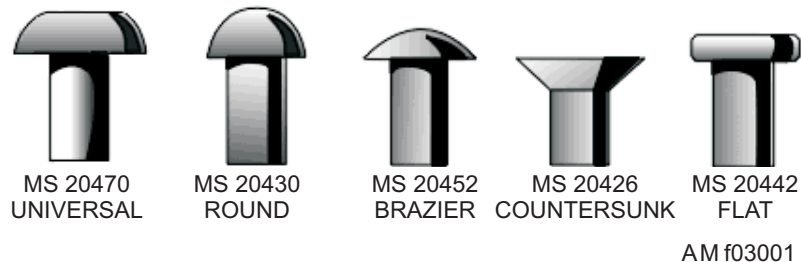
Figure 3-1.—Rivet head shapes and code numbers.
