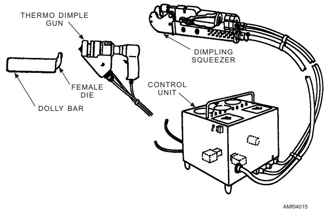
Figure 4-15.—Hot dimpling kit.
