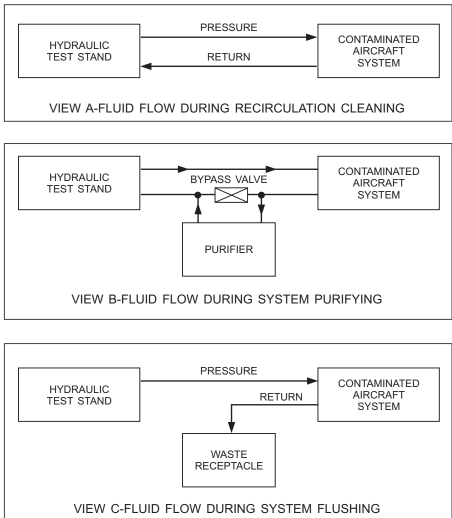
Figure 8-6.—Fluid flow during decontamination.
