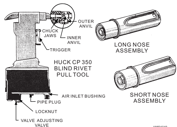
Figure 4-49.—Self-plugging rivet (mechanical lock) pull tool.
