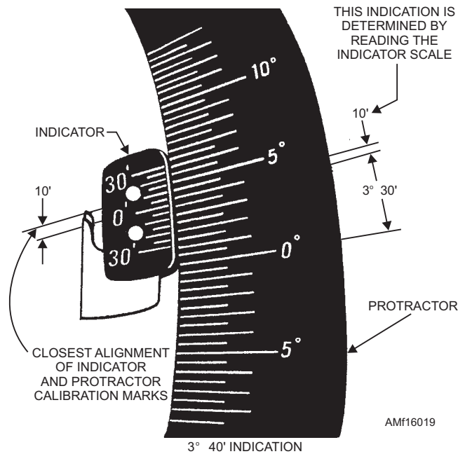
Figure 16-19.—Aileron throw protractor indications.
