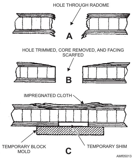
Figure 5-13.—Scarfed repair method.
