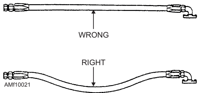
Figure 10-21.—Hose slack.
