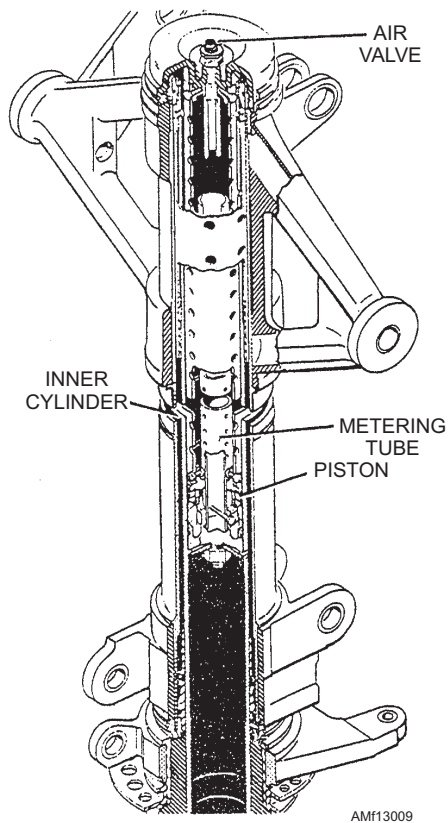
Figure 13-9.—Landing gear shock strut (metering tube type).
