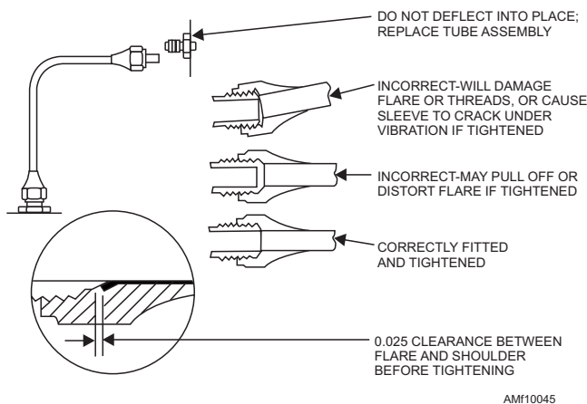
Figure 10-45.—Correct and incorrect methods of installing flared fittings.
