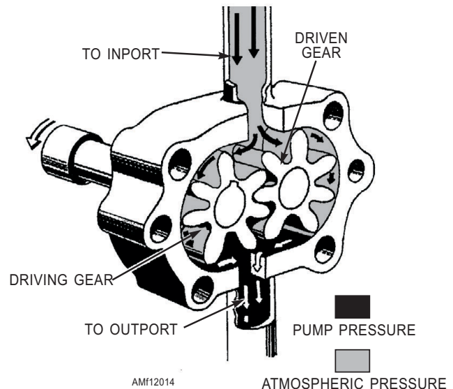
Figure 12-14.—Gear-type power pump.
