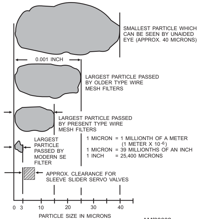
Figure 8-2.—Graphic comparison of particle sizes.
