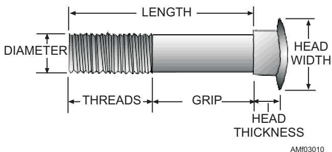
Figure 3-10.—Bolt terms and dimensions.
