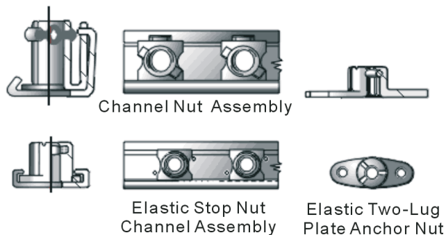
Figure 3-18.—Self-locking plate nuts.
