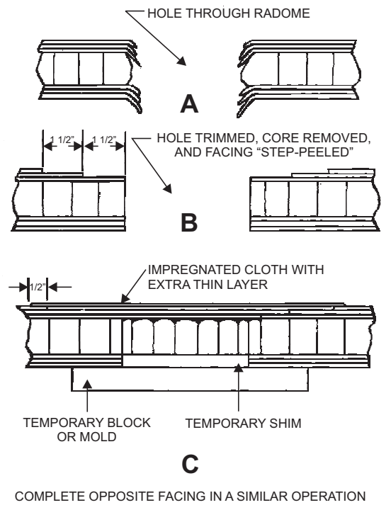
Figure 5-14.—Stepped repair method.
