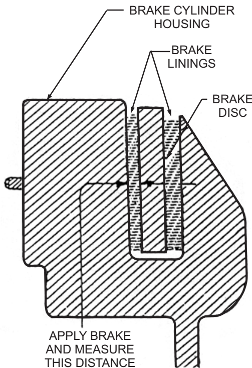
Figure 14-16.—Checking lining wear (Method No. 1).
