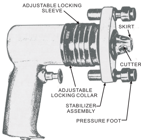
Figure 4-9.—Rivet-head shaver.
