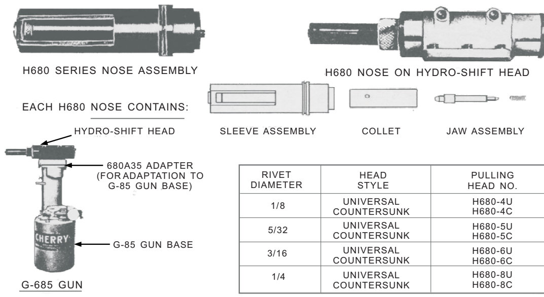
Figure 4-51.—Hydro-shift series gun.
