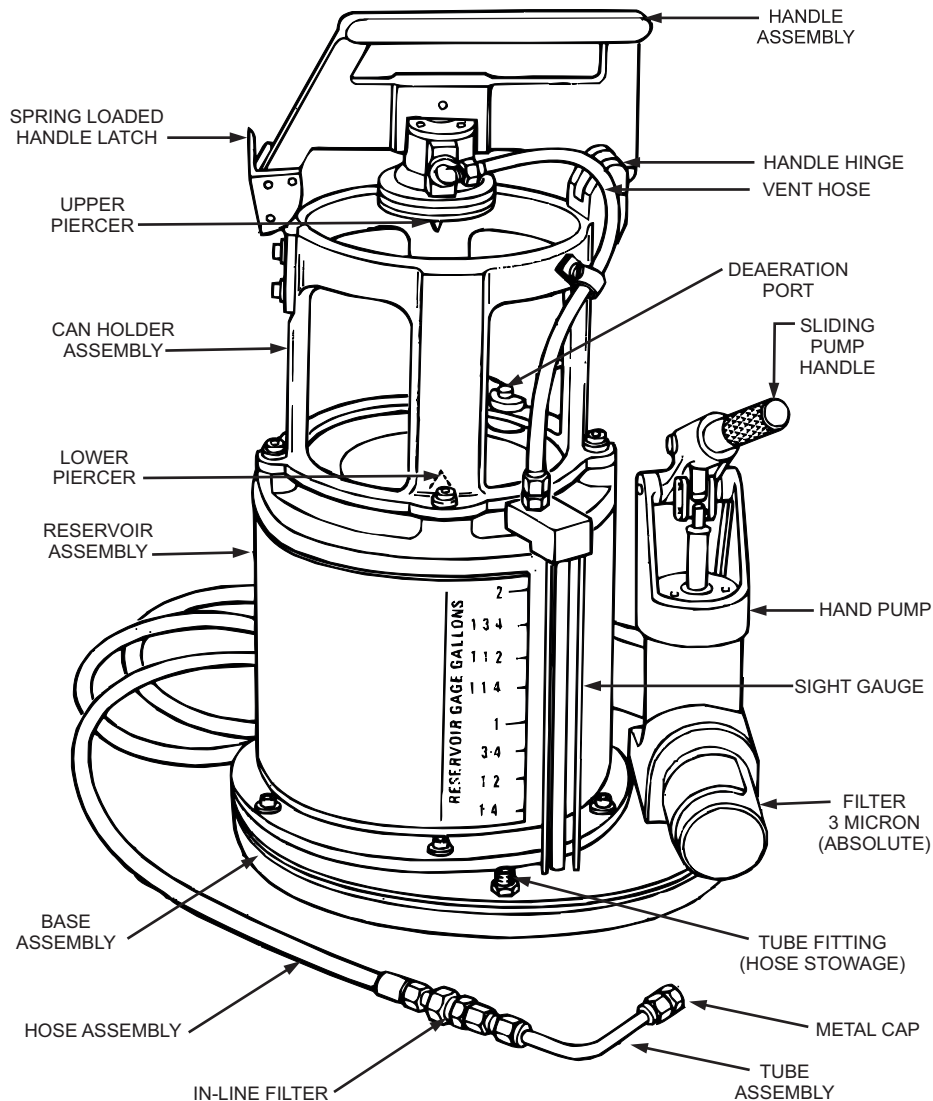
Figure 9-2.—Model HSU-1 fluid service unit.
