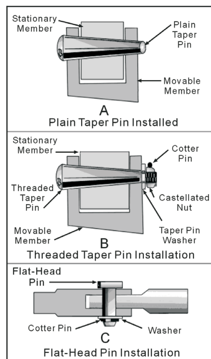
Figure 3-30.—Types of aircraft pins.
