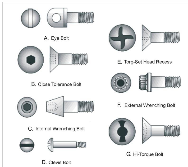
Figure 3-12.—Bolt Heads.
