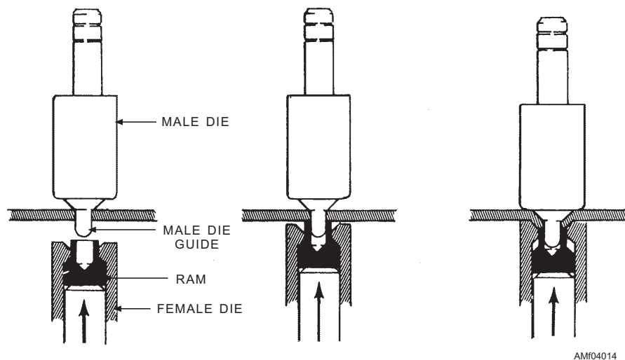
Figure 4-14.—Dimple countersinking.
