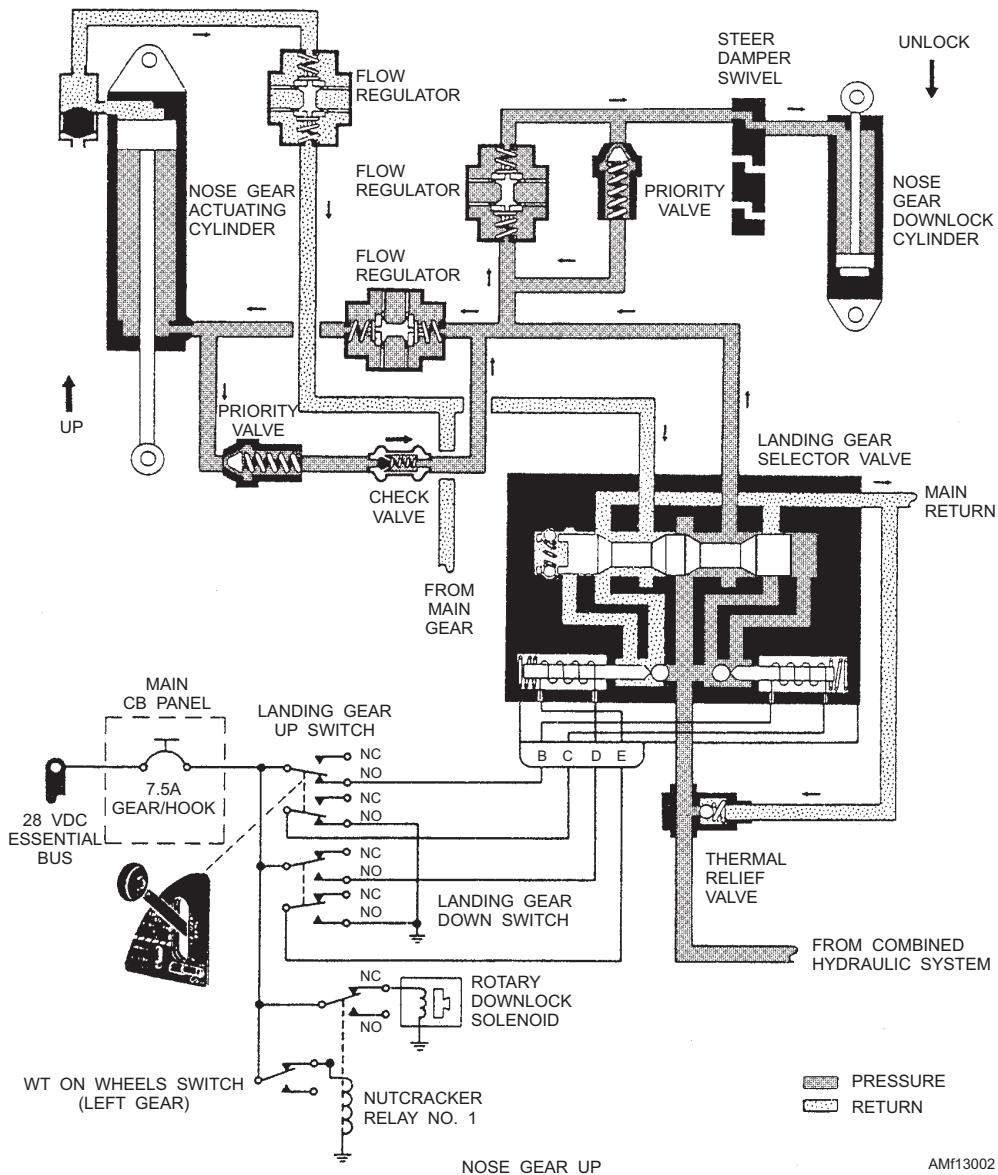
Figure 13-2.—Nose gear up cycle schematic.
