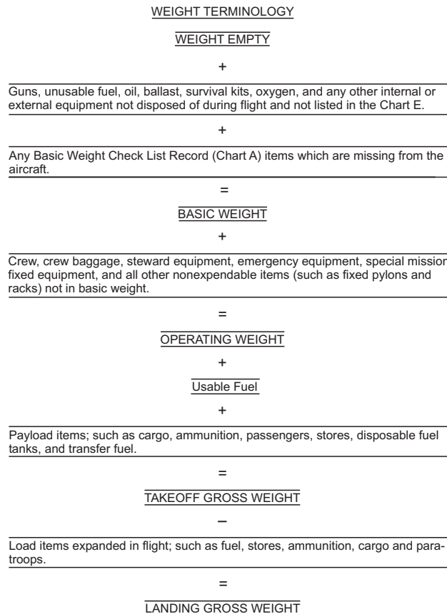
Figure 1-16.—Weight terminology.
