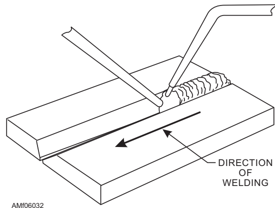
Figure 6-32.—Forehand welding.
