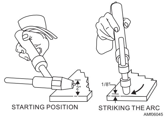
Figure 6-45.—Starting the arc.
