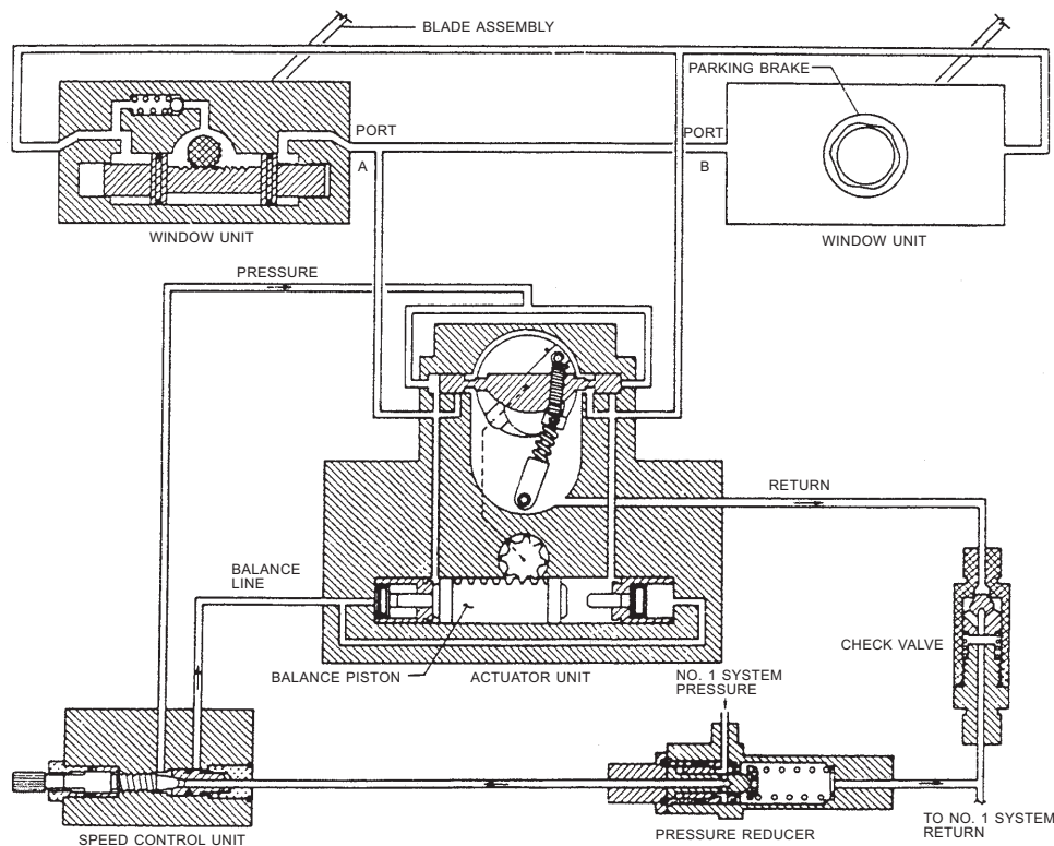
Figure 15-17.—Windshield wiper schematic.
