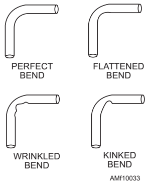
Figure 10-33.—Tubing bends.
