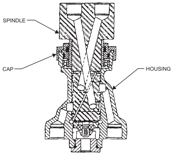
Figure 17-14.—Rotor coupling.
