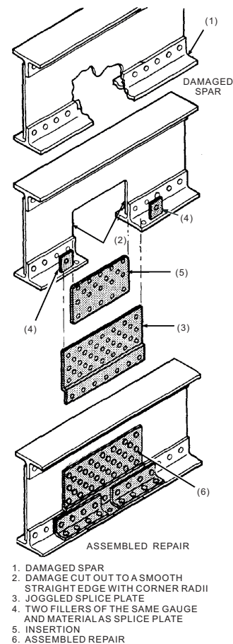
Figure 4-69.—Spar repair by insertion.
