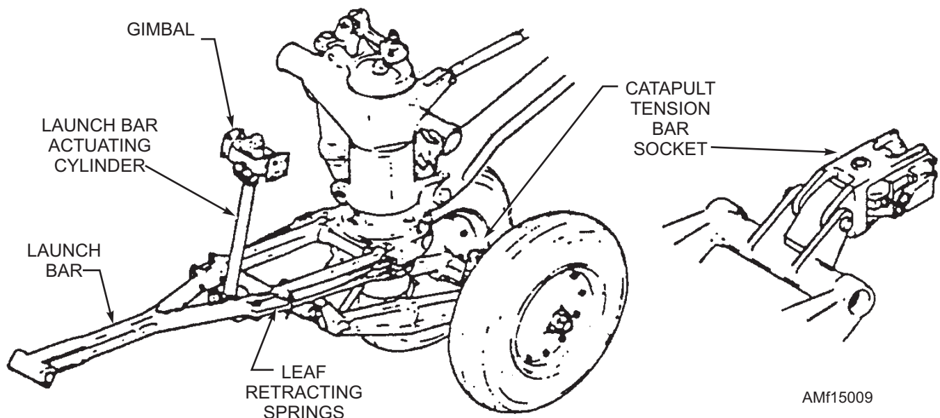
Figure 15-9.—Catapult system.
