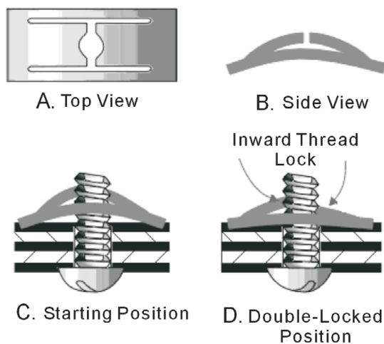
Figure 3-19.—Sheet spring nut.
