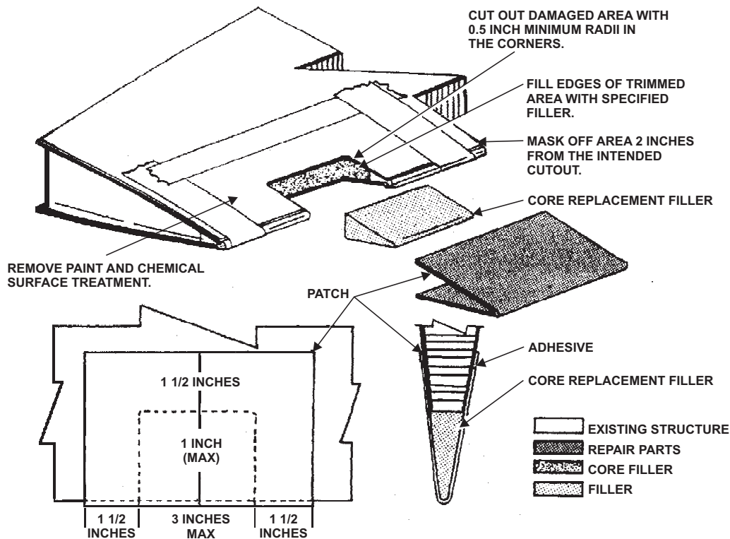
Figure 5-20.—Trailing edge repair (sandwich construction).
