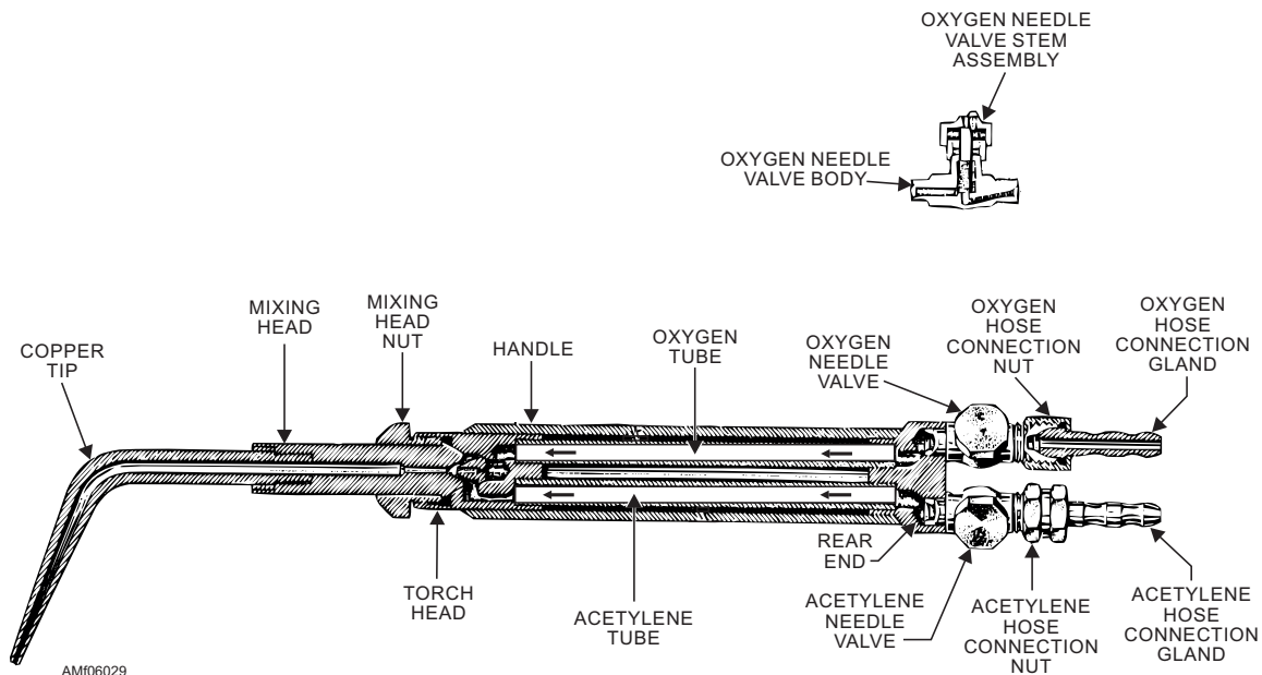
Figure 6-29.—Equal pressure welding torch.
