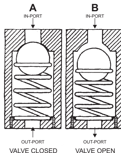
Figure 11-12.—Typical check valve.
