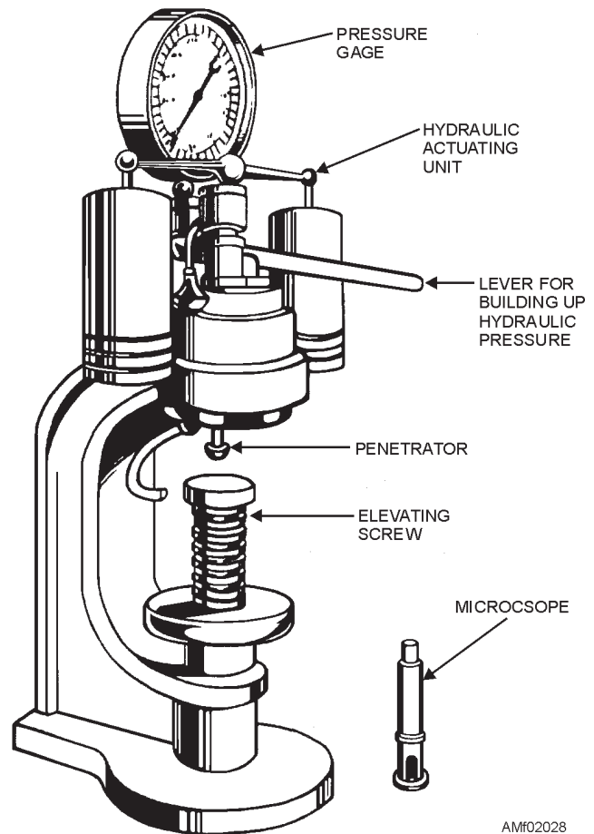
Figure 2-28.—Brinell hardness tester.
