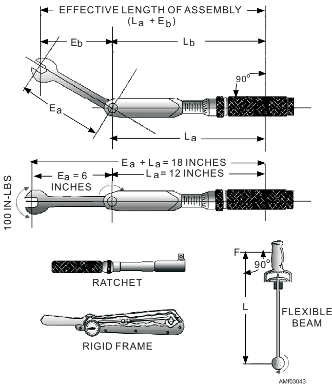
Figure 3-43.—Torque wrenches.
