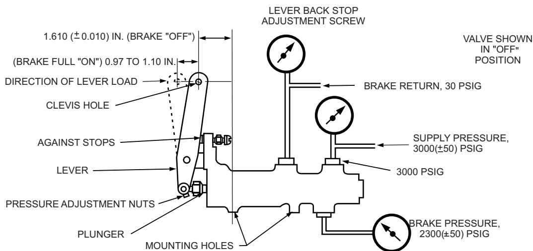
Figure 14-21.—Operational test setup—power brake valve.
