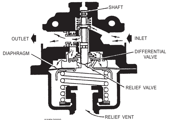
AMf12009 Figure 12-9.—Air pressure regulator.
