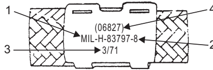
WIRE BRAID COVERED SYNTHETIC RUBBER HOSE
