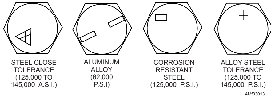
Figure 3-13.—Bolt head markings.
