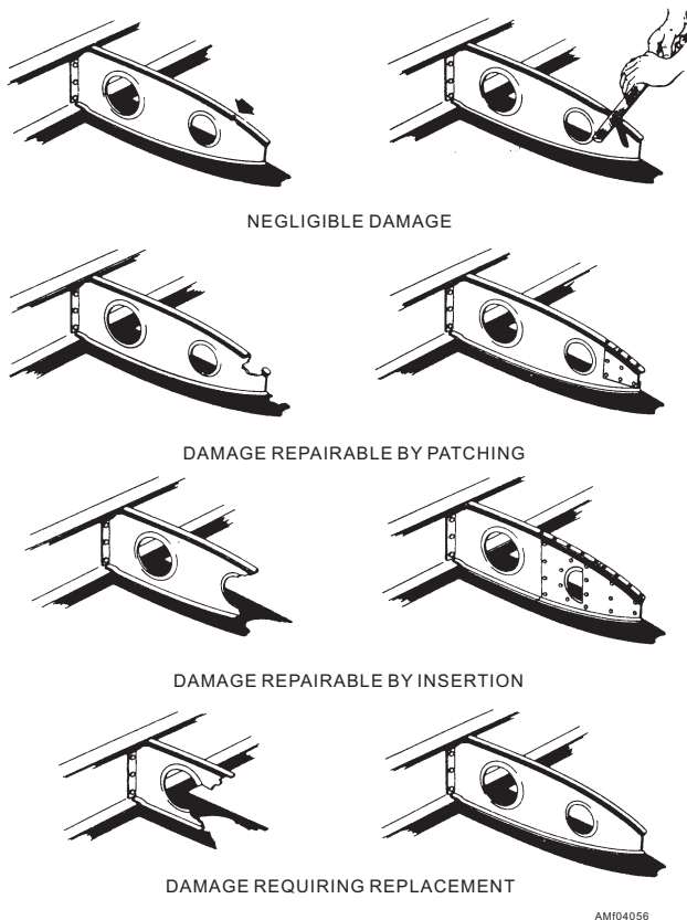
Figure 4-56.—Classifications of damage.
