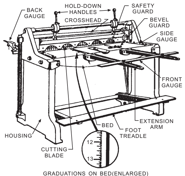
Figure 4-17.—Squaring shears.
