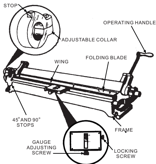
Figure 4-24.—Bar folder.
