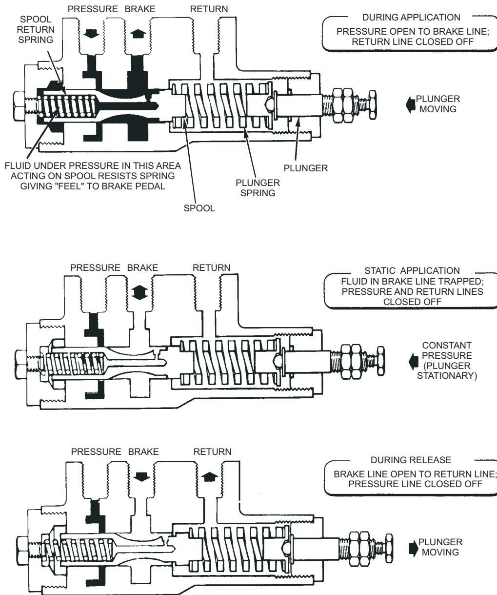
Figure 14-7.—Power brake control valve (sliding spool type).
