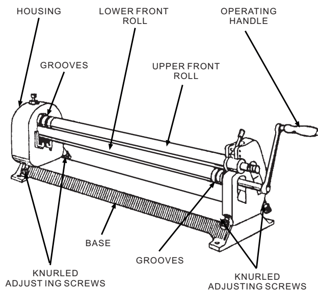
Figure 4-27.—Slip-roll forming machine.
