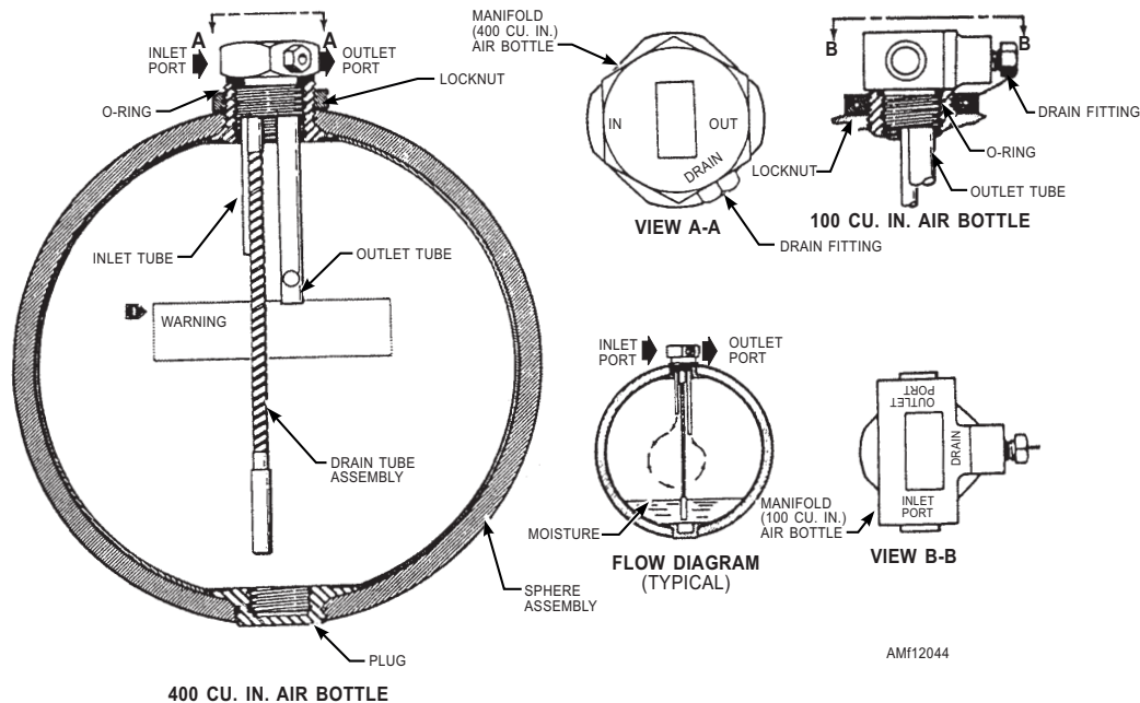
Figure 12-44.—Air cylinder.
