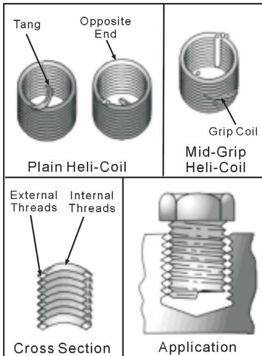
Figure 3-31.—Heli-coil insert.
