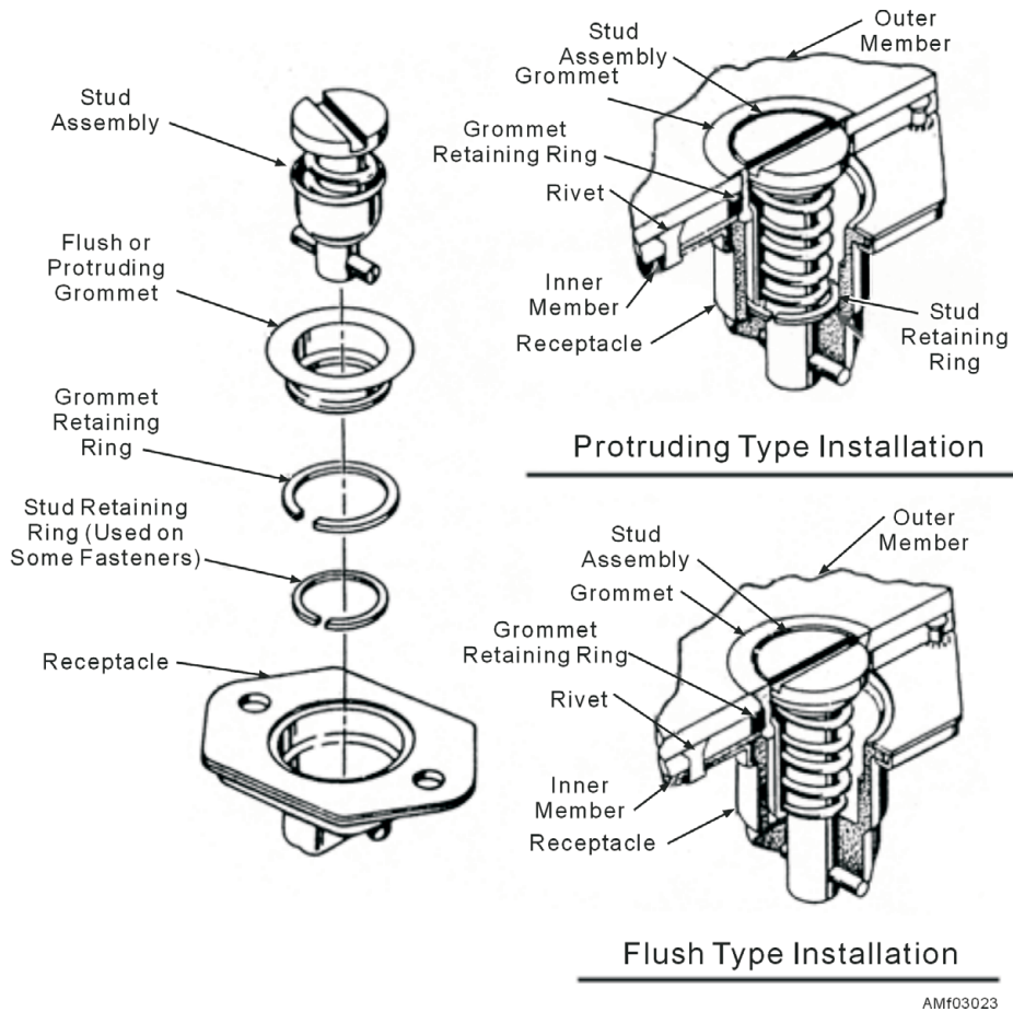
Figure 3-23.—Camloc 4002 series fastener.
