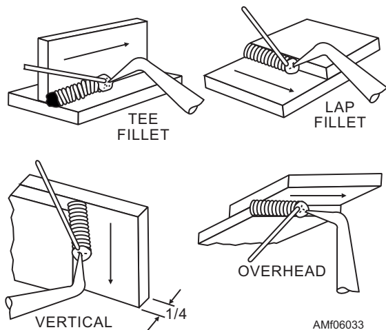
Figure 6-33.—Backhand welding.
