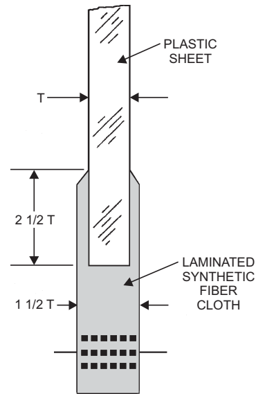
Figure 5-4.—Approved edge attachment for solid plastic.
