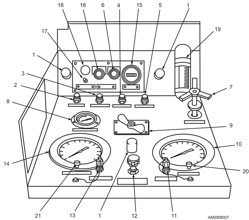
Figure 9-7.—Primary control panel controls and indicators.
