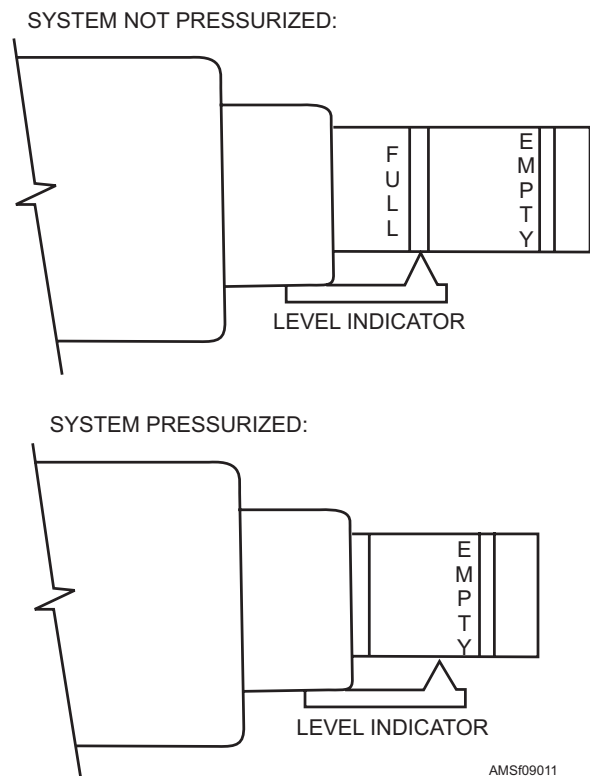
Figure 9-11.—Reservoir level changes (reservoir sink) presence of air in system.
