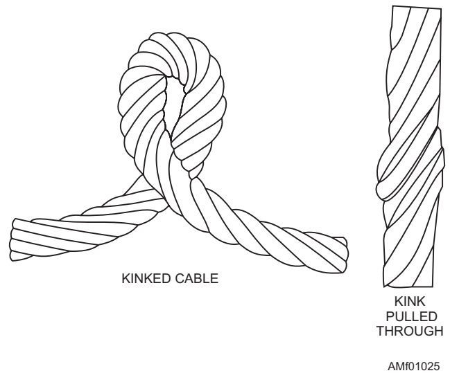
Figure 1-25.—Cable damage resulting from a pulled-through kink.
