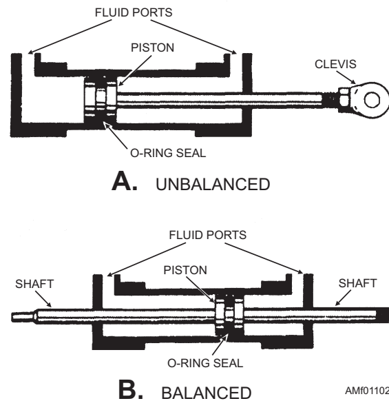
Figure 11-2.—Double-acting, piston-type, actuating cylinders.
