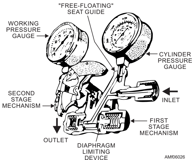
Figure 6-26.—Two-stage regulator.
