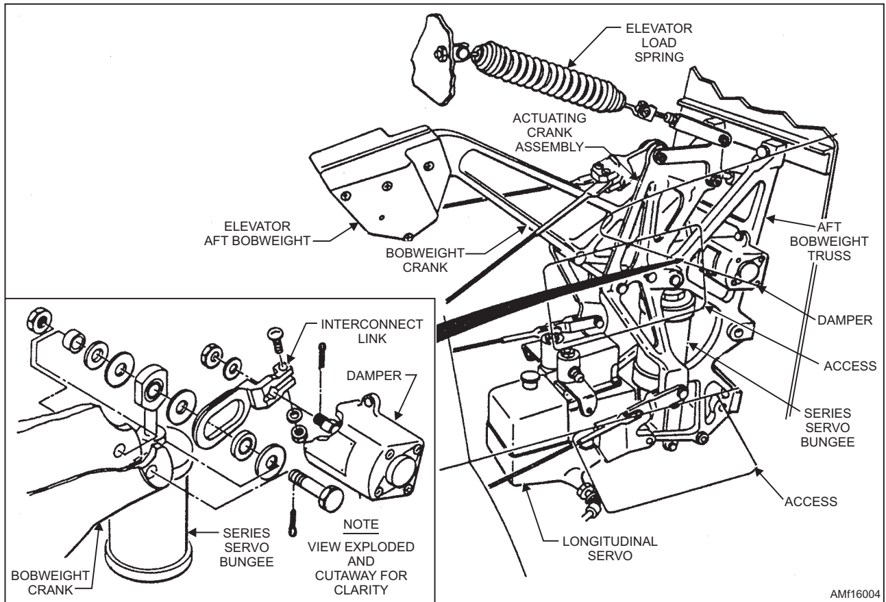
Figure 16-4.—Elevator aft bobweight and damper assembly.
