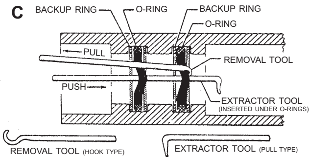
DUAL INTERNAL O-RING REMOVAL (USING PUSH TYPE EXTRACTOR AND HOOK TYPE REMOVAL TOOLS)
