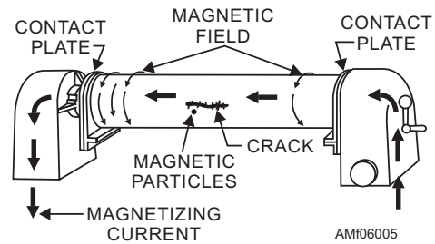
Figure 6-5.—Creating a circular magnetic field in a part.
