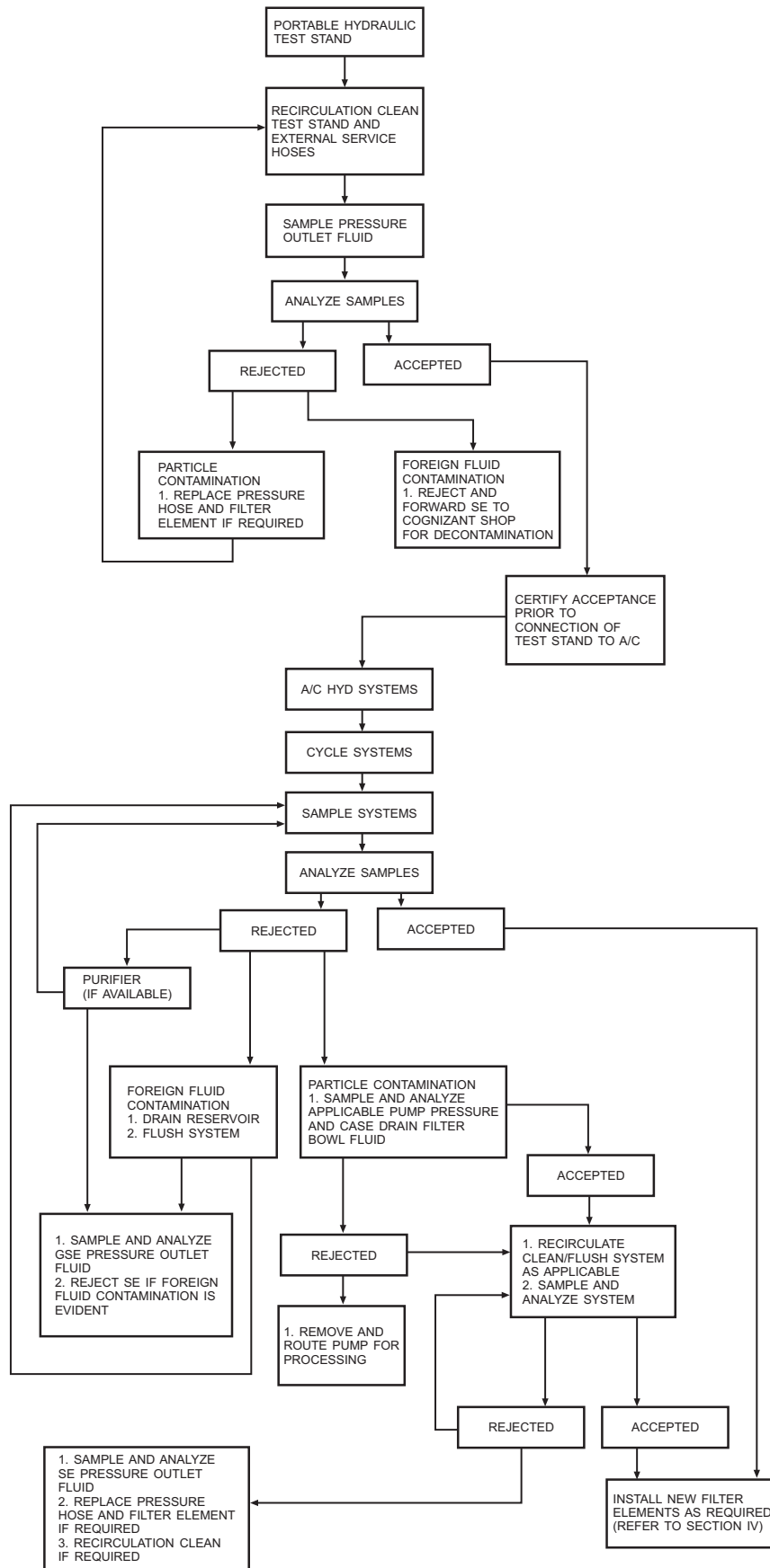
Figure 8-7.—Sequence control chart for aircraft system decontamination.
