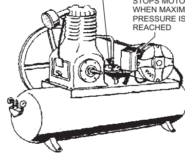
Figure 5-39.—Air compressors.
