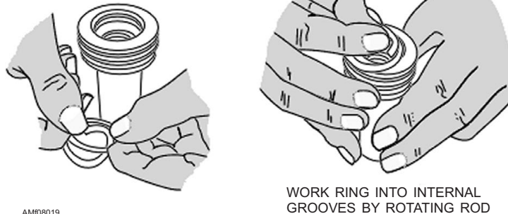
Figure 8-19.—Installation of Teflon® backup rings (internal).
