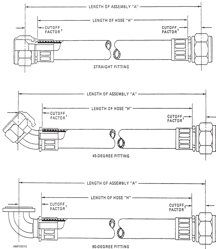
Figure 10-10.—Determining hose assembly length.
