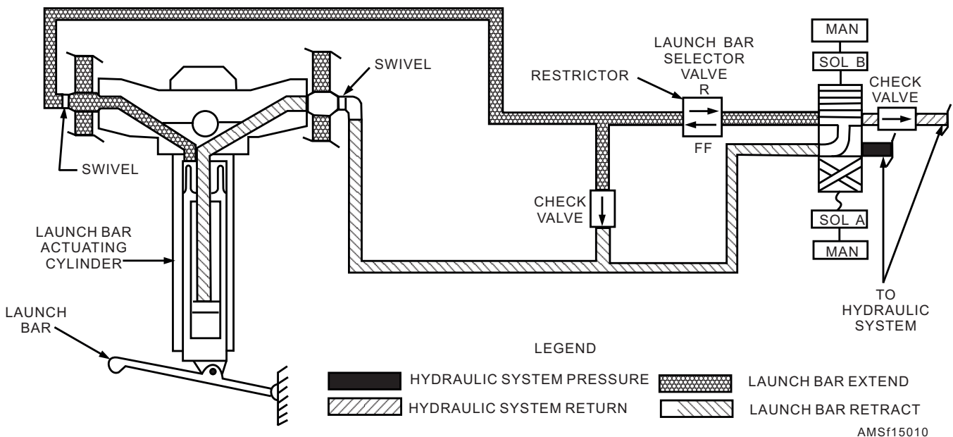
Figure 15-10.—Catapult system hydraulic schematic.
