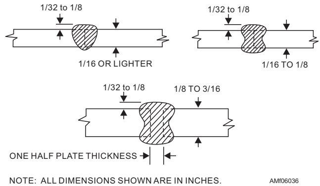
Figure 6-36.—Butt joints in light sections.
