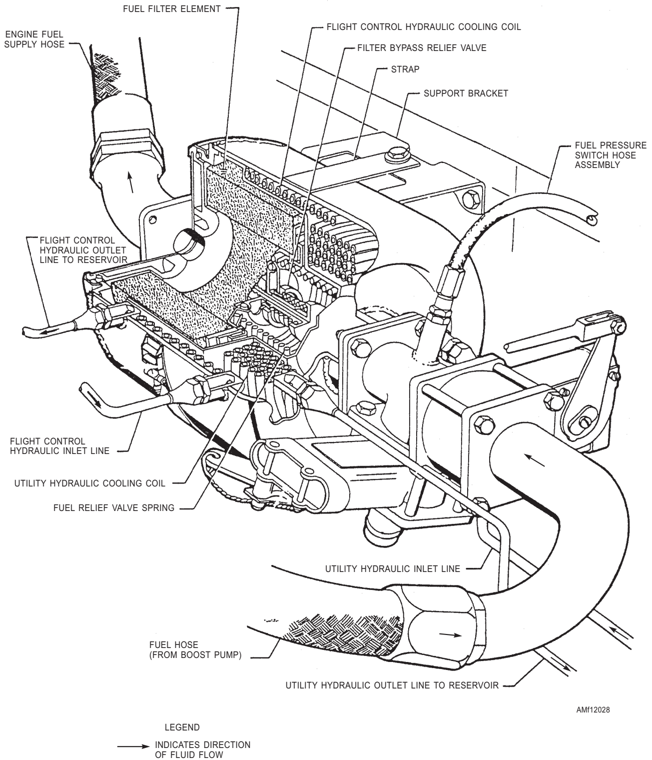
Figure 12-28.—Hydraulic fluid cooler.
