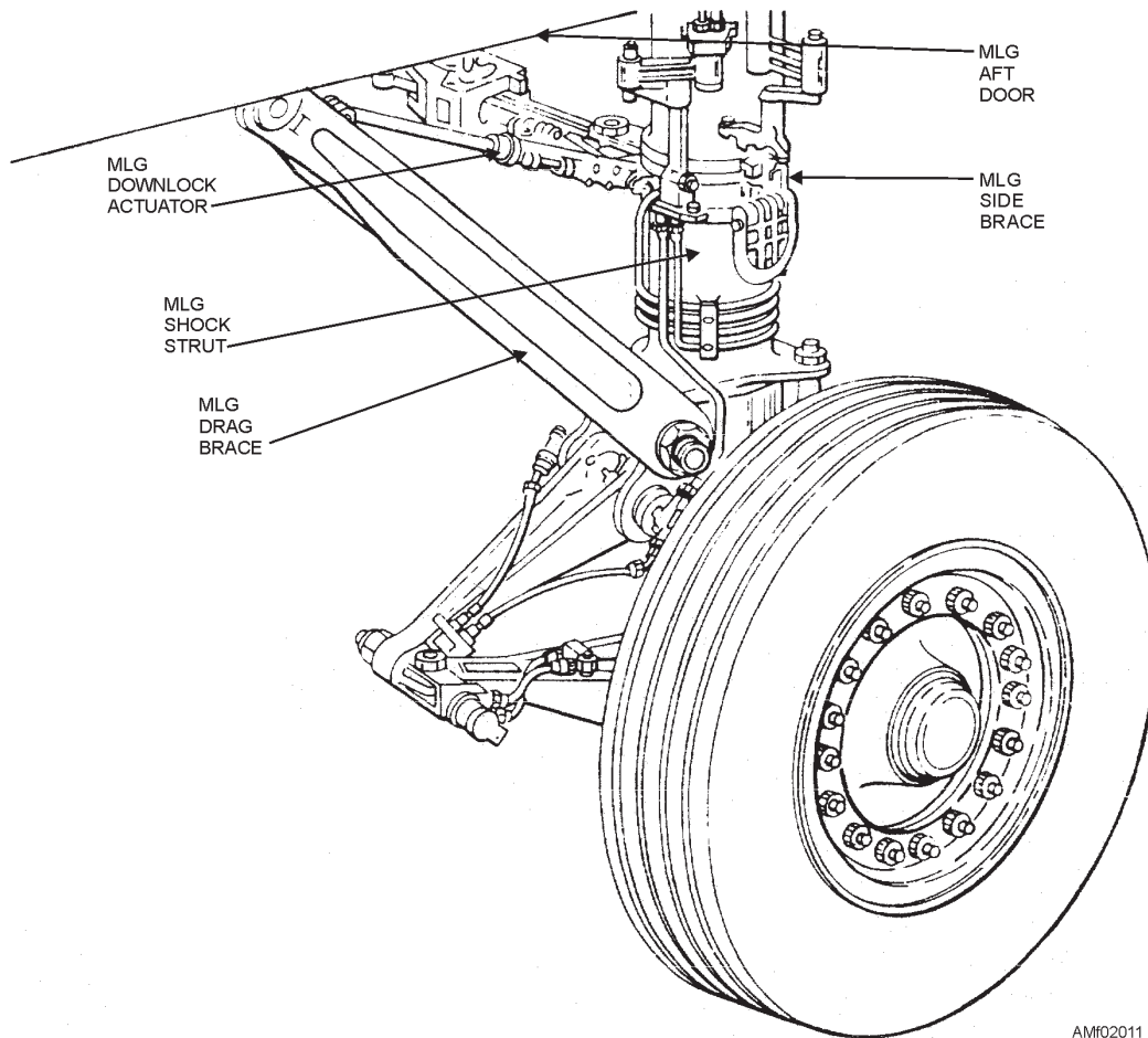
Figure 2-11.—Main landing gear.
