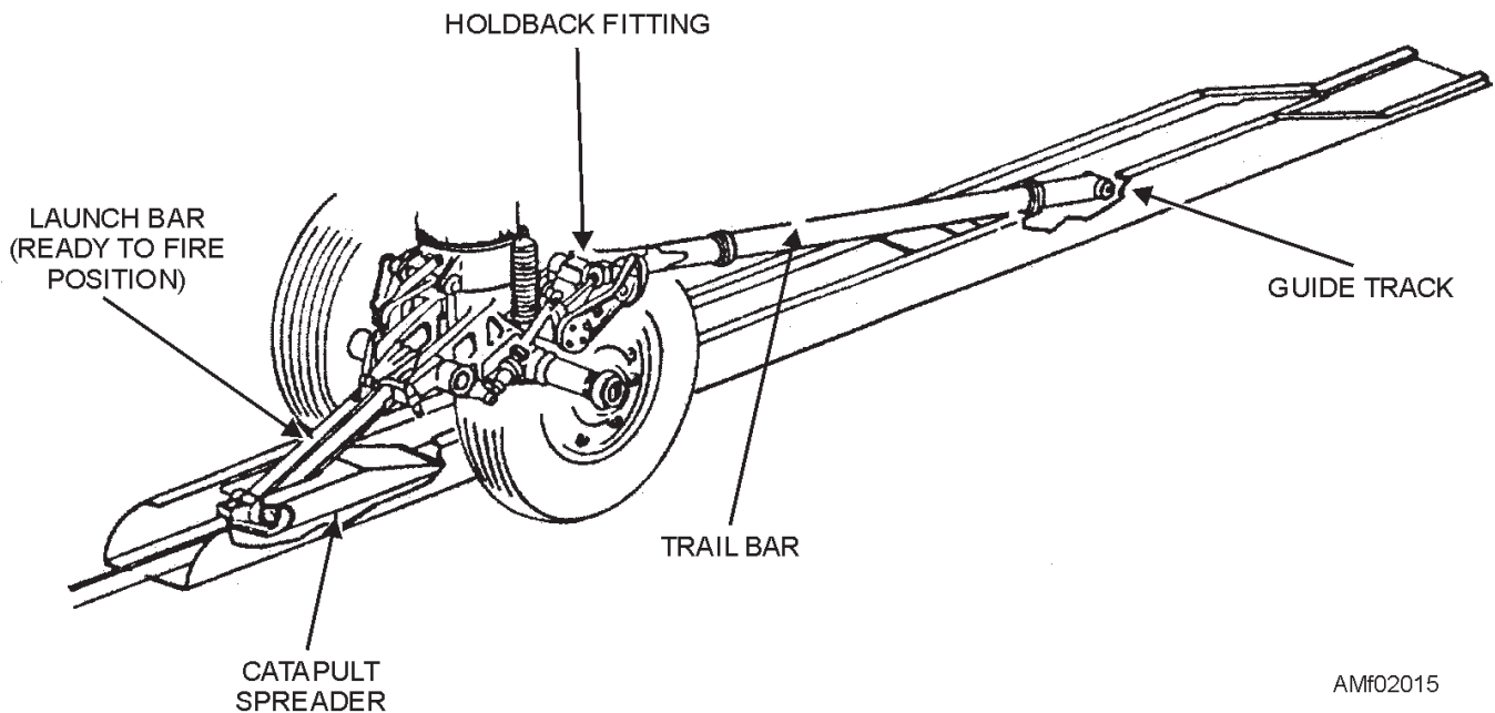
Figure 2-15.—Nose gear launch equipment.
