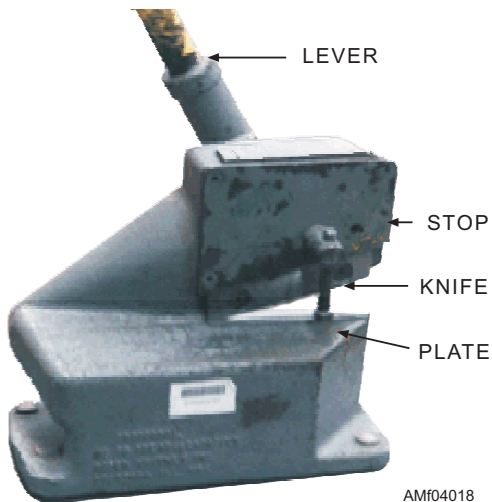
Figure 4-18.—Throatless shears.
