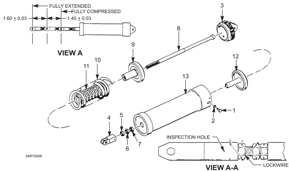
Figure 15-7.—Arresting gear assembly.
