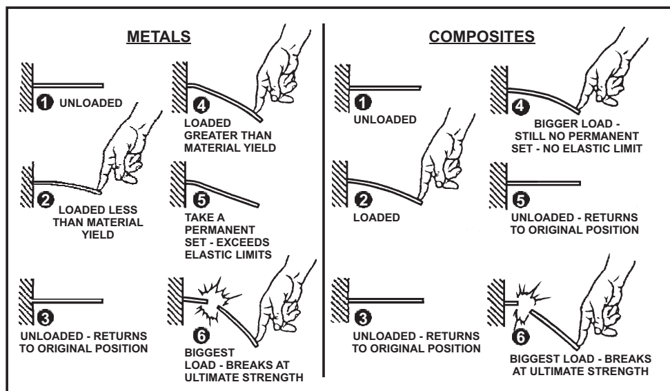
Figure 5-22.—Response to applied loads.
