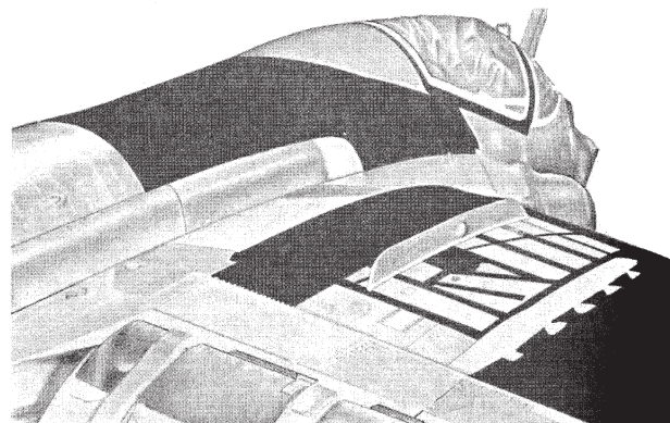
Figure 5-44.—Sealant applied to aircraft exterior surfaces.
