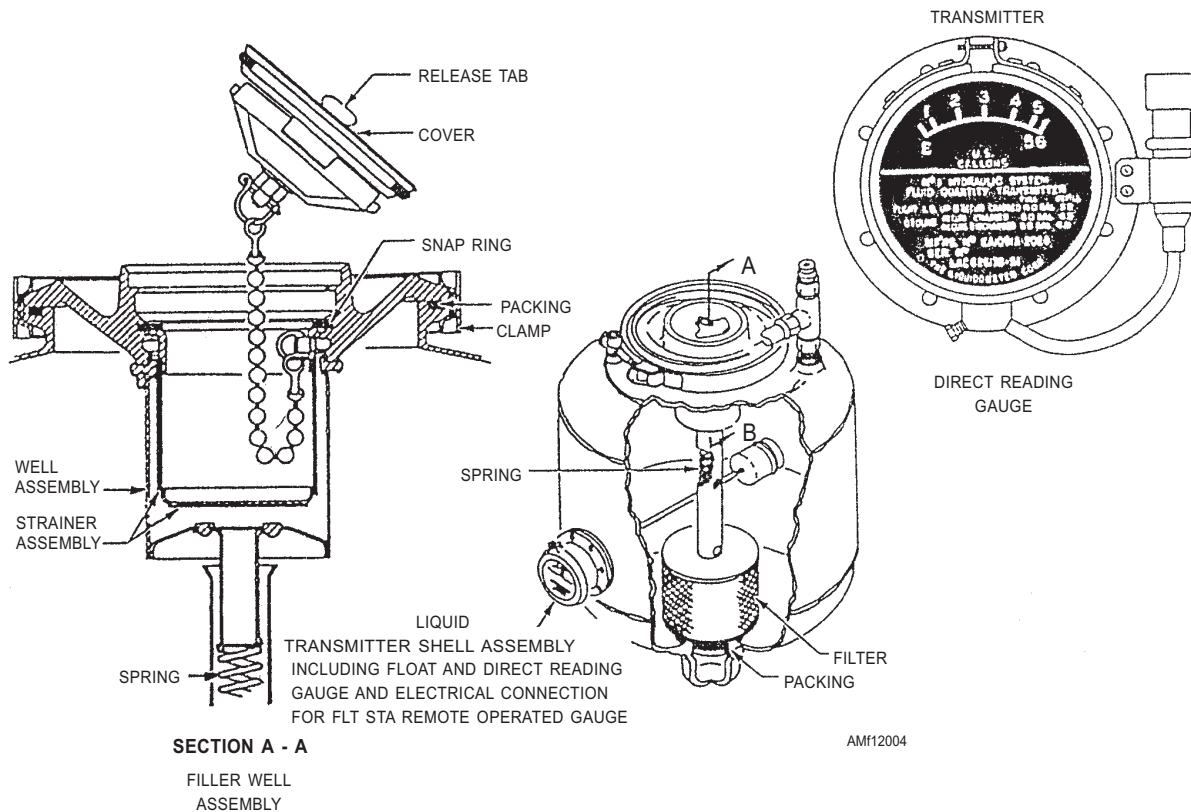
Figure 12-4.—Nonpressurized reservoir.
