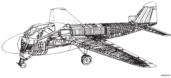
Figure 2-1.—Semimonocoque fuselage construction.
