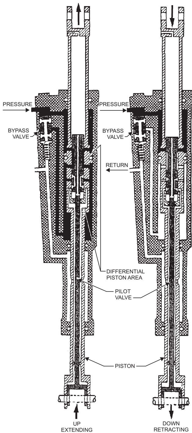
Figure 17-8.—Primary servo cylinder.
