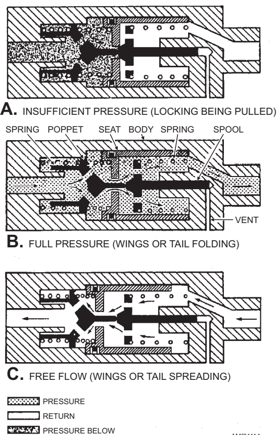
Figure 11-14.—View of priority valve.
