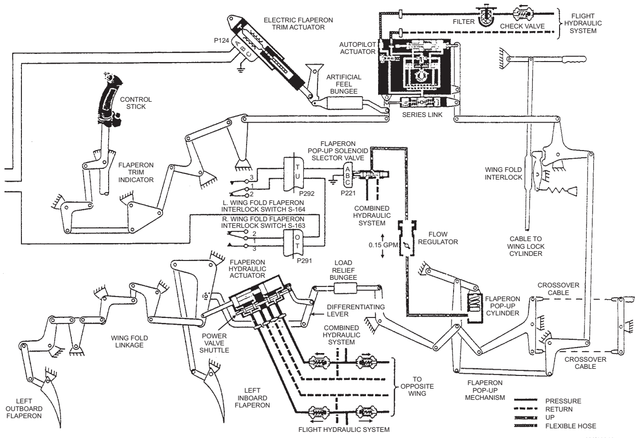
Figure 16-12.—Flaperon control system.
