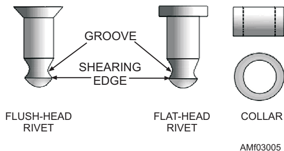
Figure 3-5.—Hi-shear rivet.
