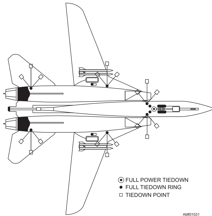
Figure 1-31.—Carrier tie-downs for aircraft jacking.
