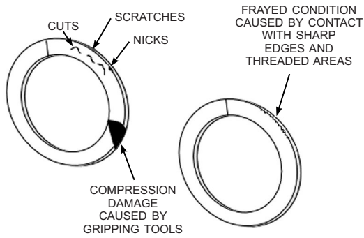
Figure 8-17.—Teflon® backup ring damages caused by improper handling.
