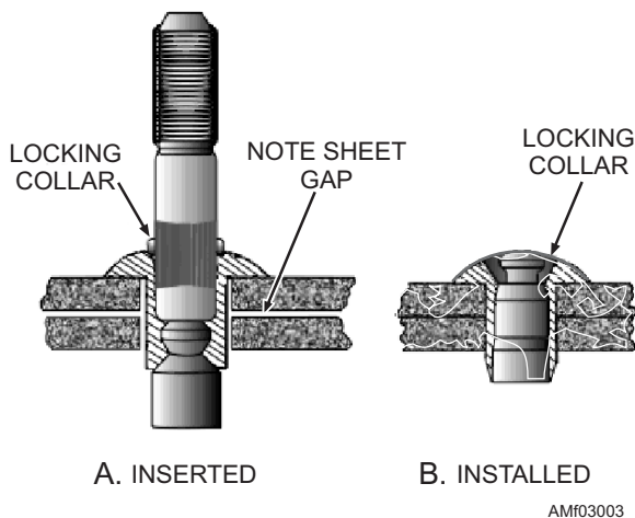
Figure 3-3.—Self-plugging rivet (mechanical lock).
