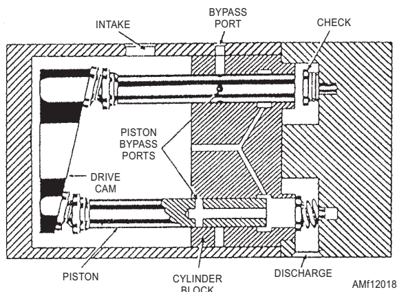
Figure 12-18.—Fluid displacement.
