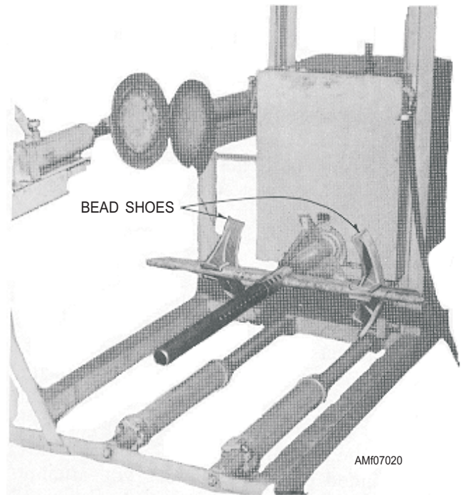
Figure 7-20.—Shaft arranged to hold tire bead while removing locking.
