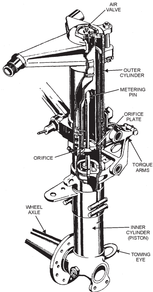
Figure 2-12.—Shock strut showing internal construction.
