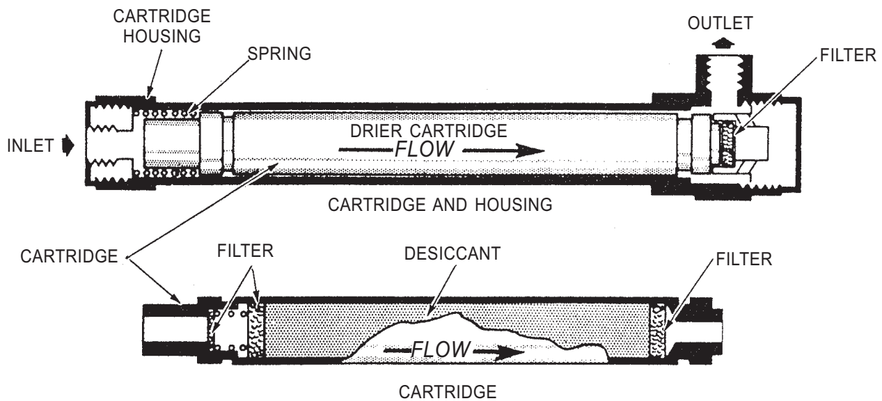
AMf12008 Figure 12-8.—Chemical air drier.
