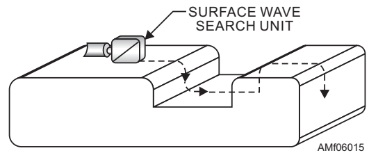
Figure 6-15.—Surface-wave inspection.
