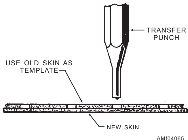
Figure 4-65.—Transferring rivet holes.
