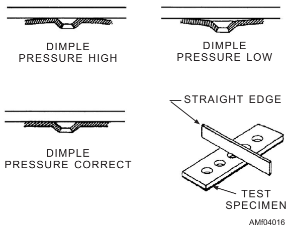
Figure 4-16.—Checking dimple equipment air pressure.
