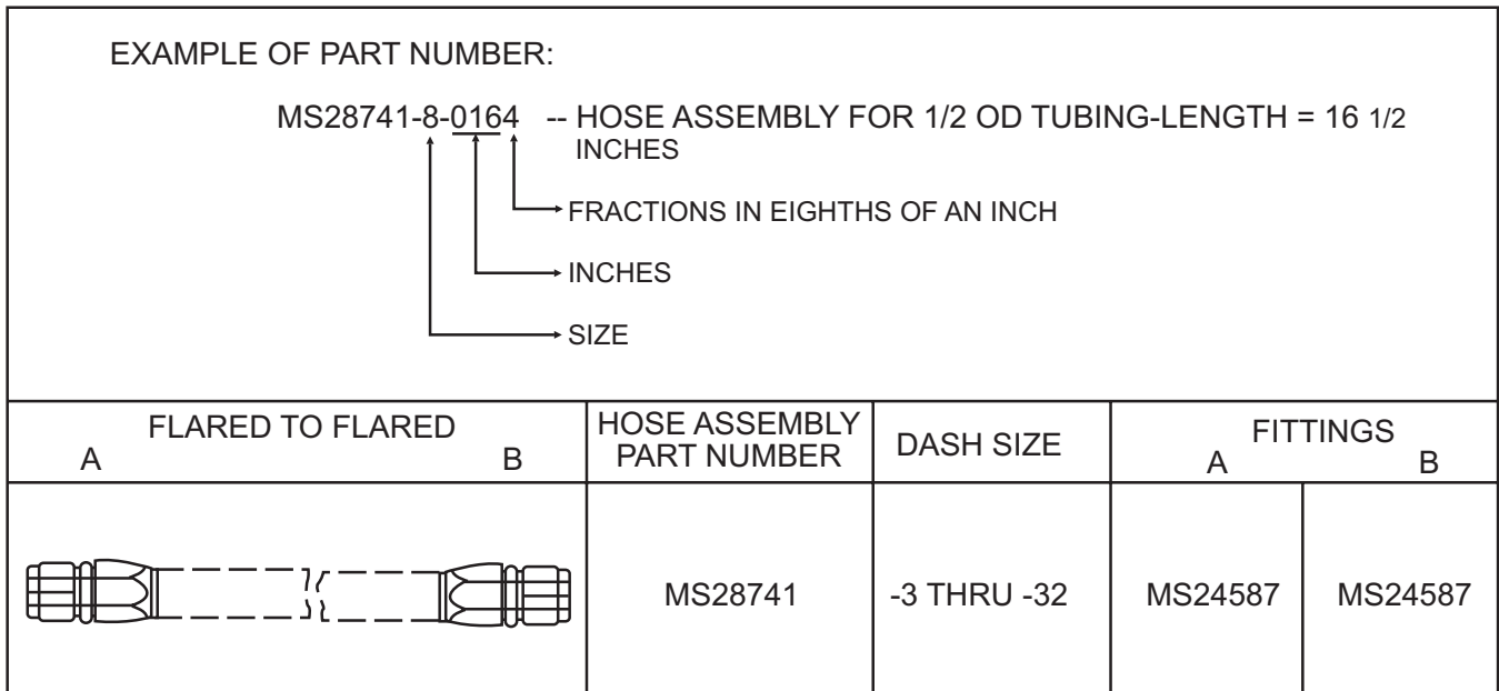
Figure 10-9.—Synthetic rubber medium-pressure hose assembly.
