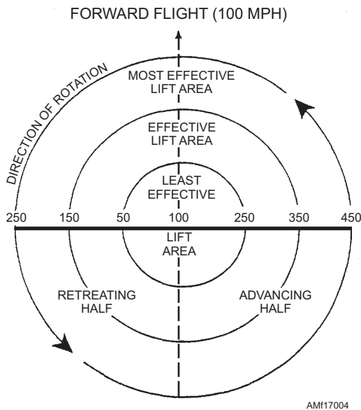
Figure 17-3.—Symmetry of lift.
