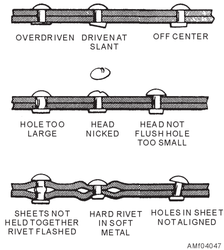
Figure 4-47.—Incorrectly driven rivets.
