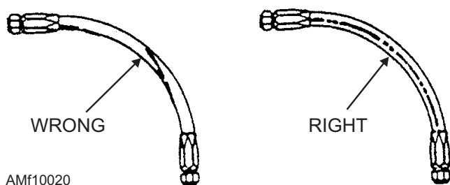
Figure 10-20.—Hose twist.
