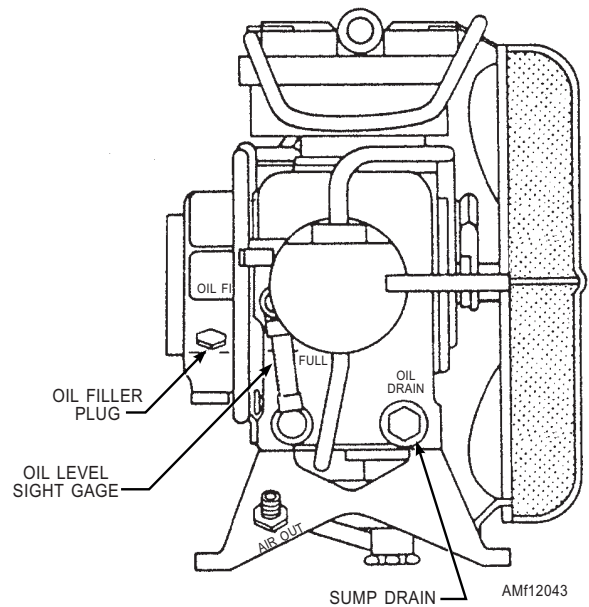
Figure 12-43.—Air compressor.
