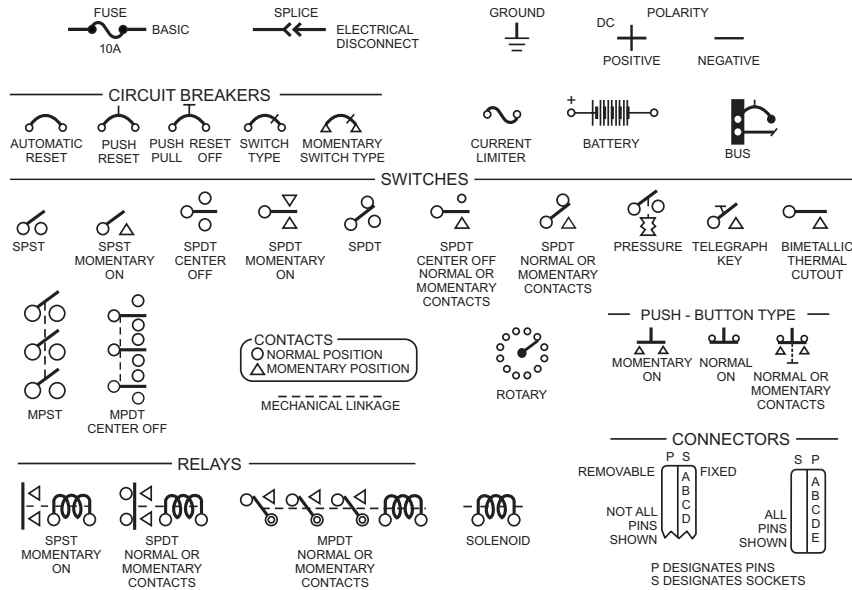
Figure 1-4.—Electrical symbols.
