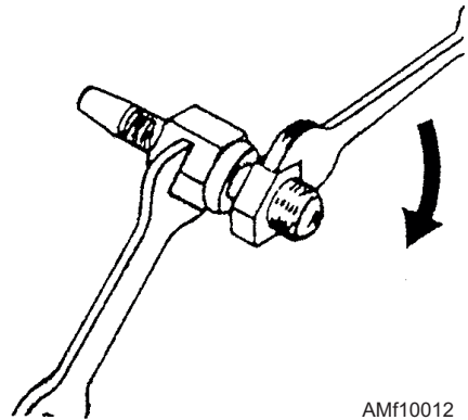
Figure 10-12.—Nipple and nut assembly.
