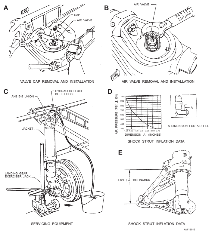
Figure 13-15.—Servicing a landing gear strut.
