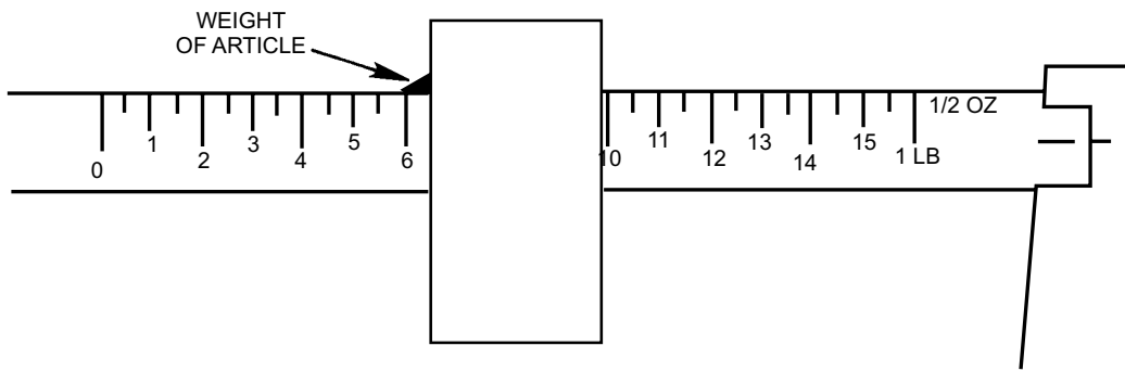
Figure 3-12.—Beam scale.
