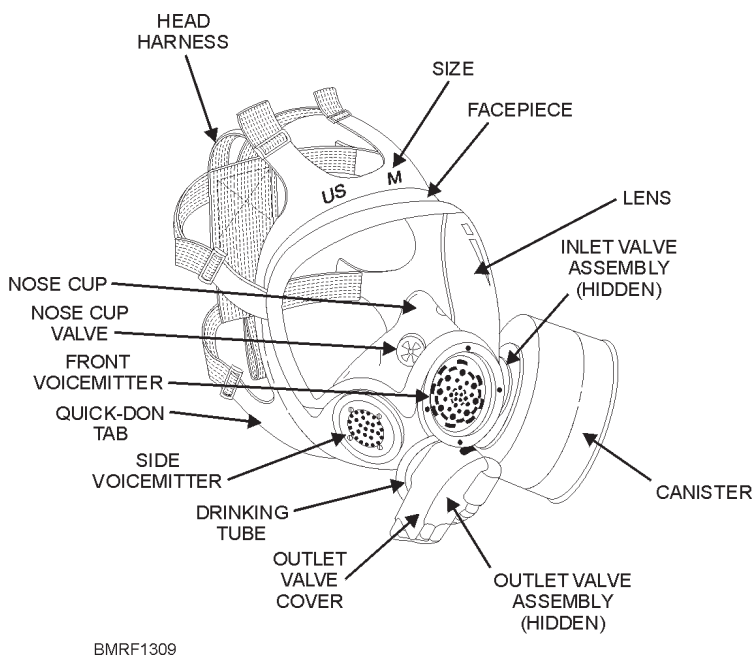
Figure 13-9.—MCU-2/P protective mask.
