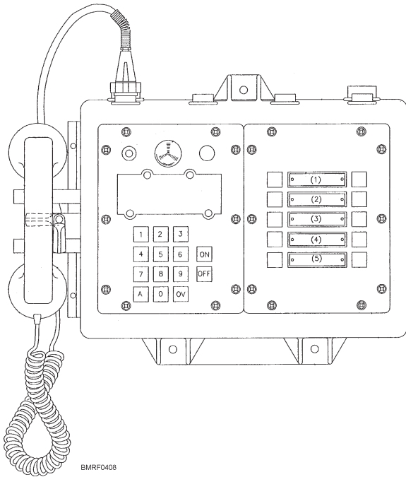
Figure 4-8.—Network terminal.
