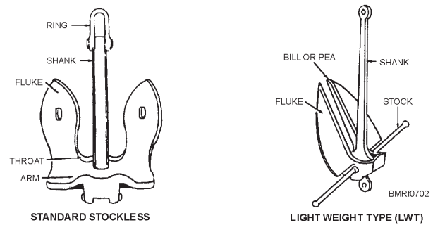
Figure 7-2.—Anchors.
