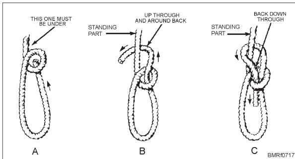
Figure 7-17.—Tying a bowline.
