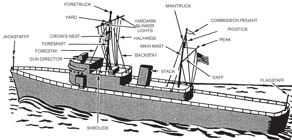
Figure 8-10.—Top hamper.
