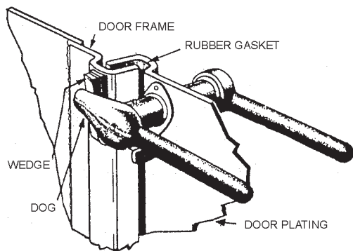
Figure 8-4.—Dogs and gasket for watertight door.
