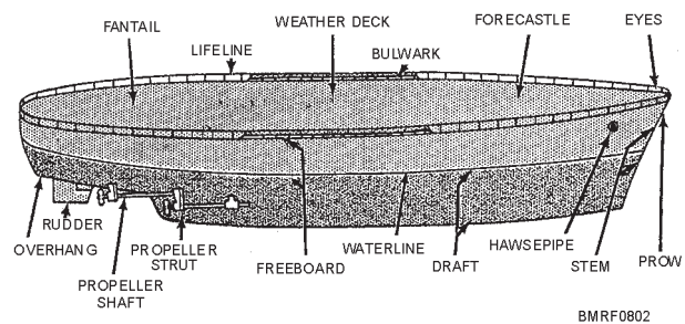
Figure 8-2.—The hull.
