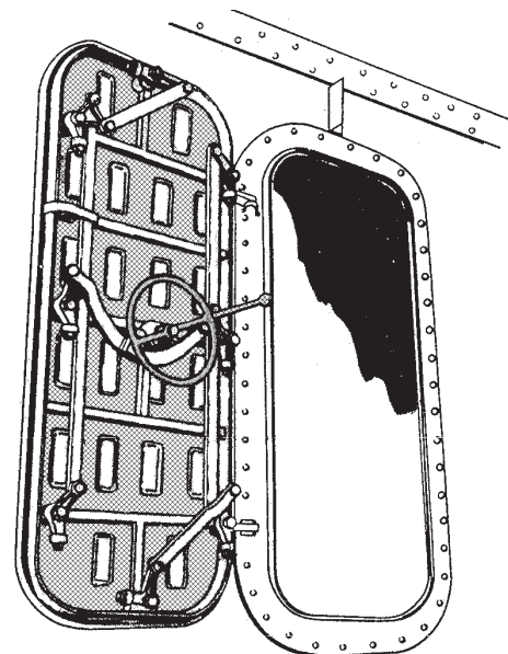
Figure 8-6.—Quick-acting watertight door.
