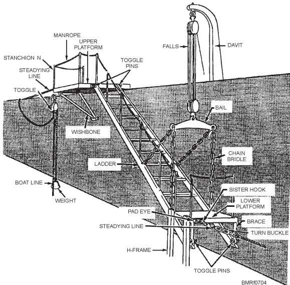
Figure 7-4.—A rigged accommodation ladder.
