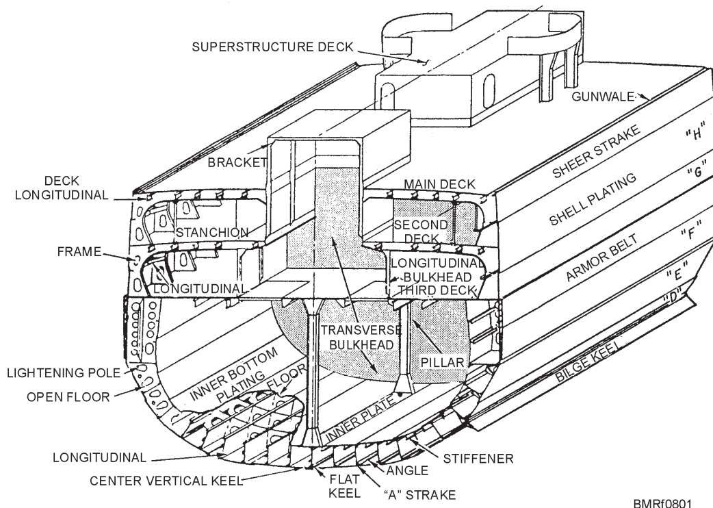
Figure 8-1.—Hull structure of a cruiser.
