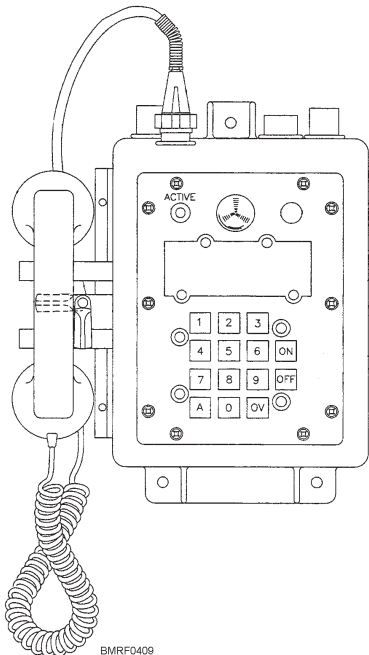
Figure 4-9.—Dial terminal.
