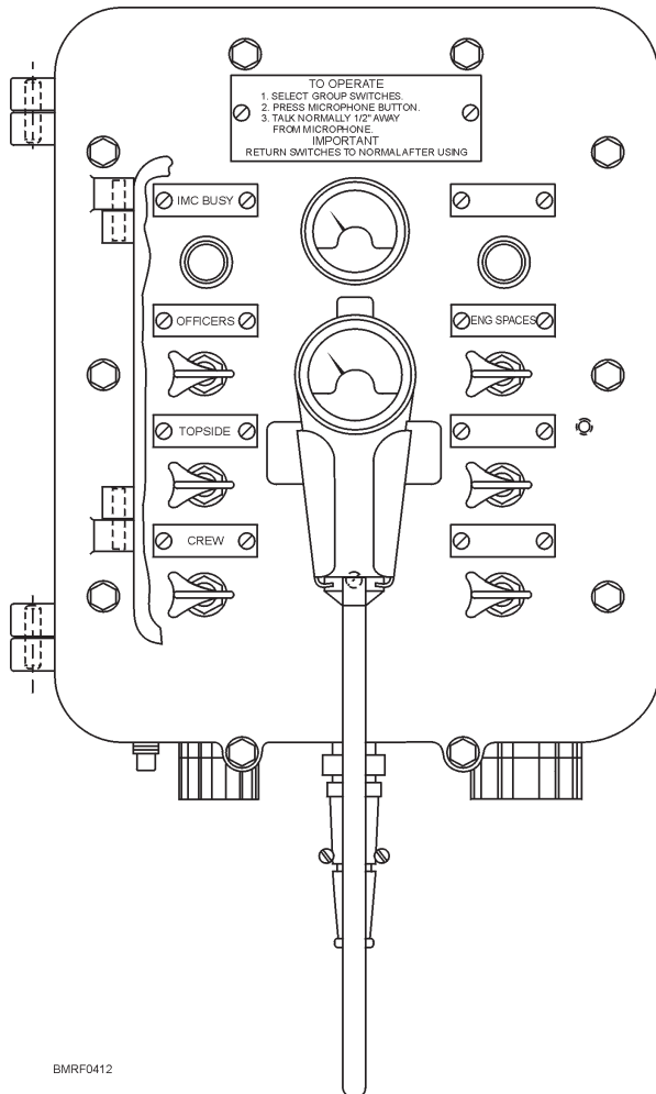
Figure 4-12.—Loudspeaker transmitter
