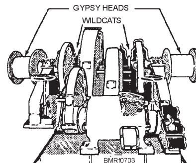
Figure 7-3.—Horizontal shaft anchor windlass.
