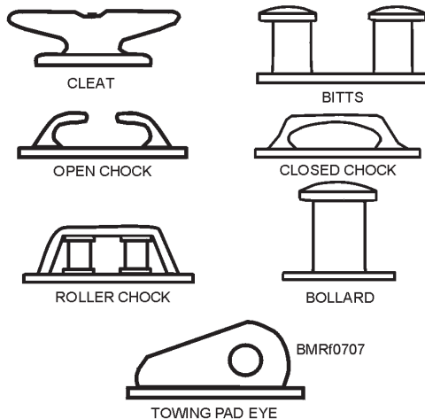
Figure 7-7.—Deck fittings.
