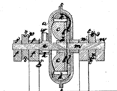
Section of Pulveriser.
