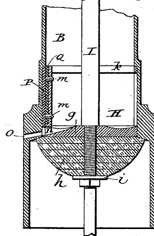
Fig. 2. on x-x
