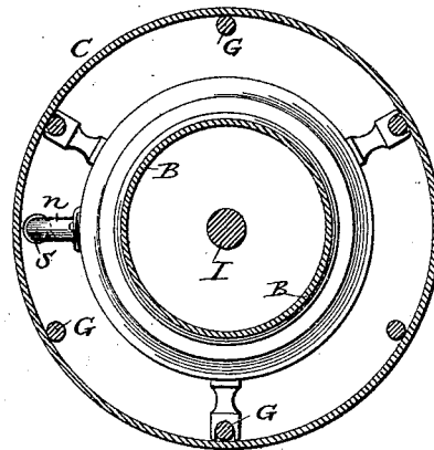
Fig. 2. on x-x
