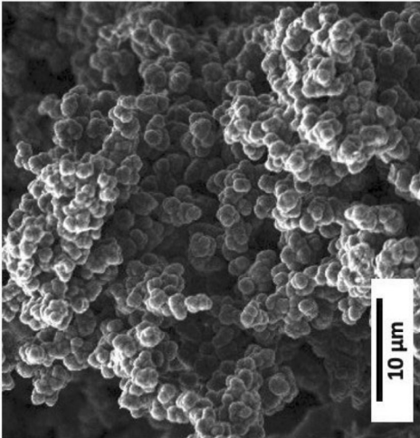
6,200x magnification
