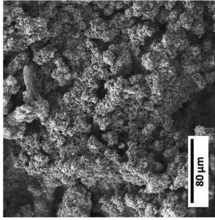
1,000x magnification
